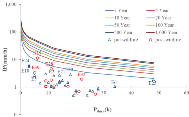
FIGURE 6 Monchique's IDF curves of varying return periods with the precipitation events selected and analyzed in this study (blue triangles are pre-wildfire events, red circles are post-wildfire events) [Colour figure can be viewed at wileyonlinelibrary.com]
