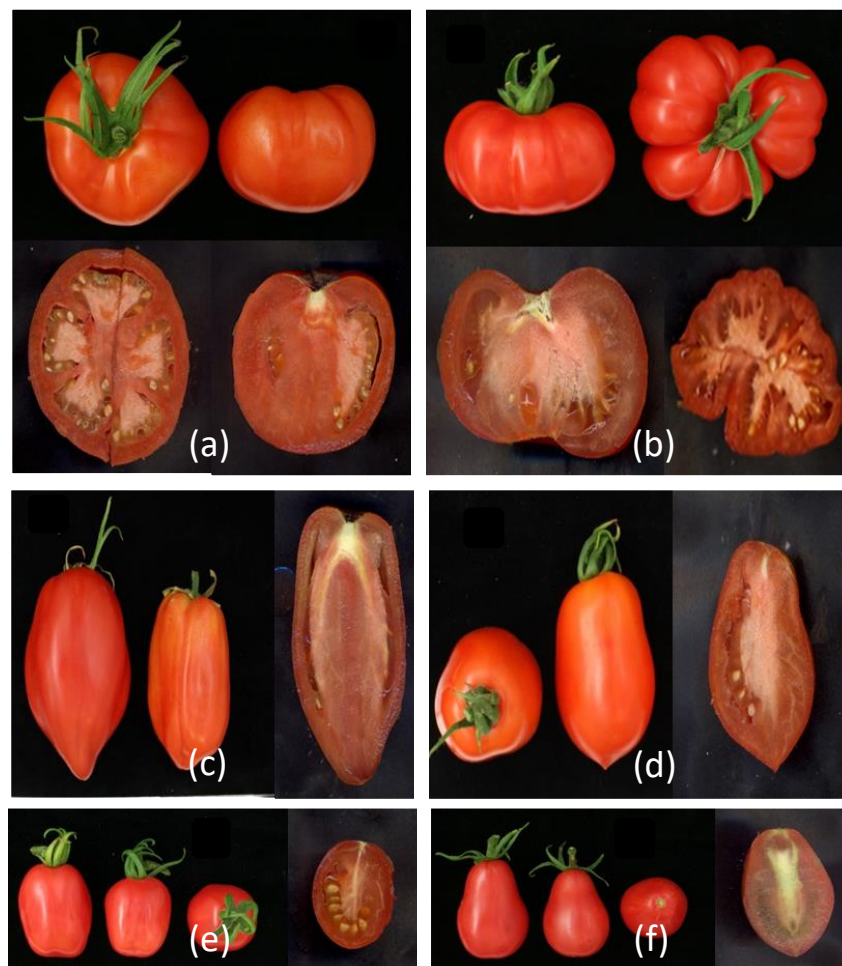
Figure 10. Examples of accessions with fruit shape mutations in our collection. (a) RF_096 with the lc mutation; (b) RF_041 with the fas mutation; (c) RF_024 with the sun mutation; (d) RF_214 with the ovate mutation; (e) RF_035 with the ovate mutation; and, (f) RF_043 with the sun and ovate mutations.
