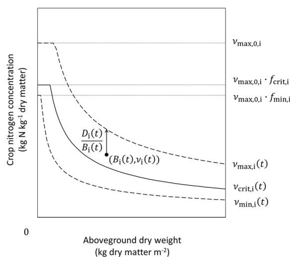
Fig. 1 Schematic representation of nitrogen dilution curves (Greenwood et al. 1990; Justes et al. 1994; Stöckle and Debaeke 1997) of the maximum ( \nu_{\max,i}(t) ), critical ( \nu_{\text{crit},i}(t) ) and minimum nitrogen concentrations ( \nu_{\min,i}(t) ) with aboveground dry crop biomass. At very low biomasses, the maximum, critical and minimum nitrogen concentrations are equal to \nu_{\max,0,i} , \nu_{\max,0,i} \cdot f_{\text{crit},i} and \nu_{\max,0,i} \cdot f_{\min,i} respectively. At higher biomasses, the curves are described by a power law. The nitrogen demand D_i(t) for a given biomass B_i(t) is calculated as the difference between the amount of nitrogen that would result to the maximum nitrogen concentration for that biomass, \nu_{\max,i}(t) \cdot B_i(t)
