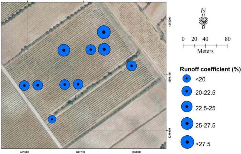
Figure 4. Spatial distribution of runoff coefficient.
