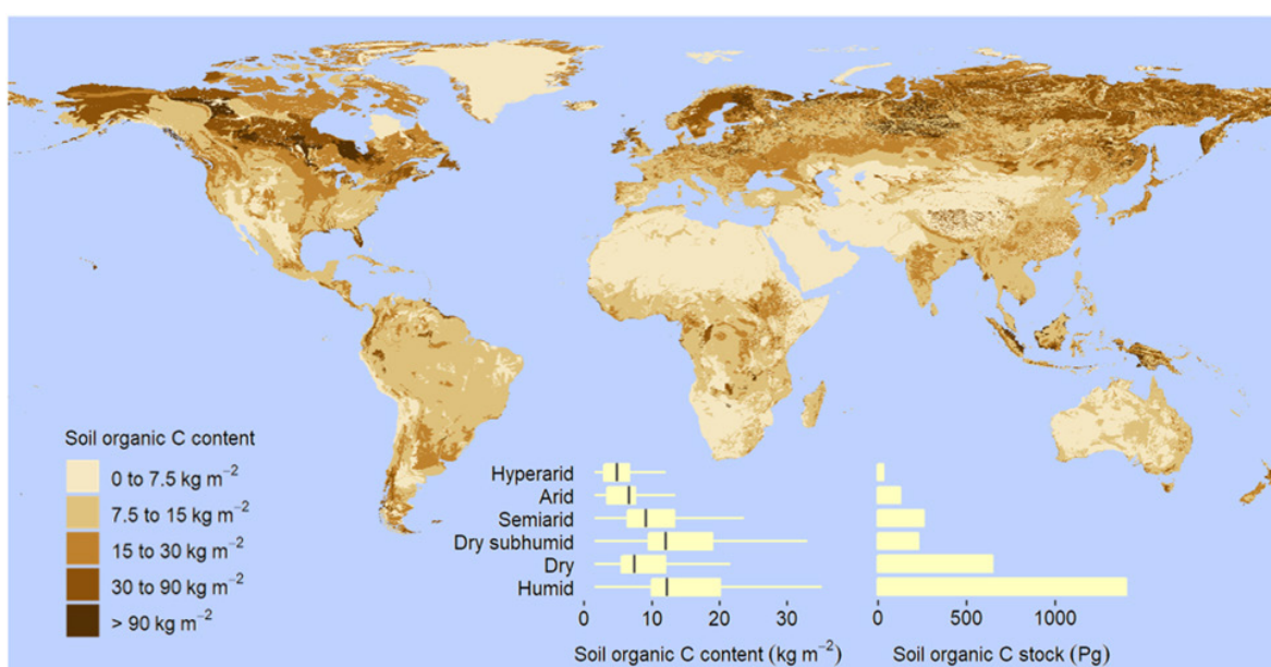
Figure 8 Distribution of soil organic carbon to one metre depth (USDA Natural Resources Conservation Service, 2006).
