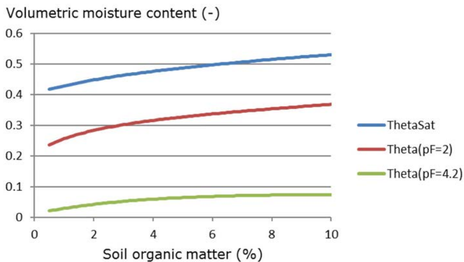
Figure 5 Curve of the volumetric moisture content at saturation, at pF 2 (field capacity) and at 4.2 (wilting point) with organic matter content.
