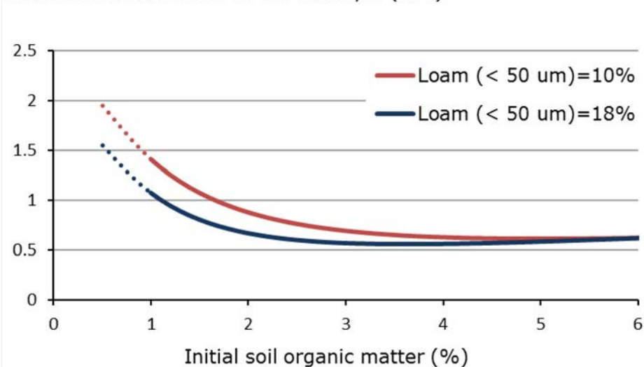
Figure 6 Increase of water availability (mm) in a layer of 10 cm with an increase of organic matter of 1%.
