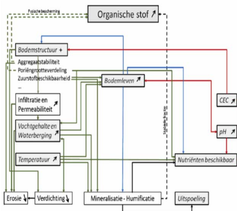
Figure 3 Schematic representation of soil interactions related to organic matter; blue lines: effect of soil life; green arrows: soil physical effects; red lines: soil chemical effects; dark lines: effects of soil processes. Dash lines: correlation with organic matter. Source: Reubens et al., 2010.
