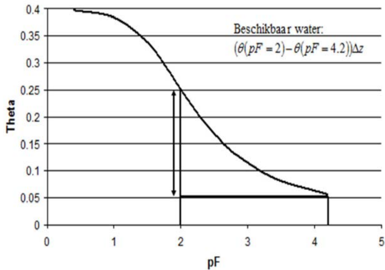
Figure 4 Water retention characteristic indicating the relationship between the pressure head (pF value) and the corresponding volumetric moisture content (Theta).
