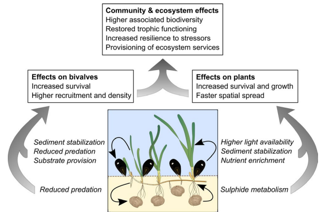
FIGURE 7 Conceptual model of prevailing mechanisms (in italics ) by which plant-bivalve co-restoration can facilitate bivalves (left) and plants (right), and the resulting community- and ecosystem-level effects (top). Images represent organism types (plant, epifaunal bivalve and infaunal bivalve), not species. Epifaunal bivalves and plants can also positively affect each other when spatially separated. Images courtesy of Integration and Application Network, University of Maryland Center for Environmental Science ( ian.umces.edu/imagelibrary/ )
