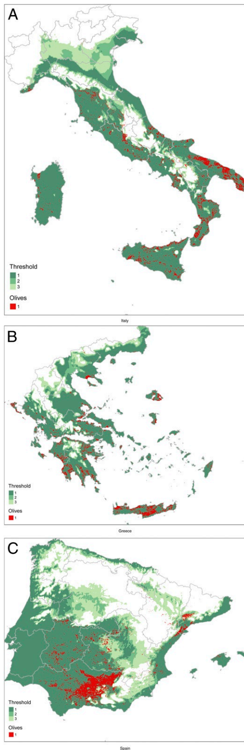
Fig. 1. Binary suitability maps and olive-production sites in Italy (A), Greece (B), and Spain (C).
