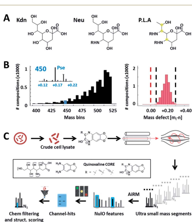
Fig. 1 Universal sialic acid large-scale survey approach. (A) outlines the three main NulO core structures known to date: Kdn (deamino-neuraminic acid), Neu (neuraminic acid) and P.L.A. = Pse (pseudaminic acid), Leg (legionaminic acid) and Aci (acinetaminic acid). (B) demonstrates the potential diversity generated through (combinations of) (natural) diversifications of the three main NulO core compositions Kdn, Neu and P.L.A. (Pse/Leg/Aci). The left graph shows a binned mass histogram (5 Da) of the theoretically possible chemical compositions between 380–520 Da. Already more than 25 different compositions are found within \pm 0.05 Da of Pse5Ac7Ac. The image on the right shows the mass defect binned for every calculated structure, which all fall within a very narrow window between 0.05–0.25 Da. The mass spectrometric mass defect is defined as the delta of monoisotopic mass and nominal mass. For combinatorial space and abbreviations see ESI-Table, sheet 8.† This filters for possible realistic structures during parent NulO annotation. (C) outlines the established large-scale survey pipeline starting from crude cell lysates, \alpha -keto acid specific chemical labelling, small mass channel scanning (2.75 m/z windows, from 380–520 Da), and the automated structural filtering and evidence scoring pipeline to annotate parent NulOs. In summary, channel hits and compositions are discovered based on highly conserved quinoxaline-core fragments together with the diversification-independent carbon chain length and structural features.
