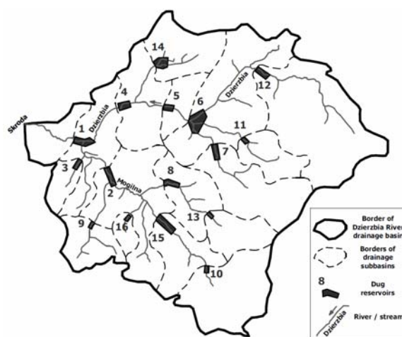
Fig. 3. Localization of planned reservoirs in the catchment; source: own elaboration
