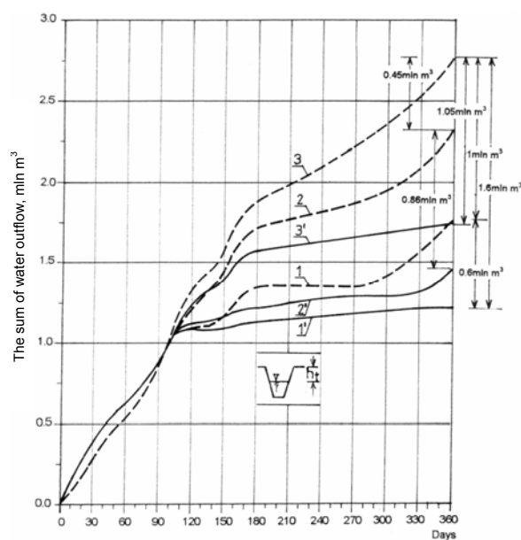
Fig. 12. Total outflow from the catchment with existing drainage system and also with ditches system filled up for different retention; 1 – existing system ht = 0.2 \text{ m} , 2 – existing system ht = 0.8 \text{ m} , 3 – existing system ht = 1.2 \text{ m} , 1' – ditches system filled up ht = 0.2 \text{ m} , 2' – ditches system filled up ht = 0.8 \text{ m} , 3' – ditches system filled up ht = 1.4 \text{ m} ; source: own study
