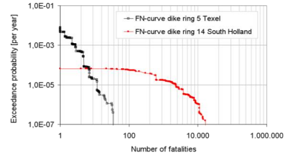
FN-curve
