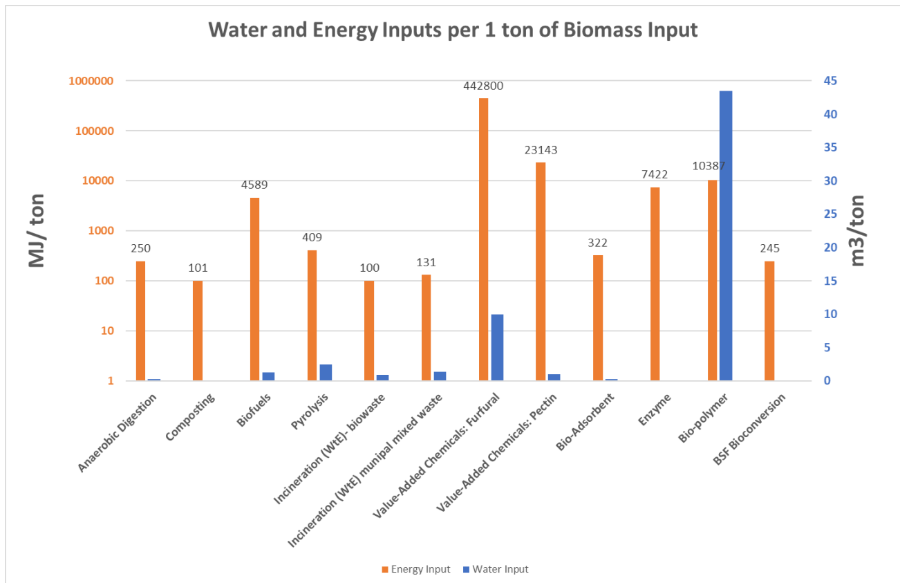
Figure 5.1: The energy and water required to treat 1 ton of biomass for 12 different technologies
