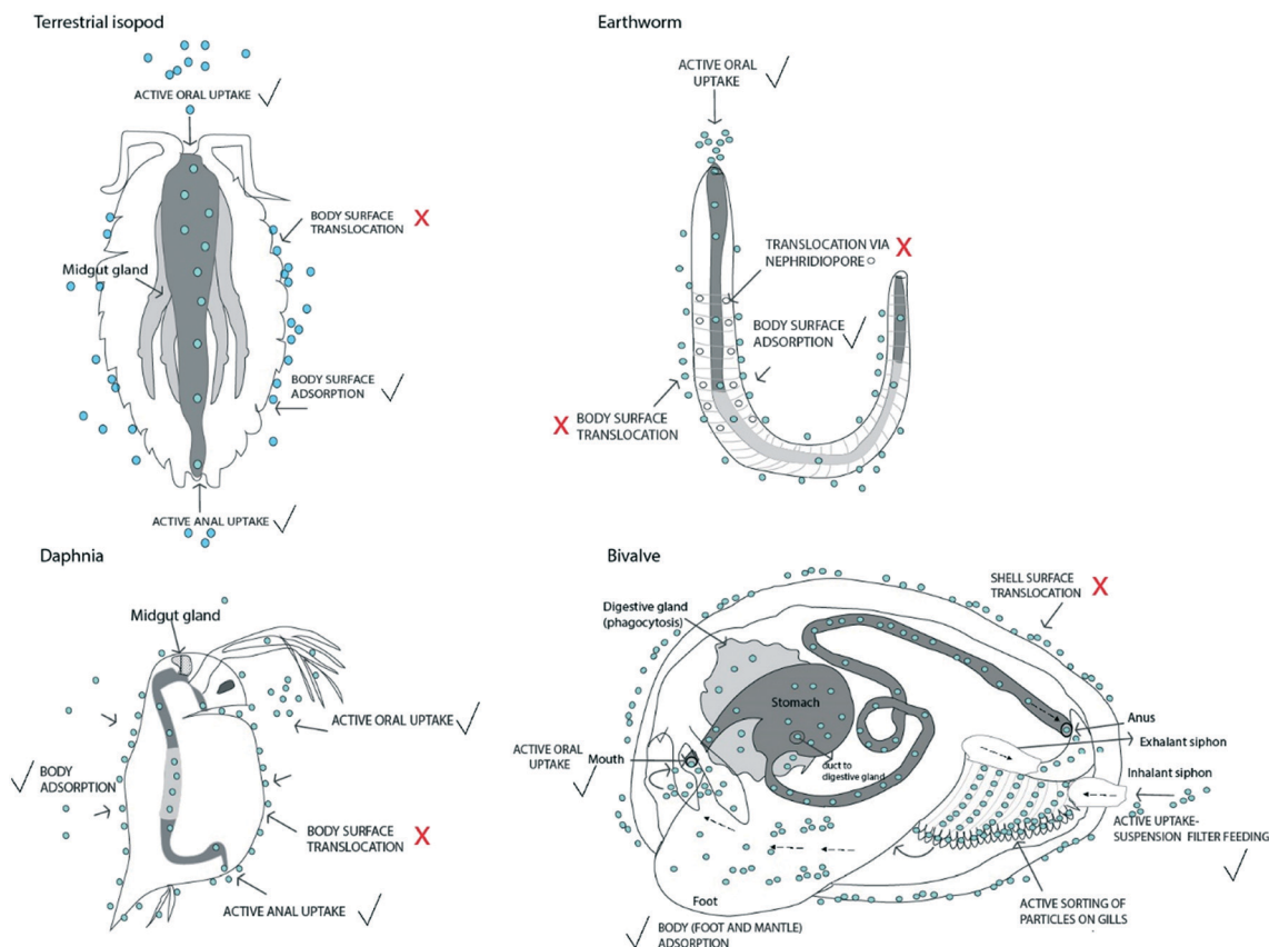
Fig. 1 Active and passive uptake of nanomaterials in different representative invertebrate species commonly used in environmental research: terrestrial isopod (Crustacea), earthworm (Annelida), water flea (Crustacea), and bivalve (Mollusca; e.g. Mytilus sp.; only one valve with a removed mantle is shown). The organisms are presented schematically, as extracted from Brusca et al. (2016) 30 and Ruppert et al. (2004). 25 The gut is shown as a grey tube. Light grey represents the midgut, while the foregut and hindgut regions are dark grey. The position and length of each gut region are not shown at realistic scales. Nanomaterials are shown as blue circles. Routes where NM passage is questionable are marked with a question mark and a red cross. Probable uptake routes are marked with a black tick symbol.
