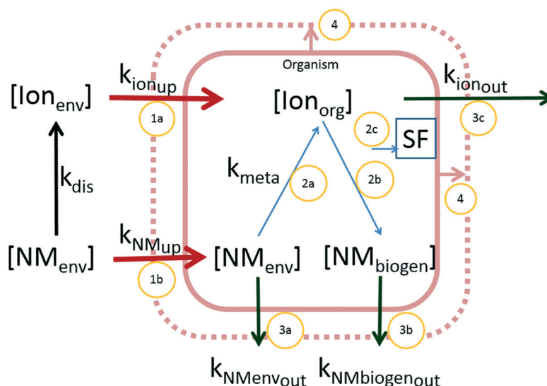
Fig. 2 Conceptual overview of different forms of metal-based NMs and kinetic pathways of uptake and elimination. Forms of materials: NM env : nanomaterial in the original form (can be both in the environment and in the organism), Ion env : ionic form of the NM-material in the environmental compartment (dissolved), Ion org : ionic form in the organism (may originate from both Ion env as well as dissolved from NM env in the organism), NM biogen : biogenic particulate form, F i : inert fraction; kinetic processes displayed by arrows. Red arrows: uptake. 1 a : ionic uptake, 1 b : particulate uptake; blue arrows: within organism kinetics. 2 a : dissolution of NMs, 2 b : biogenic formation of particulate materials, 2 c : transport to the inert fraction; dark green arrows: elimination: 3 a elimination of original NM, 3 b : elimination of the biogenic particulate material, 3 c : elimination of the ionic form. Pink arrows: growth dilution (4).
