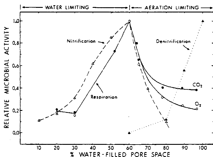
Figure 4.2. Relationship between water-filled pore space and relative amount of microbial nitrification, denitrification, and respiration ( \text{O}_2 -uptake) and \text{CO}_2 -production (Source: Linn and Doran, 1984 p. 1271)
