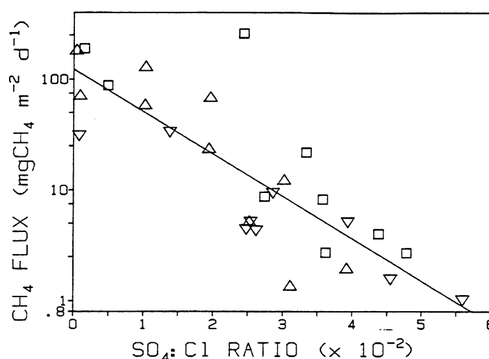
Figure 3.4. Average \text{SO}_4^{2-} /Cl - ratios in the top 15 cm of marsh soils and methane emissions across the air-soil interface ( r = -0.824 , P < 0.1 ; After Bartlett et al. , 1987)
