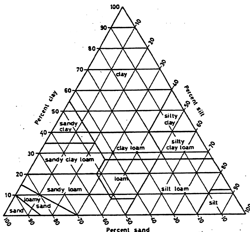
Figure 2.3. Soil textural classes determined by percentages of sand, silt and clay present (Source: Hodgson, 1978)
