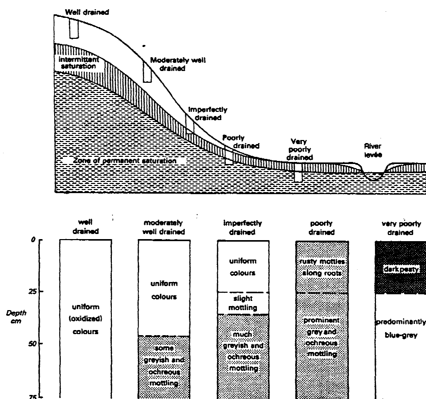
Figure 2.5. A hydrological sequence of soils in a permeable parent material (From Avery, 1987)
