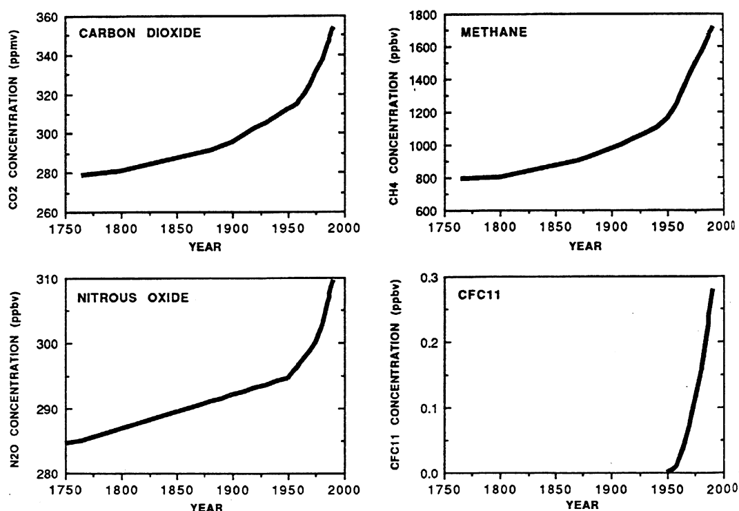
Figure 1.1. Increases in atmospheric concentrations of CO 2 , CH 4 , N 2 O and CFCs since the year 1750 (Source: IPCC, 1990 p. 16).
