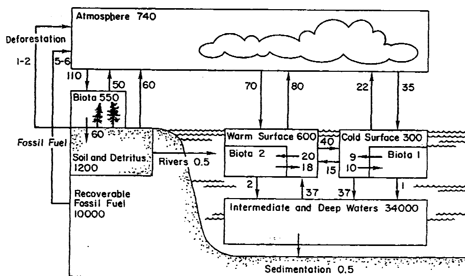
Figure 5.1. Estimates of main sources and sinks of the global carbon cycle (in Pg CO 2 -C yr -1 ; source: Moore III et al. , 1989)
