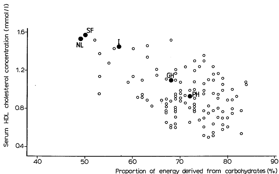
Figure 1. The relationship between the concentration of HDL cholesterol in serum and the proportion of energy (percent) from carbohydrate in young boys. ●, Mean values for Ghana (GH), The Philippines (PH), Italy (I), The Netherlands (NL) and Finland (SF). The Pearson correlation coefficient ( r ) was -0.98 . ○, Individual data for the Philippino boys ( r = -0.40 ). Data taken from Knuiman et al. (1983), and supplemented with unpublished figures of Knuiman and West.
