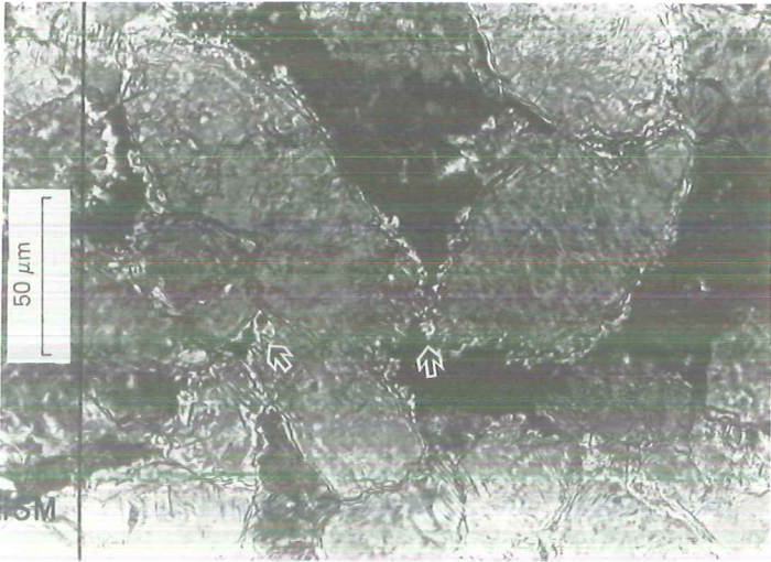
Fig. 11. Dissolution phenomena in the coarse crystic fabric of the calcite that makes up an important part of the petrocalcic horizon of Profile Arroyo 1 at a depth of approximately 10 cm below the top of this horizon. The arrows indicate frayed edges of the calcite crystals along the voids. Photograph taken with crossed polarisers. (Pseudospar in the terminology of Bathurst, 1971.) (Photo courtesy of ISM.)
