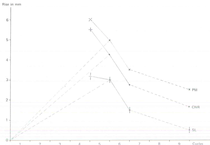
Fig. 28. The vertical movements of the objects of Experiments IIIb1 and IIIb2 plotted against time. A considerable rise for all objects is evident during the first five cycles of Experiment IIIb1. The position of the objects in moist condition shortly after the initiation of the fifth cycle is indicated by hollow symbols. At the initiation of the sixth cycle, the set-up was changed and Experiment IIIb2 started. A heavy weight was placed on the surface of the lime which caused subsidence of all objects during the sixth cycle. From the position of the objects at the end of the ninth cycle it is evident that the subsidence must have continued at a diminished rate for some time after the sixth cycle. The following objects are shown: PM = petrocalcic fragment, middle; CNR = clay nodule, right; SL = raña gravel, left.
