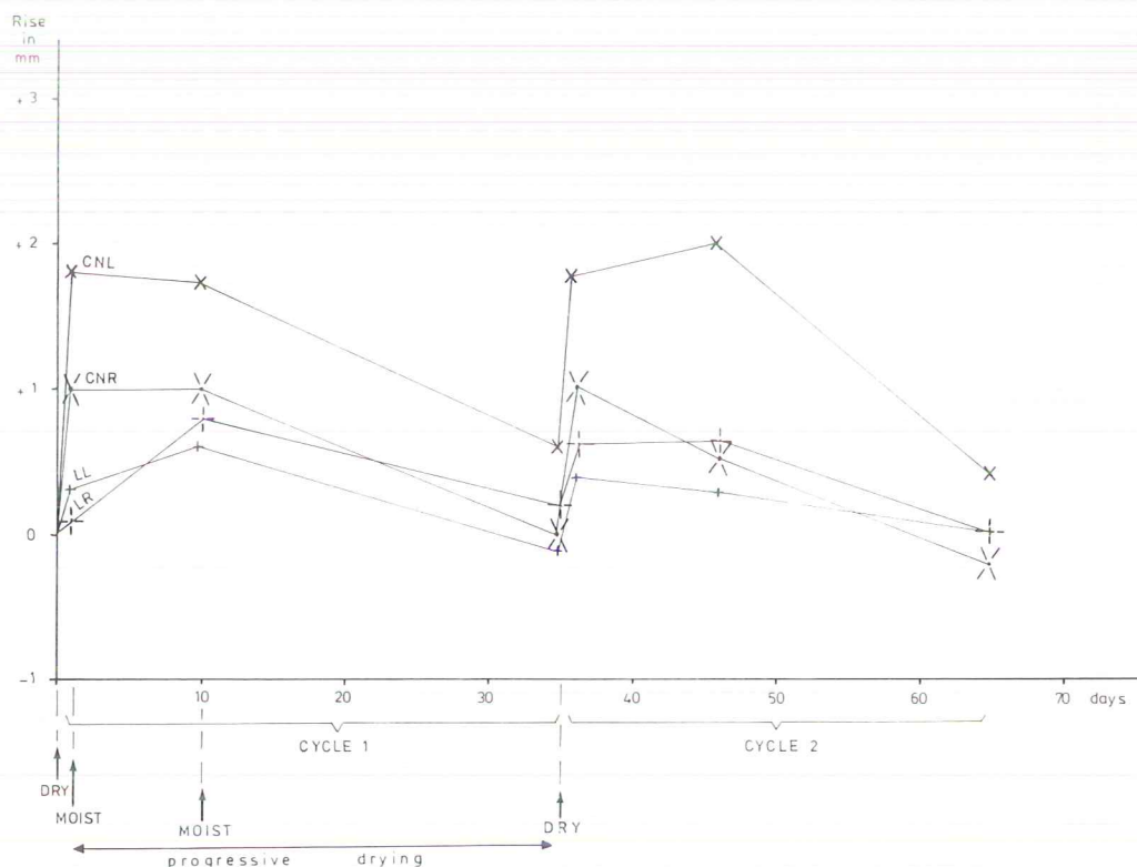
Fig. 21b. The vertical movements of Clay nodules (CNR) and (CNL) and Lead pellets (LL) and (LR) of Experiment Ia, plotted against time, during the first two cycles of the experiment.
