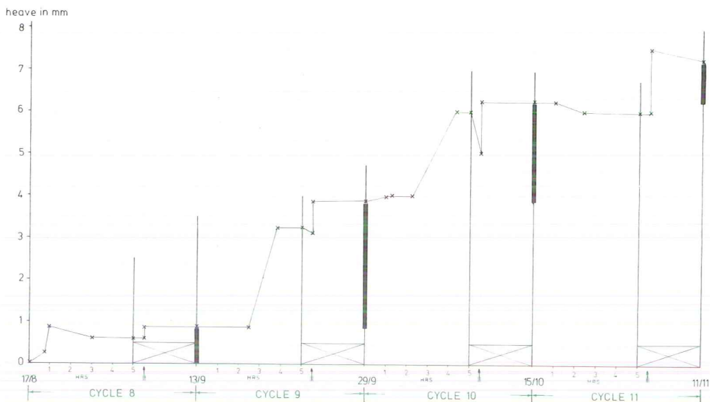
Fig. 25. The heave of the surface of the lime of Experiment II, during the last four cycles of the experiment. Each cycle has been subdivided into two parts with different scales: The first part is divided into hours, the second part (crossed) represents the remainder of the cycle (see dates). Arrows indicate the moment at which the sample was introduced into a stove for drying, which led to some heave immediately, due to expansion of the entrapped air. The solid bars indicate the net heave per cycle. It is clear that most of the heave occurs shortly after the moistening. Downward movements of the surface of the lime occur in each cycle.
