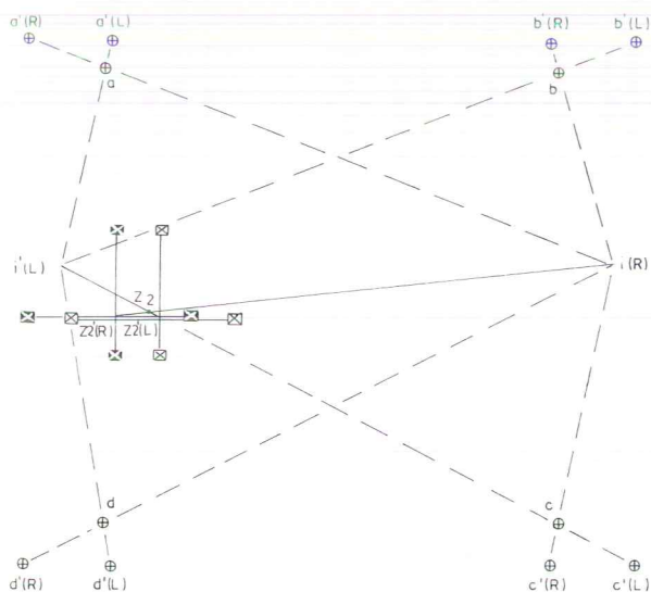
Fig. 20b. Construction of the projected position of Clay nodule CNL (Z2) of Stereo-pair 577 LR, of Experiment II, in dry condition at the end of the 11th cycle (see Fig. 19). The explanation of the radial triangulation procedure is in the text. Solid squares represent the shadows of the markers of the clay nodule in the right hand photo and open squares those in the left hand photo.
