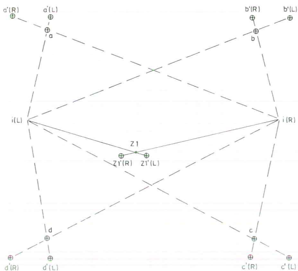
Fig. 20a. Construction of the projected position of Lead pellet LL (Z1) of Stereo-pair 577 LR, of Experiment II, in dry condition at the end of the 11th cycle (see Fig. 19). The explanation of the radial triangulation procedure is in the text.
