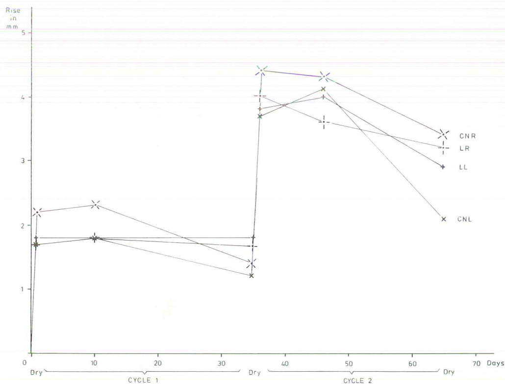
Fig. 23. The vertical movements of the objects of Experiment II plotted against time, during the first two cycles. The conditions represented in chronological order are: dry-moist-moist-dry-moist-moist-dry. CNL = clay nodule left, CNR = clay nodule right, LL = lead pellet left, LR = lead pellet right.
