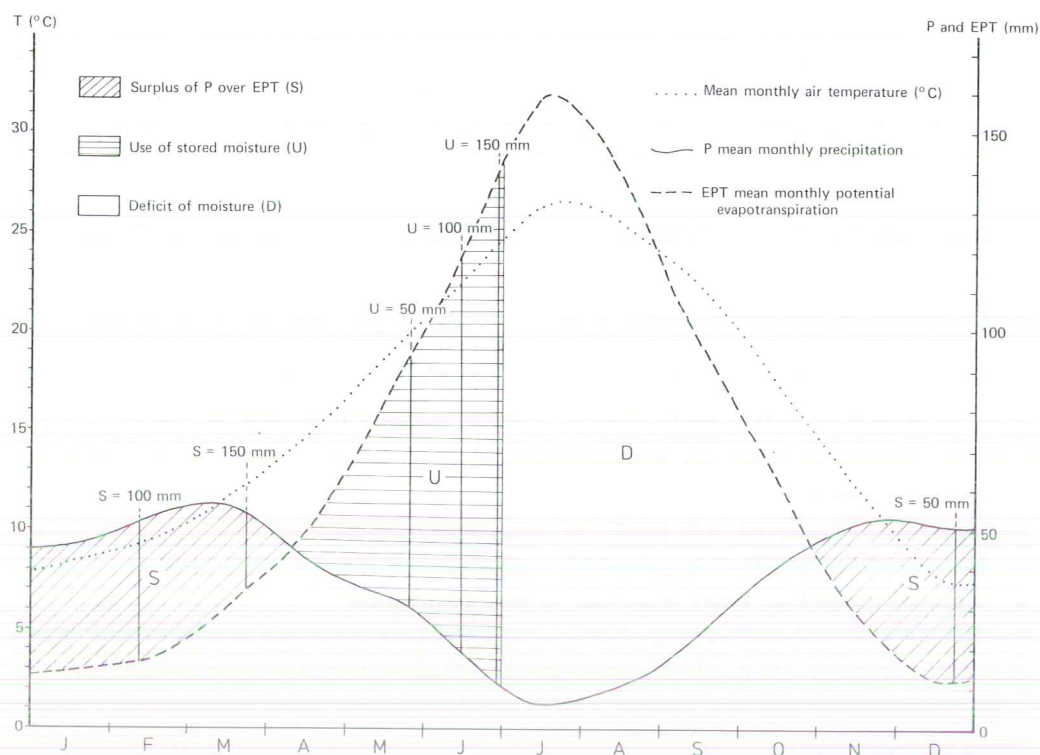
Fig. 2. Water balance diagram based on the average precipitation and evapotranspiration for the stations Lobon and Almendralejo, for the period 1957-1966. The average of the mean monthly air temperatures for these two stations has been indicated too. The potential evapotranspiration has been computed according to Thornthwaite (1948). In the graph it has been indicated, how much moisture surplus (S) results from the winter rains and during which period this moisture, if stored in the soil, can compensate for the excess of evapotranspiration over precipitation in the summer period. The total surplus of about 150 mm is used up (U) by the beginning of July.
