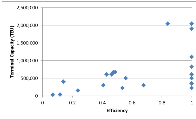
Figure 8. The Efficiency Of Different Terminals With Different Size
