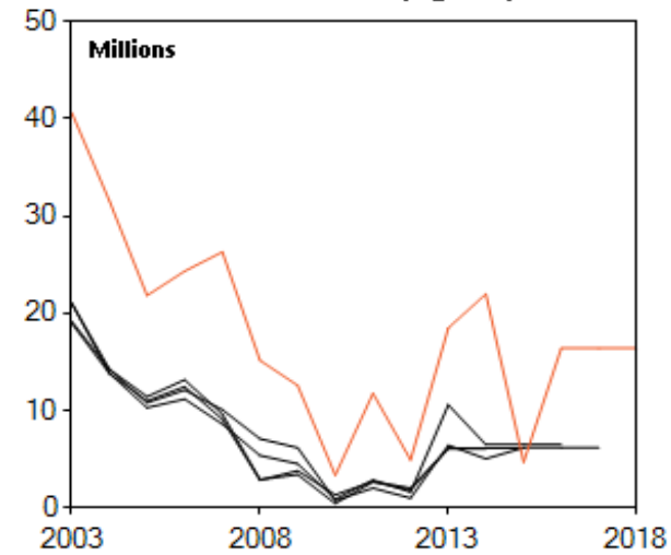
Recruitment (age 0)
