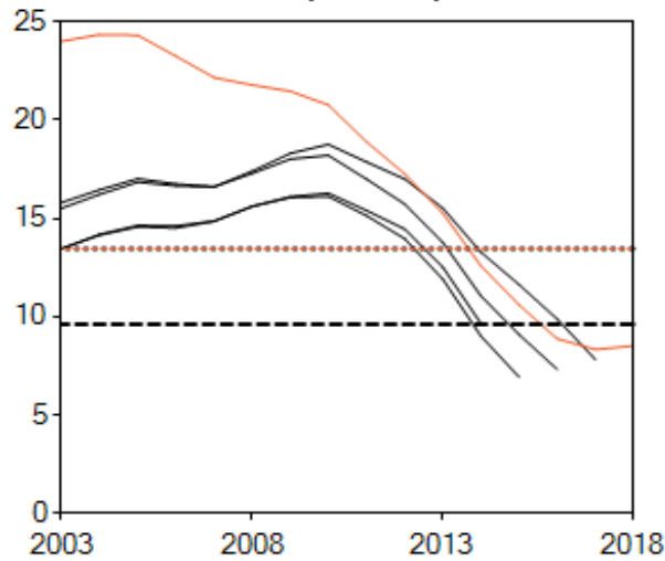
SSB (1000 t)
