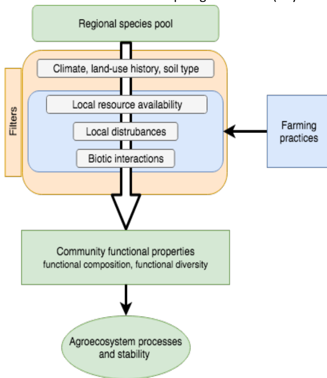
Figure 1. Conceptual framework of this study (modified from Damour et al., 2017). Interconnected environmental and anthropogenic (including farming practices) filters determine the functional properties of the regenerating plant communities. The composition and diversity of response and effect traits will in turn affect agroecosystem processes and its stability in the face of environmental fluctuations.
