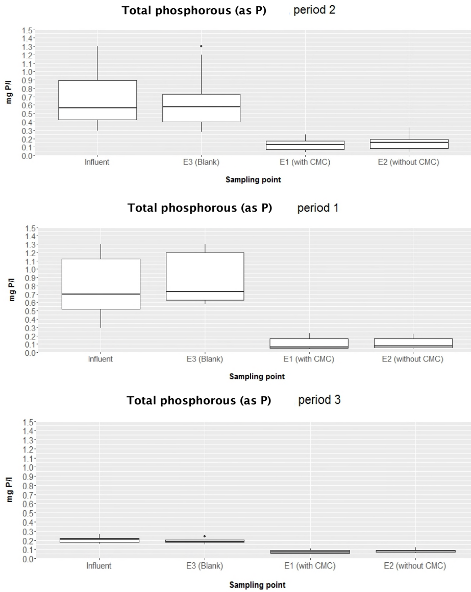
FIGURE 24: EFFECT OF FILTRATION ON TOTAL PHOSPHOROUS (P) CONCENTRATIONS DURING PERIODS 1, 2 AND 3. E1 = EFFLUENT FROM TANK 1 (GIH PELLETS WITH CMC); E2 = EFFLUENT FROM TANK 2 (GIH PELLETS WITHOUT CMC); E3 = EFFLUENT FROM TANK 3 (WITHOUT GIH PELLETS);
