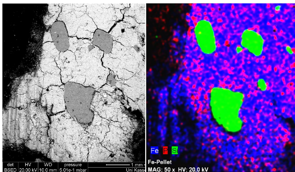
FIGURE 16: X-RAY ANALYSIS OF LOADED IRON PELLETS. RED PARTS INDICATE THE PRESENCE OF PHOSPHOROUS
