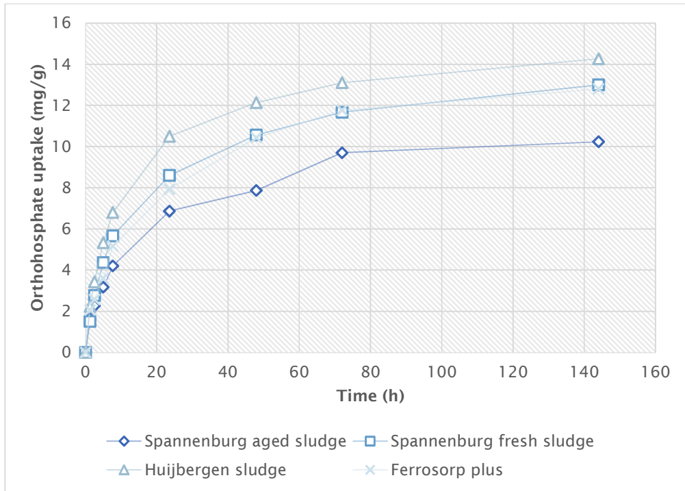
FIGURE 17 UPTAKE OF ORTHOPHOSPHATE AS A FUNCTION OF TIME.
