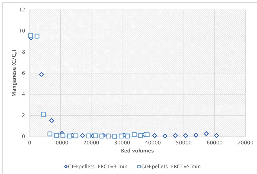
FIGURE 37 MANGANESE BREAKTHROUGH CURVE OF GIH-PELLETS AT PRINSENBOSCH.
