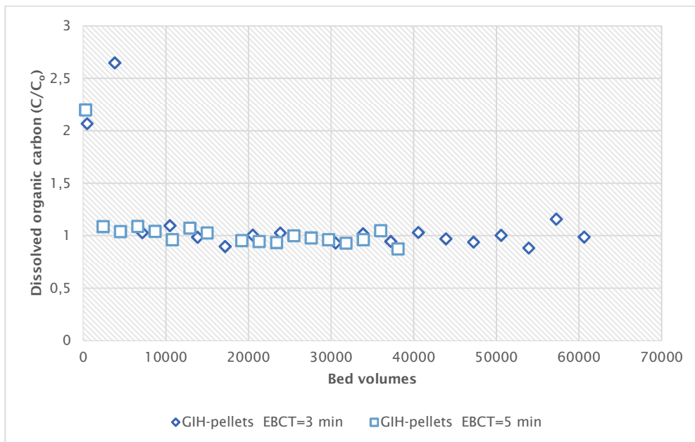
FIGURE 36 DISSOLVED ORGANIC CARBON BREAKTHROUGH CURVE OF GIH-PELLETS AT PRINSENBOSCH.
