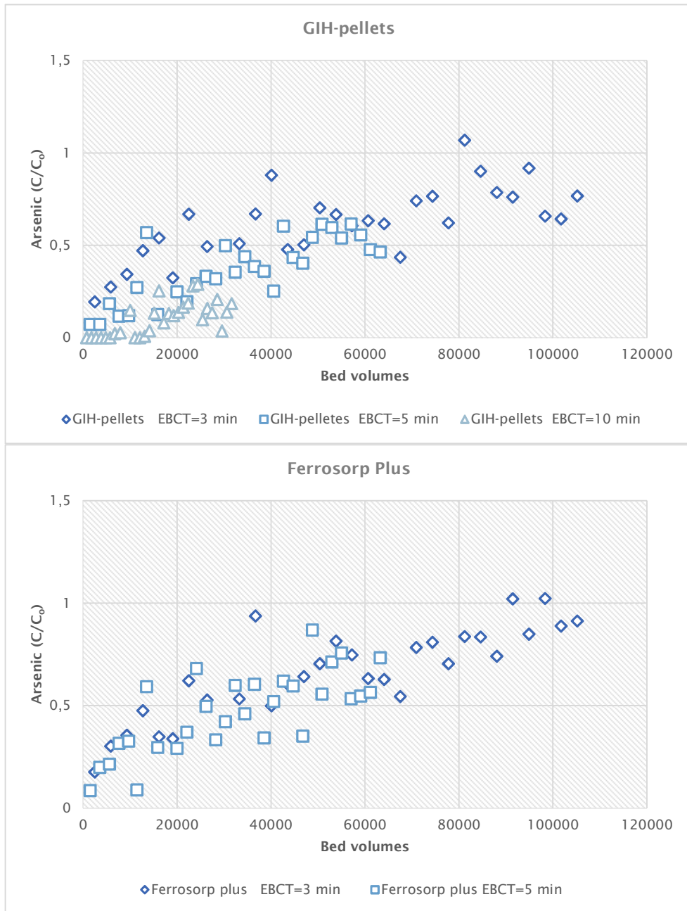
FIGURE 31 ARSENIC BREAKTHROUGH CURVE OF GIH-PELLETS (TOP) AND FERROSORP PLUS (BOTTOM) AT KATWIJK.
