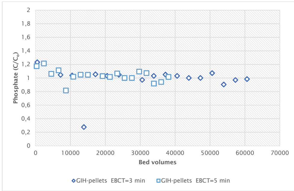
FIGURE 35 ORTHOPHOSPHATE BREAKTHROUGH CURVE OF GIH-PELLETS AT PRINSENBOSCH.
