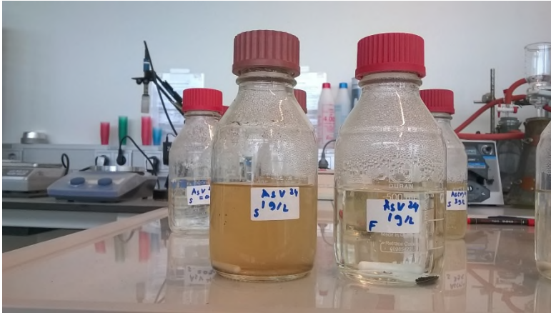
FIGURE 6 STABILITY OF GIH-PELLETS PRODUCED FROM FESH SPANNENBURG RESIDUAL (LEFT) VERSUS FERROSORP PLUS (RIGHT) WHEN MIXING SPEED OF >200 RPM WAS TESTED IN BATCH EXPERIMENTS.
