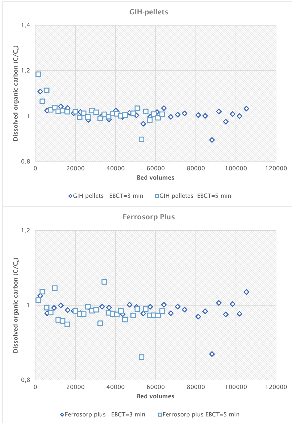
FIGURE 33 TOTAL ORGANIC CARBON BREAKTHROUGH CURVE OF GIH-PELLETS (TOP) AND FERROSORP PLUS (BOTTOM) AT KATWIJK.
