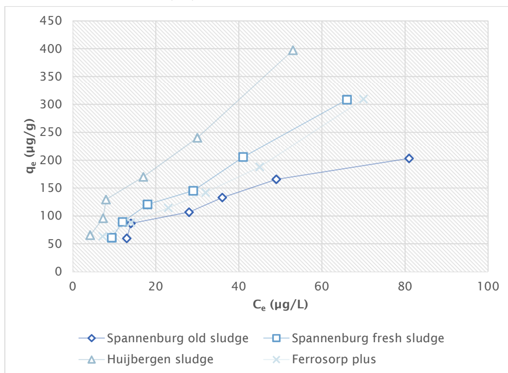
FIGURE 28 ADSORPTION ISOTHERMS OF As ONTO GIH-PELLETS AND FERROSORP PLUS AT 15°C.
