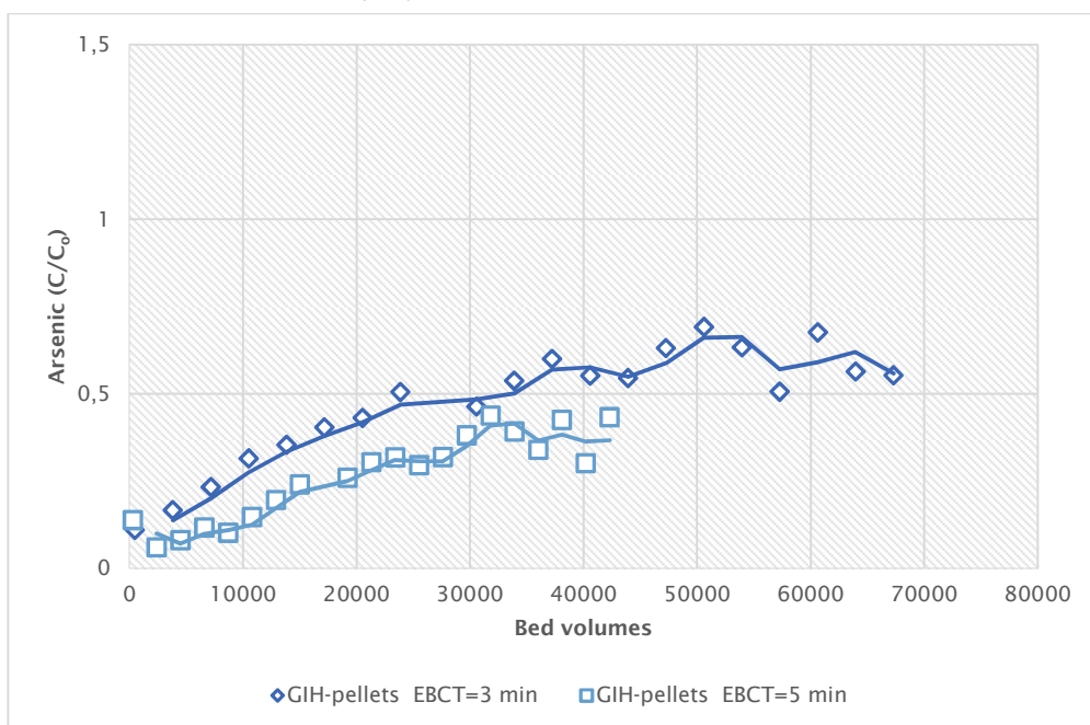
FIGURE 34 ARSENIC BREAKTHROUGH CURVE OF GIH-PELLETS AT PRINSENBOSCH.
