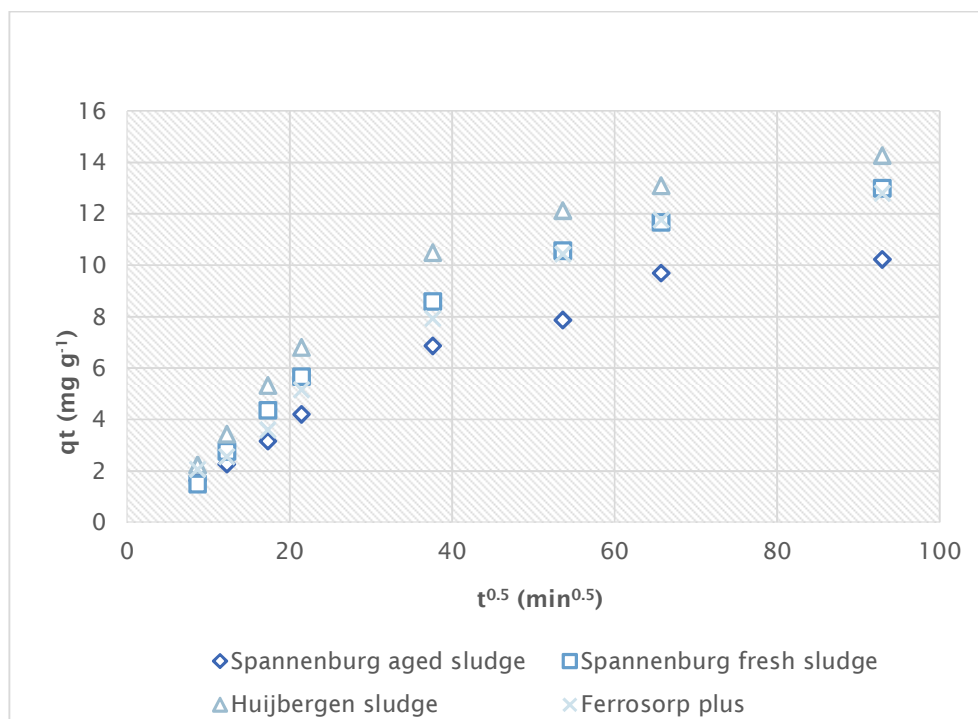
FIGURE 42 PLOT OF q_t AGAINST t^{0.5} . APPLICATION OF INTRA-PARTICLE DIFFUSION MODEL TO THE EXPERIMENTAL DATA OF FIGURE 5-1.
