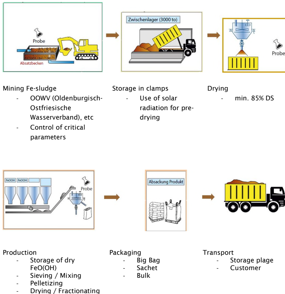
FIGURE 38: PRODUCTION PROCESS FOR GIH PELLETS (INFORMATION FROM AGRAVIS)
