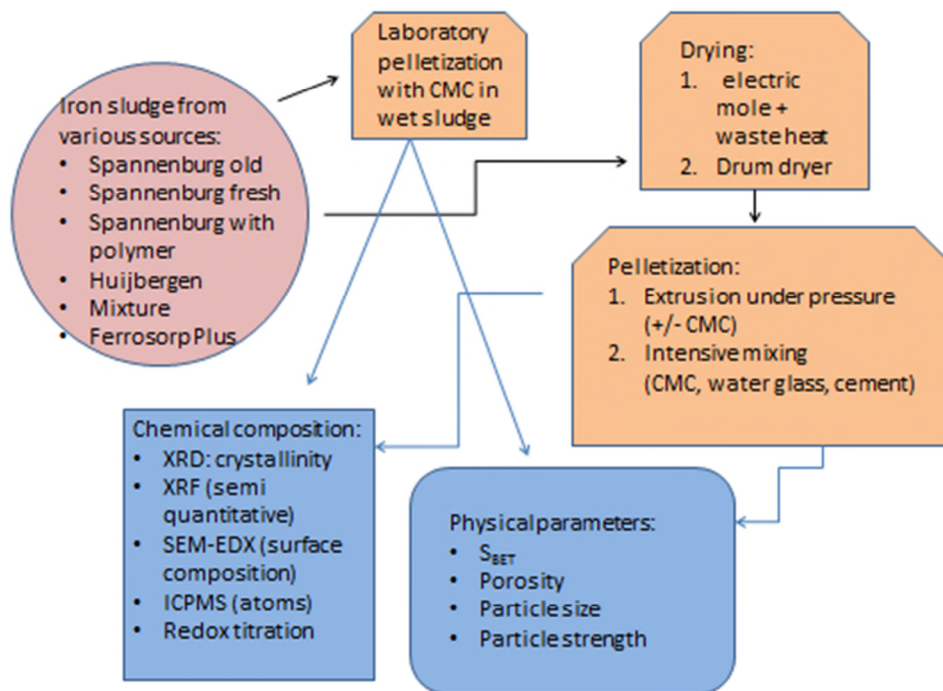
FIGURE 1: CHARACTERIZATION OF VARIOUS SLUDGES AND PELLETS.
