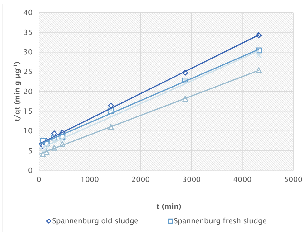
FIGURE 43 PLOT OF t/q_t AGAINST t . APPLICATION OF PSEUDO-SECOND ORDER KINETIC MODEL TO THE EXPERIMENTAL DATA OF FIGURE 7-1
