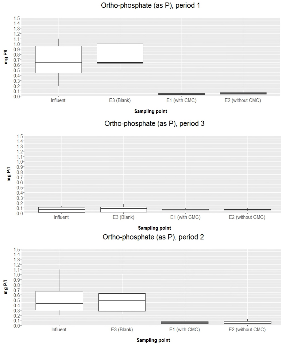
FIGURE 22: EFFECT OF FILTRATION ON ORTHOPHOSPHATE CONCENTRATIONS DURING THE PILOT TESTS. E1 = EFFLUENT FROM TANK 1 (GIH PELLETS WITH CMC); E2 = EFFLUENT FROM TANK 2 (GIH PELLETS WITHOUT CMC); E3 = EFFLUENT FROM TANK 3 (WITHOUT GIH PELLETS)
