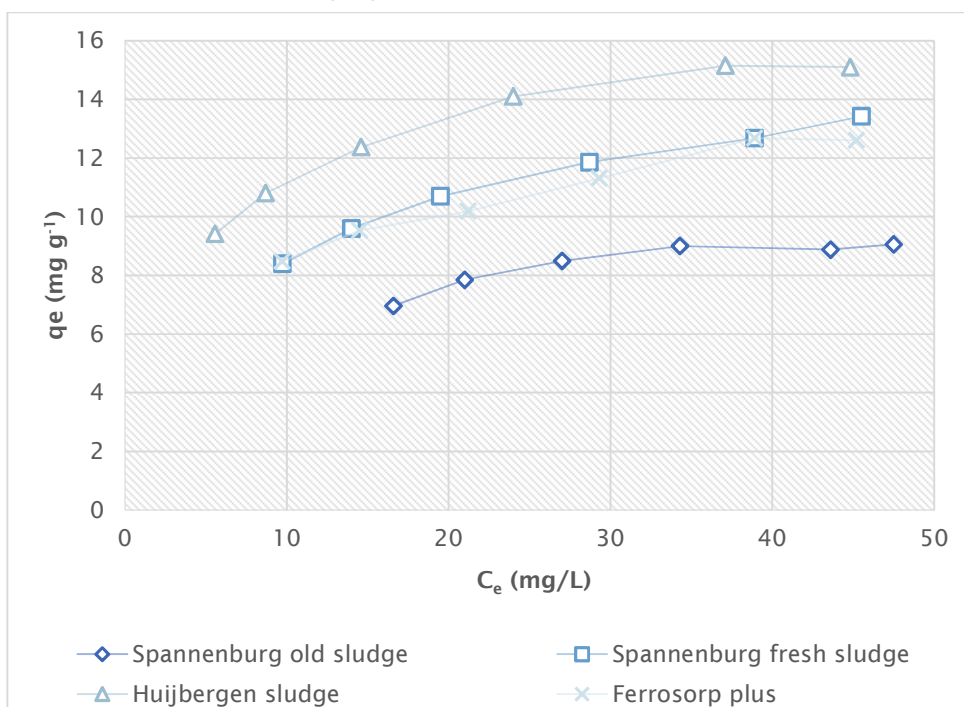
FIGURE 18 ADSORPTION ISOTHERMS OF ORTHO-PO 4 ONTO GIH PELLETS AND FERROSORP PLUS AT 15°C.
