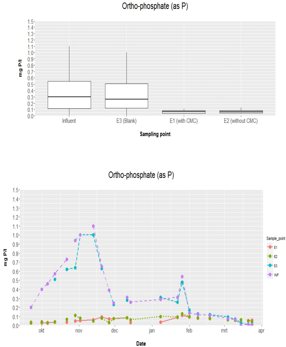
FIGURE 23: ORTHOPHOSPHATE CONCENTRATIONS IN INFLUENT AND EFFLUENTS DURING THE EXPERIMENTAL PERIOD. E1 = EFFLUENT FROM TANK 1 (GIH PELLETS WITH CMC); E2 = EFFLUENT FROM TANK 2 (GIH PELLETS WITHOUT CMC); E3 = EFFLUENT FROM TANK 3 (WITHOUT GIH PELLETS);
