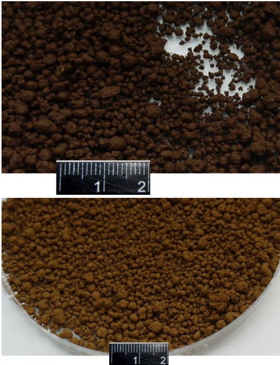
FIGURE 14: PELLETS MADE WITH DIFFERENT BINDERS, USING A DRUM DRYER AND INTENSIVE MIXING. UPPER PICTURE: CEMENT AS BINDING MATERIAL; LOWER PICTURE: SODIUM WATER GLASS AS BINDING MATERIAL.
