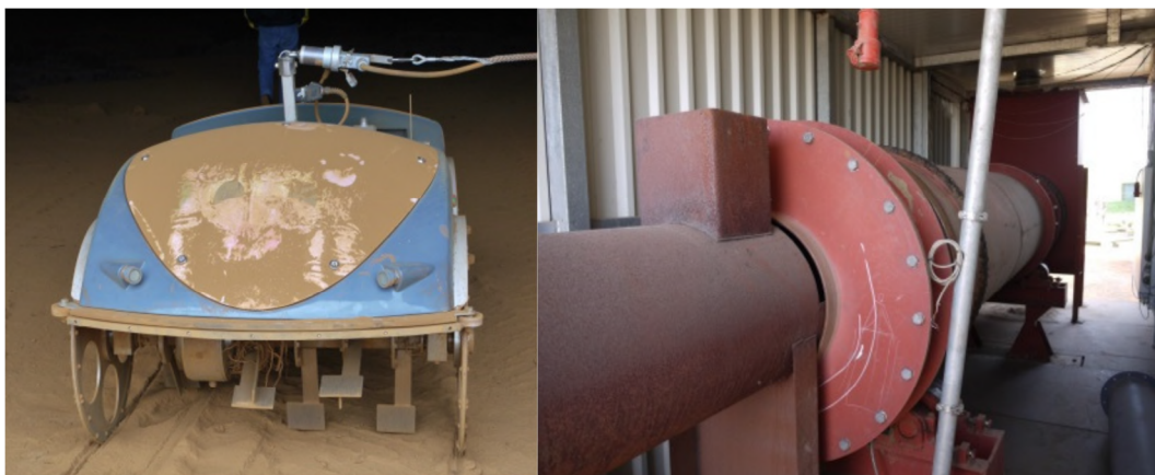
FIGURE 11: DRYING BY MEANS OF AN ELECTRIC MOLE (LEFT) OR BY MEANS OF A DRUM DRYER (RIGHT).
