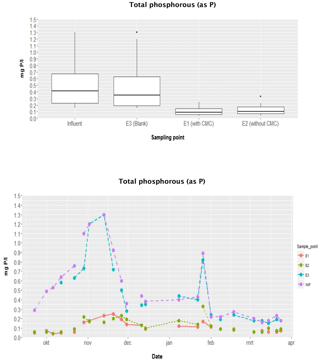
FIGURE 25: DEVELOPMENT OF TOTAL PHOSPHOROUS (AS P) CONCENTRATIONS DURING THE EXPERIMENTAL PERIOD. E1 = EFFLUENT FROM TANK 1 (GIH PELLETS WITH CMC); E2 = EFFLUENT FROM TANK 2 (GIH PELLETS WITHOUT CMC); E3 = EFFLUENT FROM TANK 3 (WITHOUT GIH PELLETS);
