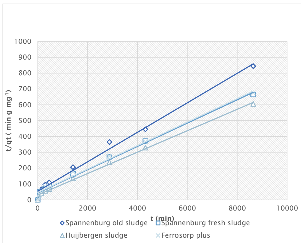
FIGURE 41 PLOT OF t/q_t AGAINST t . APPLICATION OF PSEUDO-SECOND ORDER KINETIC MODEL TO THE EXPERIMENTAL DATA OF FIGURE 5-1.
