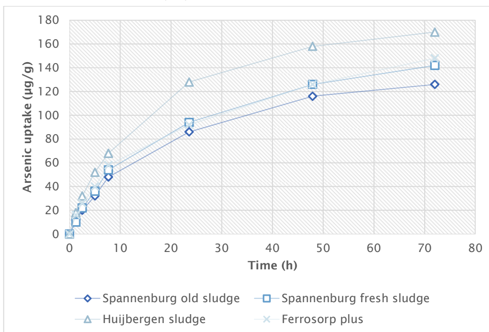
FIGURE 27 UPTAKE OF As AS A FUNCTION OF TIME.
