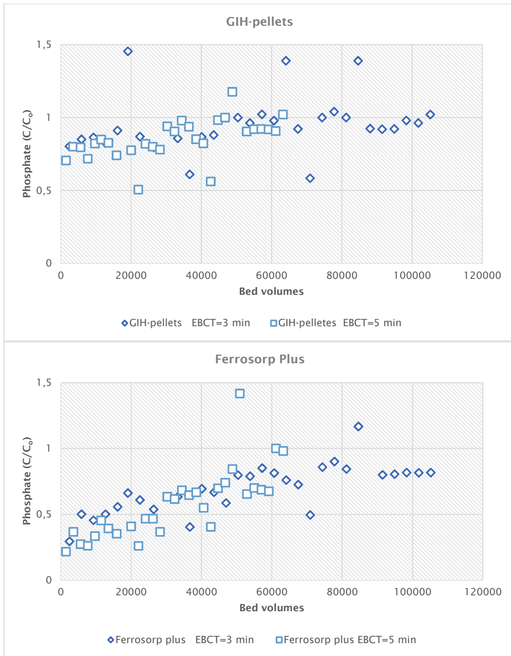
FIGURE 32 ORTHOPHOSPHATE BREAKTHROUGH CURVE OF GIH-PELLETS (TOP) AND FERROSORP PLUS (BOTTOM) AT KATWIJK.
