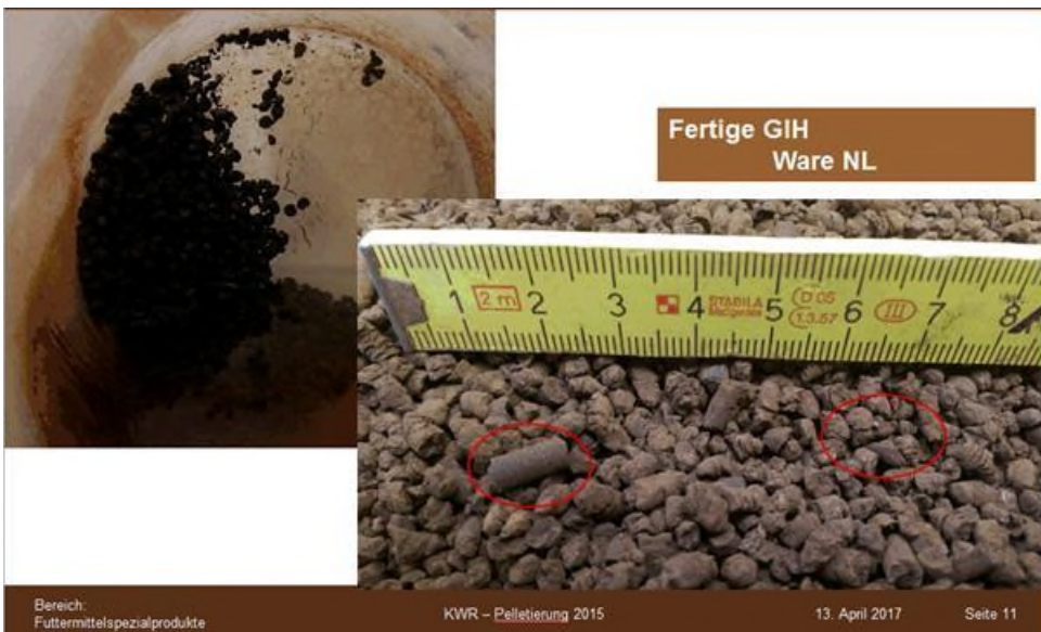
FIGURE 10 GIH-PELLETS PRODUCED BY EXTRUSION.
