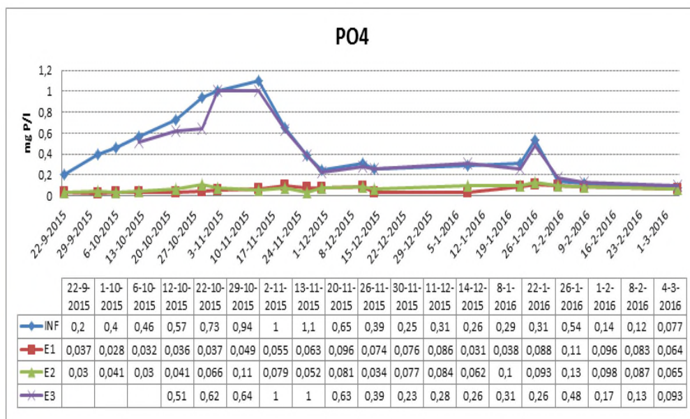
FIGURE 26: PHOSPHATE CONCENTRATIONS IN INFLUENT AND ALL THREE EFFLUENTS DURING THE EXPERIMENTAL PERIOD. E1 = EFFLUENT FROM TANK 1 (GIH PELLETS WITH CMC); E2 = EFFLUENT FROM TANK 2 (GIH PELLETS WITHOUT CMC); E3 = EFFLUENT FROM TANK 3 (WITHOUT GIH PELLETS);
