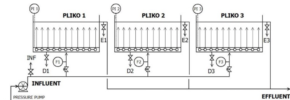
FIGURE 21: PROCESS FLOW DIAGRAM OF THE PILOT SET-UP AT THE SLOTTERPLAS IN AMSTERDAM
