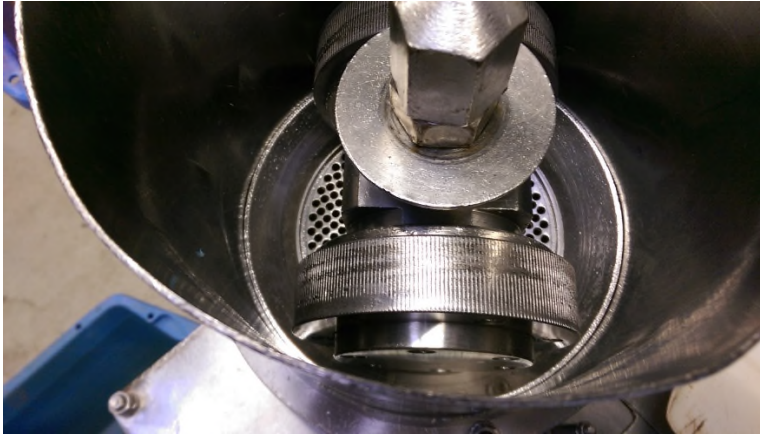
FIGURE 9 THE FLAT DIE PRESS USED FOR EXTRUSION PELLETISING.
