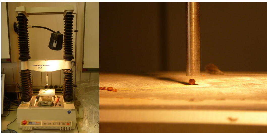
FIGURE 15: ROBOTIC COMPRESSION TESTER.
