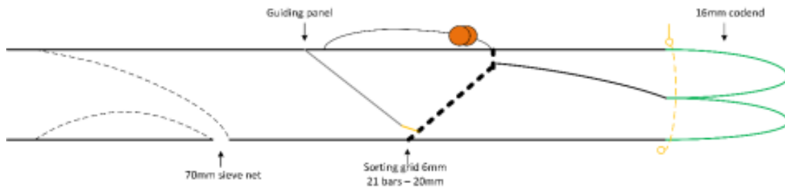
Figure 9: Details of Single-grid gear Design 1
