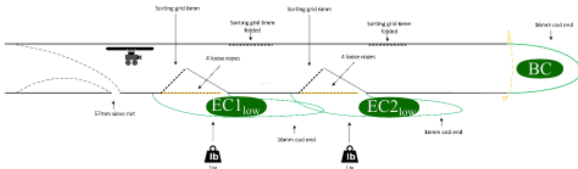
Figure 19: Details of Multi-grid gear design MG5
