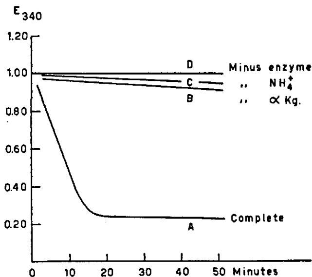
Fig. 1. The rates of DPNH oxidation by an extract of tomato root mitochondria in the presence (curve A) and in the absence (curves B and C, respectively) of \alpha -ketoglutarate and ammonium ions. Curve D represents the same as curve A, except that the enzyme extract was omitted.
