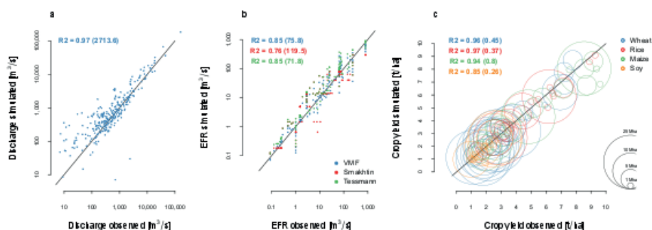
Figure 4.4: Evaluation of LPJmL-simulated key variables. Validation results against observational data are highlighted for mean annual discharge (a), environmental flow requirements respectively for three differing calculation methods (b), and country-level crop yields (calibrated for management intensity) for main staple crops and the respective top 30 producer countries, chart symbols are scaled by country cropland extent (c). The coefficient of determination ( R^2 ) is shown along with the root mean square error in parenthesis (all data 1980-2009, further details in Methods).
