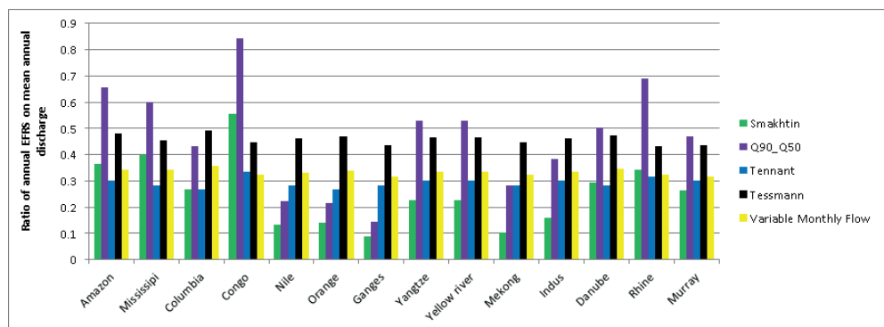
Figure 2.7. Comparison of five environmental flow methods at the outlet of 14 river basins.
