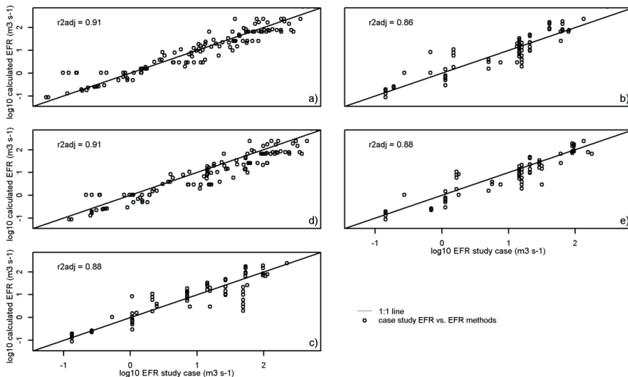
Figure 2.3. Relation between the monthly calculated EFRs and the locally calculated monthly EFRs of 11 case studies with the (a) Variable Monthly Flow, (b) Smakhtin, (c) Tessmann, (d) Q_{90\_Q_{50}} , (e) Tennant methods. In each sub-figure, each dot represents EFRs for one month and for one case study.
