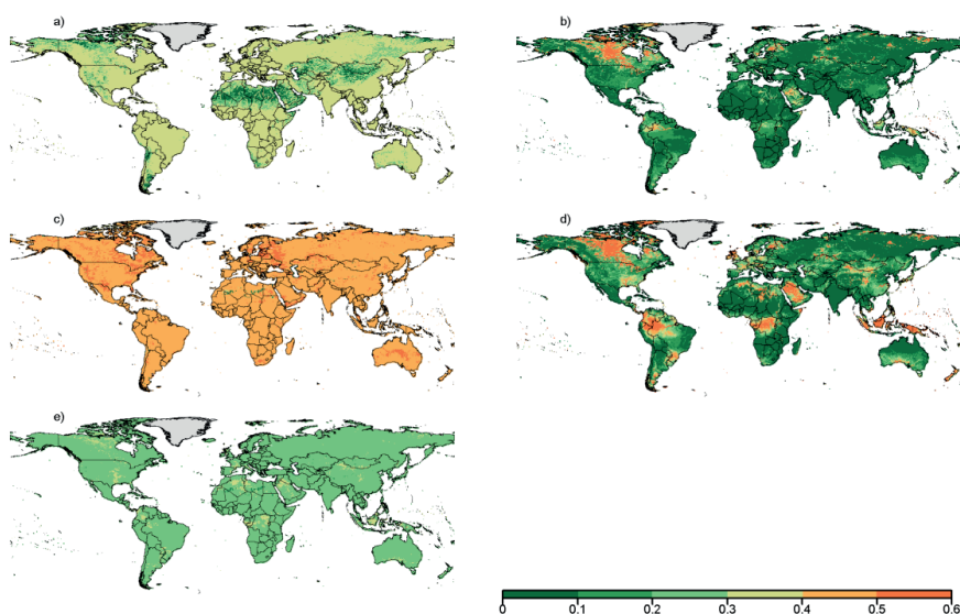
Figure 2.4. Ratios of annual environmental flow by annual natural flow within a) Variable Monthly Flow, b) Smakhtin, c) Tessmann, d) Q_{90} - Q_{50} , e) Tennant environmental flow methods.
