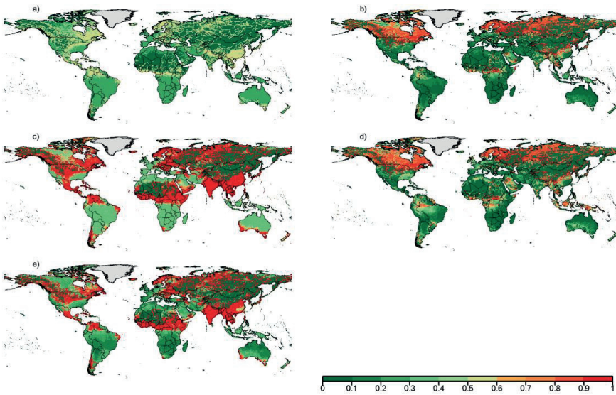
Figure 2.5. Ratios of monthly environmental flow by monthly actual flow (January) within a) Variable Monthly Flow, b) Smakhtin, c) Tessenmann, d) Q_{90}-Q_{50} , e) Tennant environmental flow methods.
