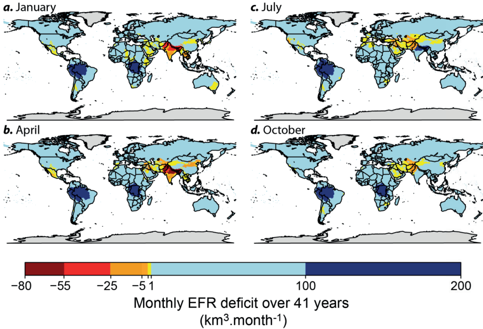
Figure 3.2. Spatial representation of monthly deficit at global scale for four months: Jan, Apr, Jul, Oct averaged over 41 years. Units are in \text{km}^3 \cdot \text{month}^{-1} . Negative values represent deficit of flow (in yellow/orange/red) whereas positive values (in blue) represent surpluses of flow.
