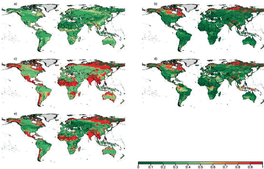
Figure 2.6. Ratios of monthly environmental flow by monthly actual flow (April) within a) Variable Monthly Flow, b) Smakhtin, c) Tessenmann, d) Q_{90}-Q_{50} , e) Tennant environmental flow methods.
