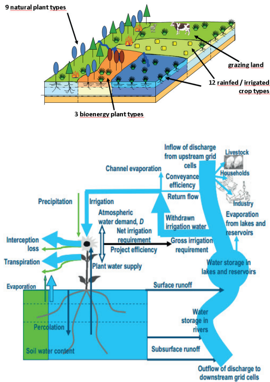
Figure 1.3. Representation of LPJmL with the dynamic module (upper plot - adapted from (Hoff 2011)) and river routine scheme (down plot) (Rost, Gerten et al. 2008)
