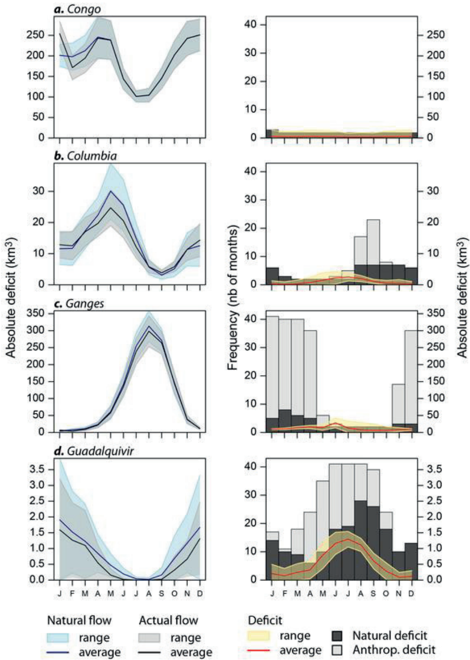
Figure 3.5. Temporal representation of natural and actual flow (left plot) with intra-annual monthly deficit ( \text{km}^3 \text{ month}^{-1} ) and frequency of deficit (number of months) for four river basins representing each group of river basins. Y axis represent absolute flow and deficit have the same scale to enable comparison, Barplots (right plot) represent the frequency of natural deficit (black) and anthropogenic deficit (grey). Total Environmental Deficit (EF) (yellow range-right plot) was shown with positive values for comparison with the flow (blue/grey range – left plot).
