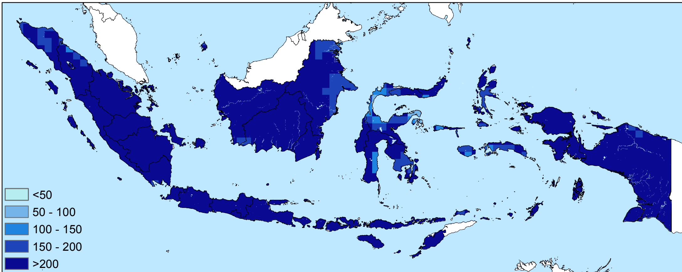
Average precipitation total in January (mm/month)
