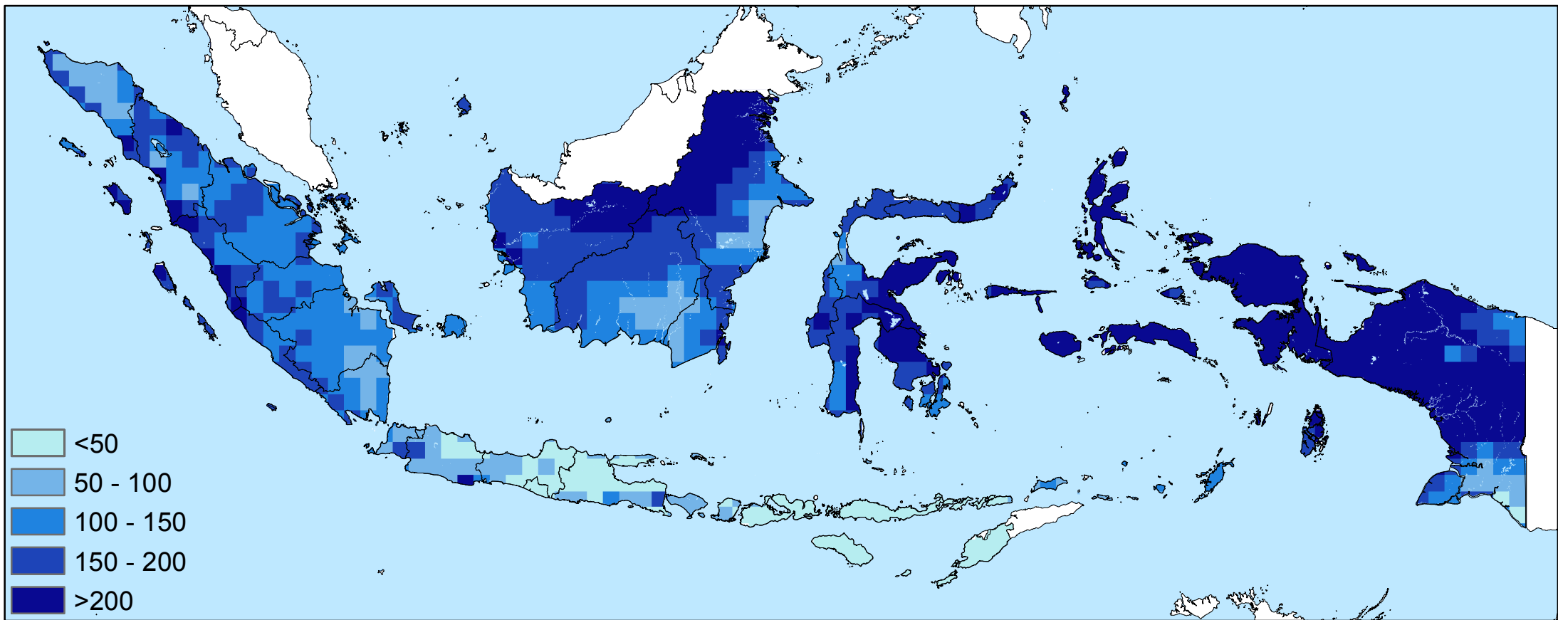
Average precipitation total in July (mm/month)
