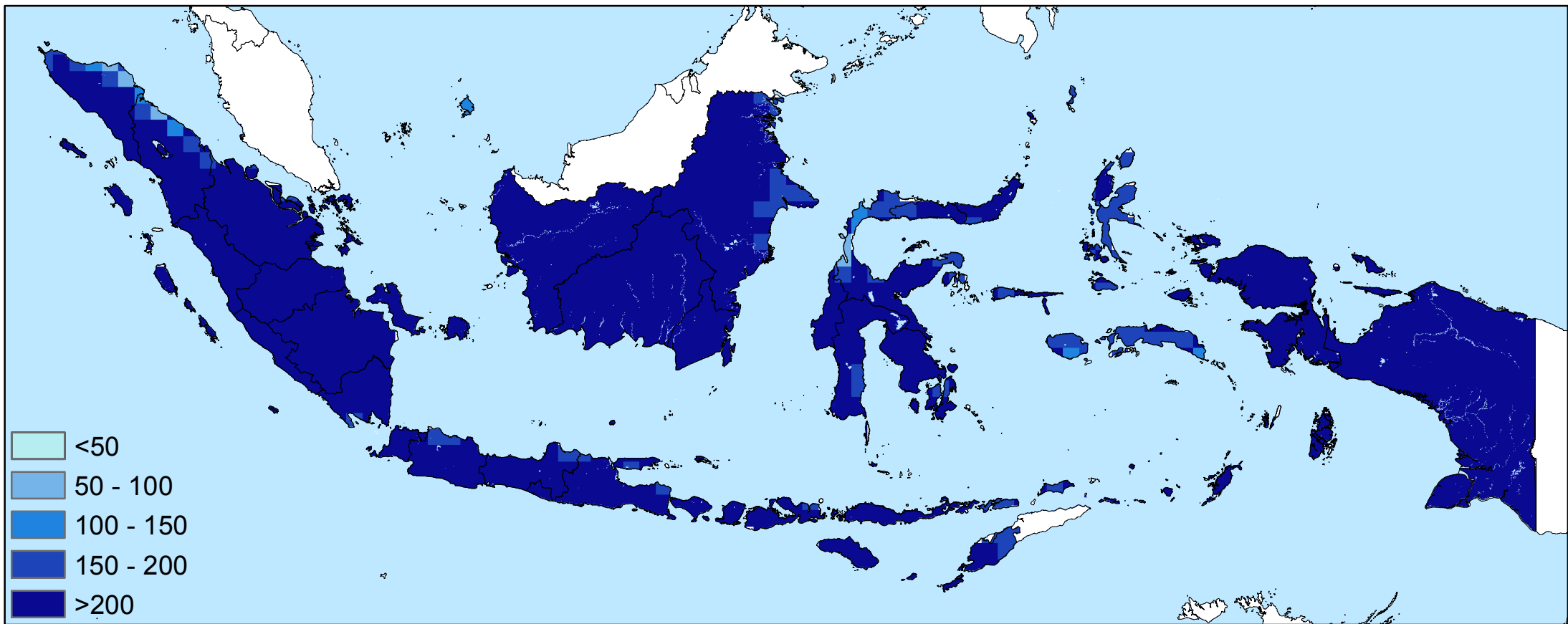
Average precipitation total in March (mm/month)
