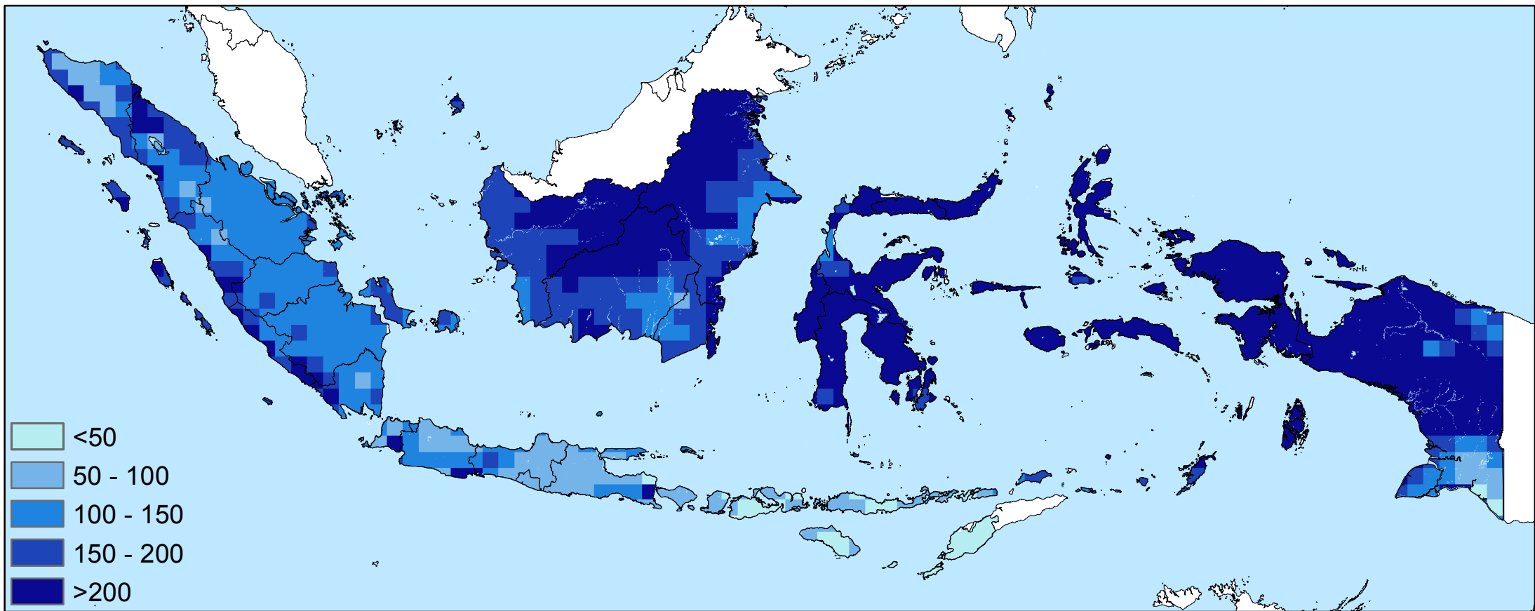
Average precipitation total in June (mm/month)
