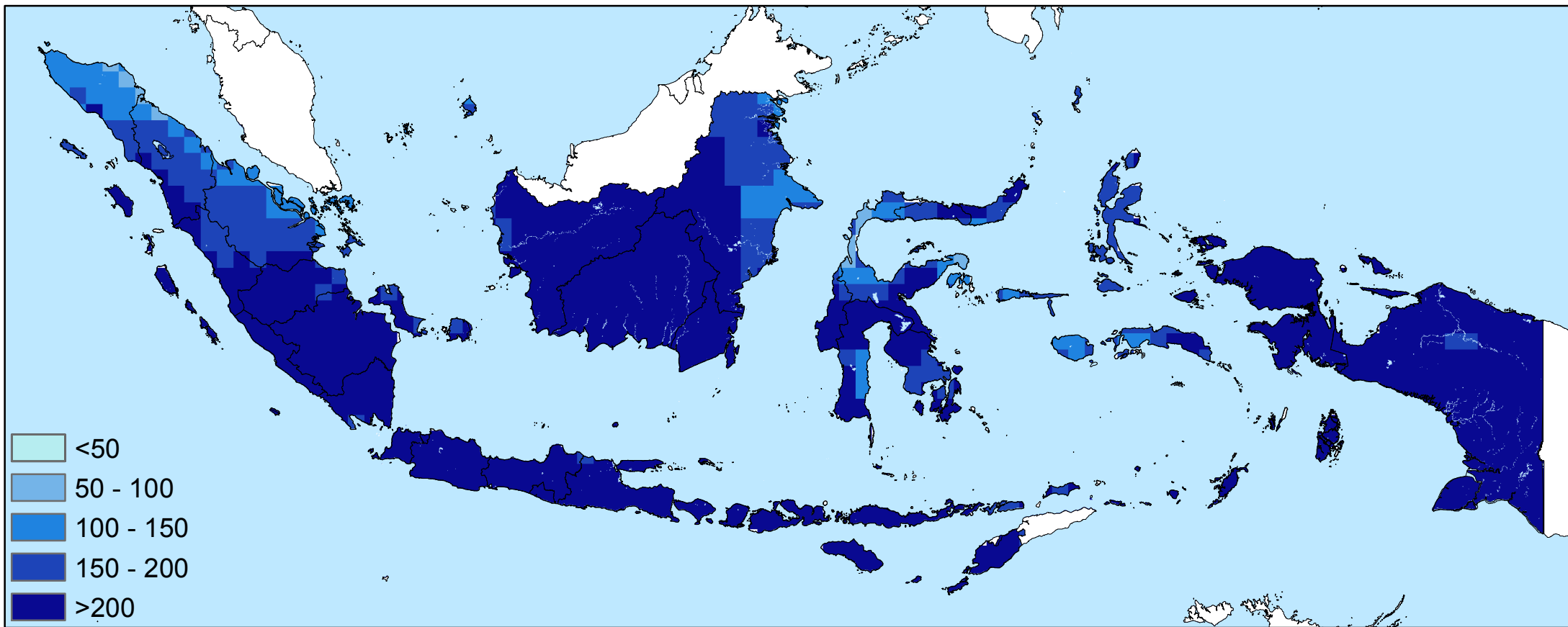
Average precipitation total in February (mm/month)
