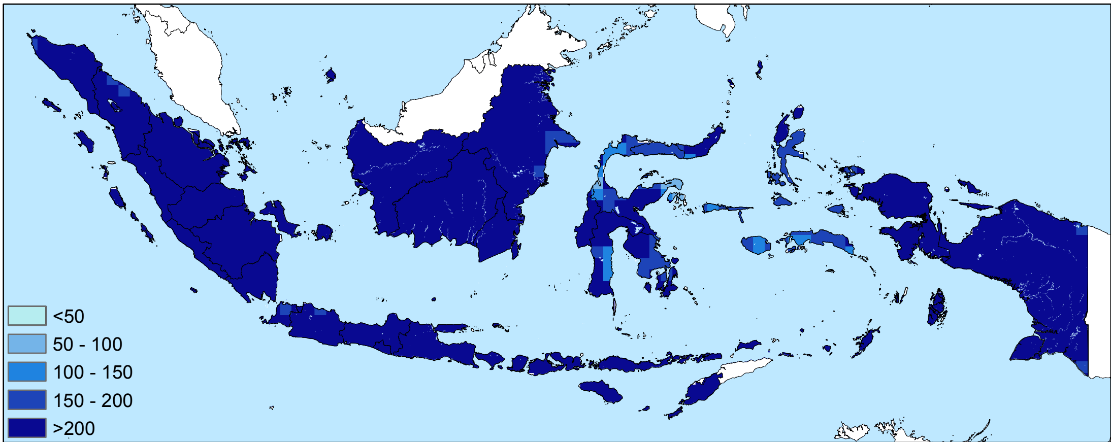
Average precipitation total in December (mm/month)
