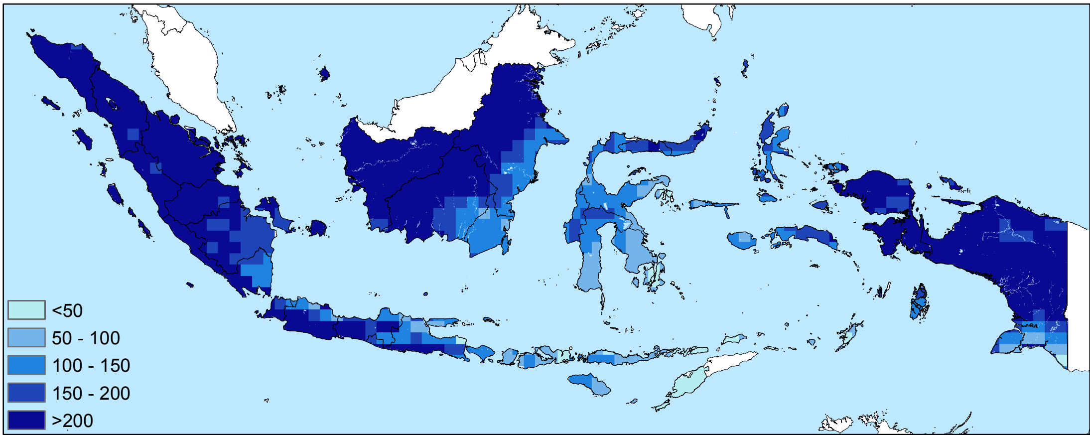
Average precipitation total in October (mm/month)
