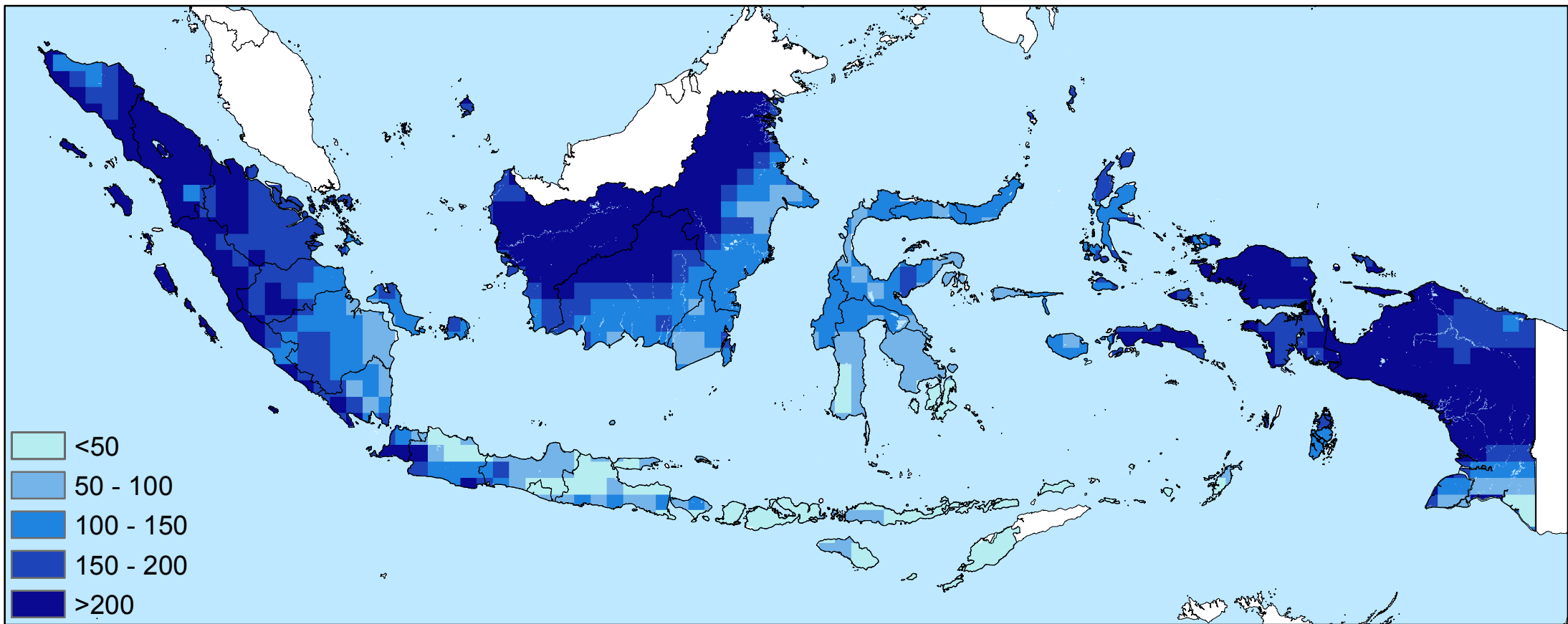
Average precipitation total in September (mm/month)
