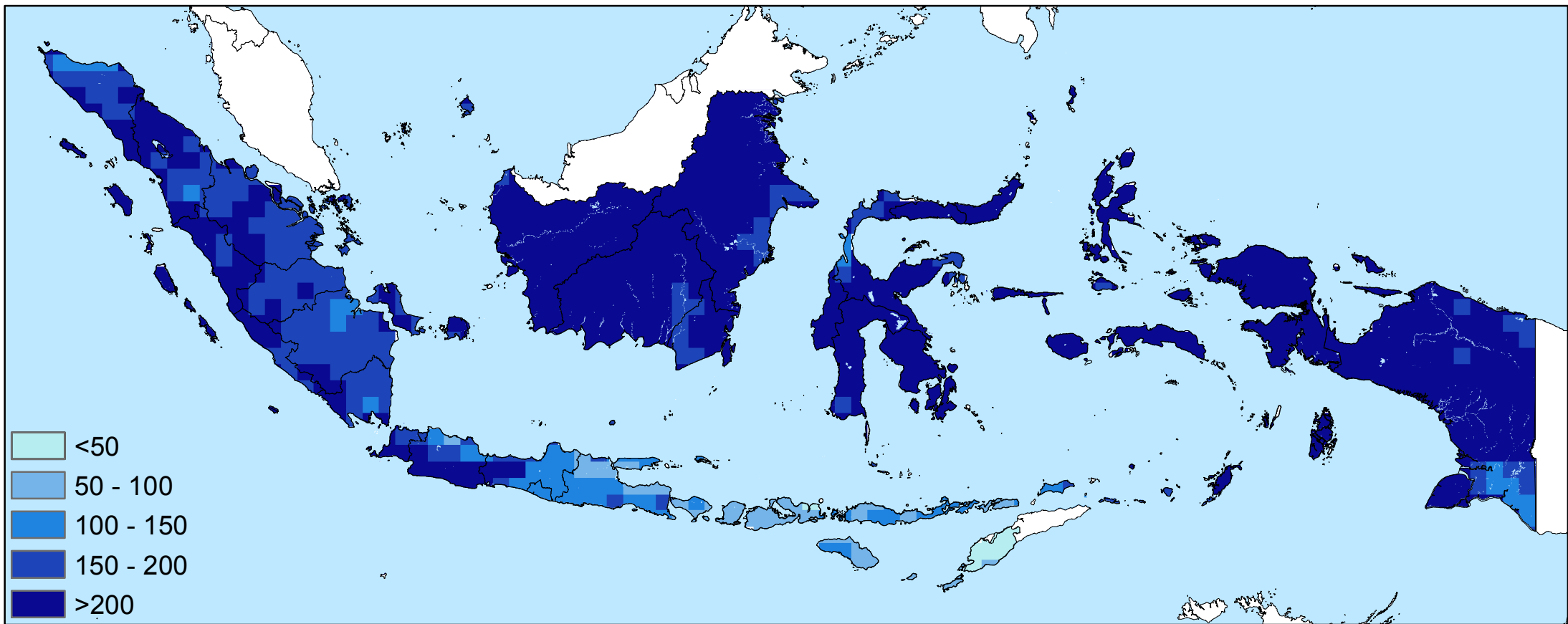
Average precipitation total in May (mm/month)
