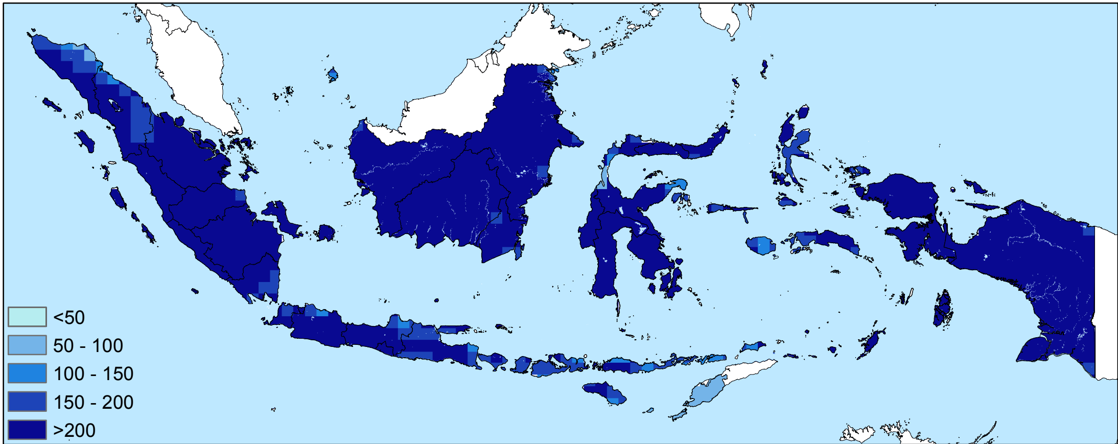
Average precipitation total in April (mm/month)
