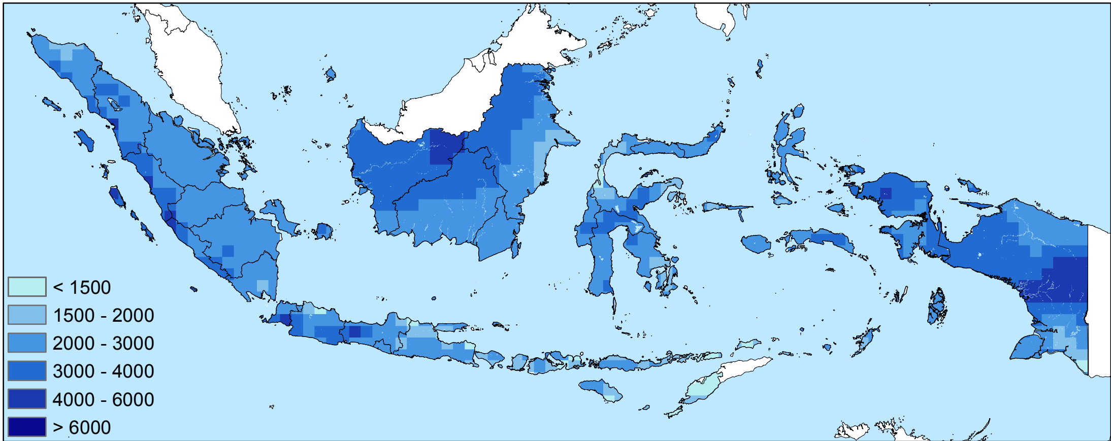
Average precipitation total (mm/year)
