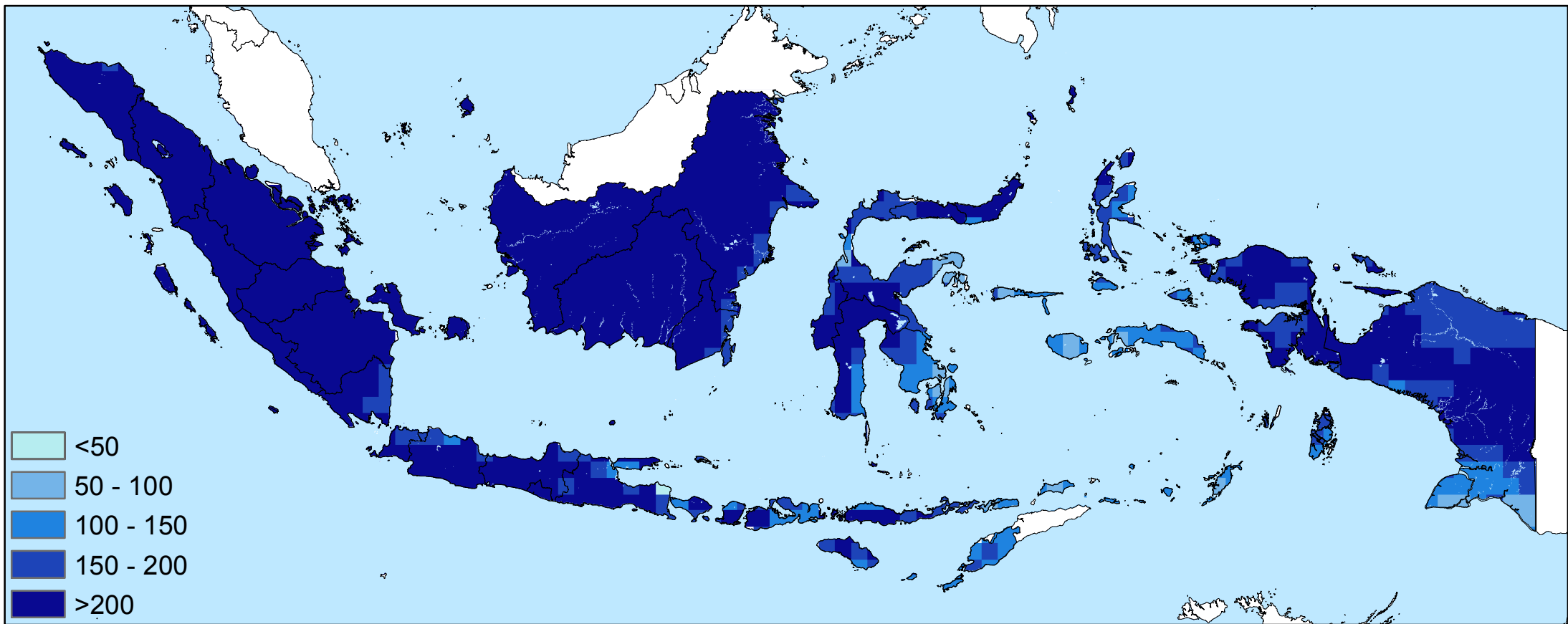
Average precipitation total in November (mm/month)
