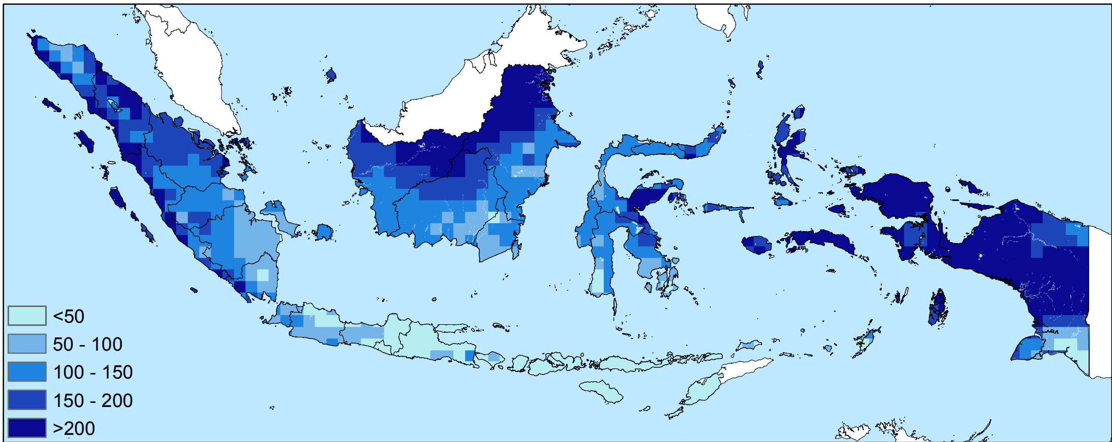
Average precipitation total in August (mm/month)
