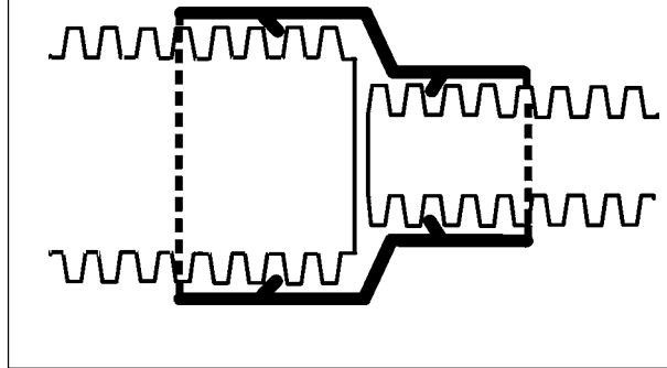
FIGURE 3 Drainpipe reducer
