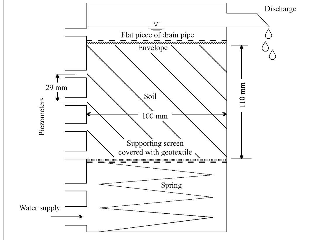
FIGURE 44 Cross section of a permeameter apparatus for evaluating soil-envelope interactions
