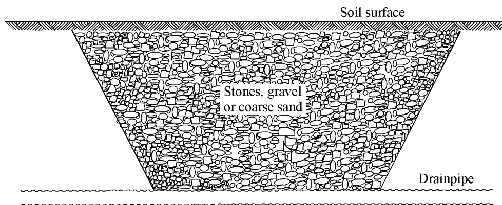
FIGURE 7 Blind inlet
