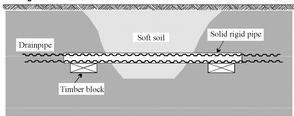
FIGURE 5 Drain bridge
