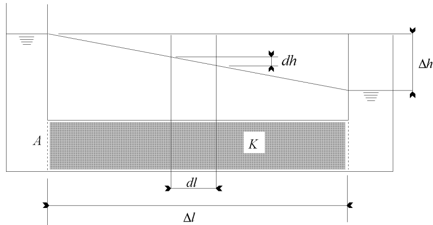
FIGURE 25 Horizontal flow
