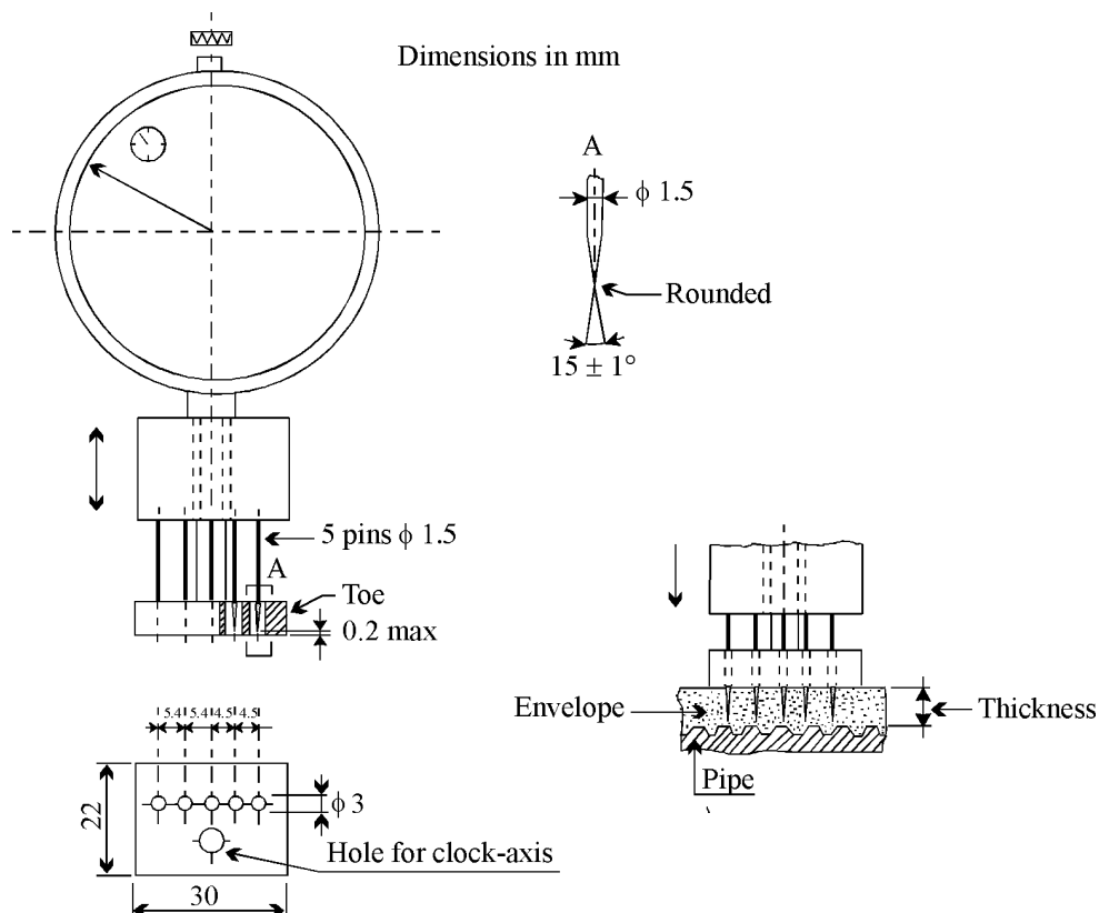
FIGURE B.1 Measuring device for the determination of the minimum thickness
