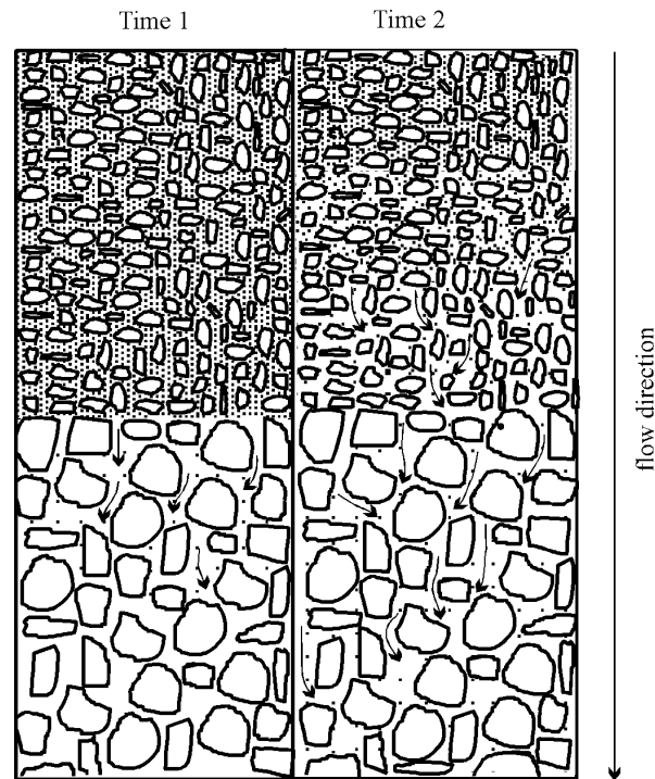
FIGURE 33 Natural filter (after Stuyt, 1982)
