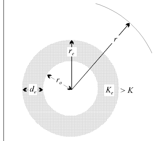
FIGURE 31 Theoretical flow towards an ideal drain surrounded by an envelope
