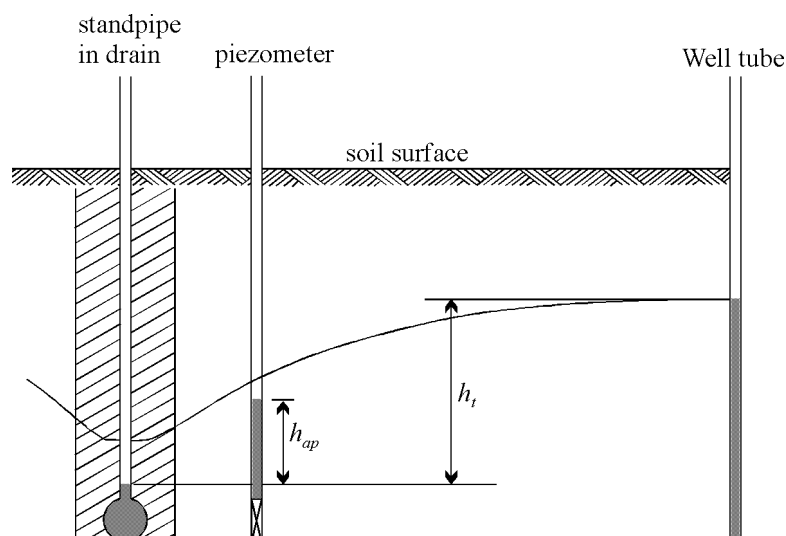
FIGURE 23 Approach flow and total head loss to evaluate drainage performance in experimental fields
