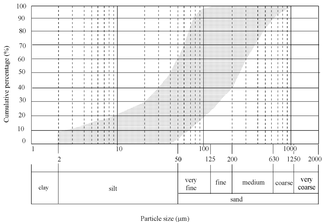
FIGURE 42 Range of particle size distribution of soils that may cause clogging of drains
