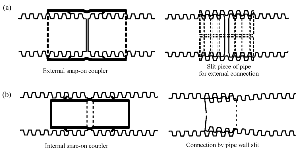
FIGURE 2 Couplers
