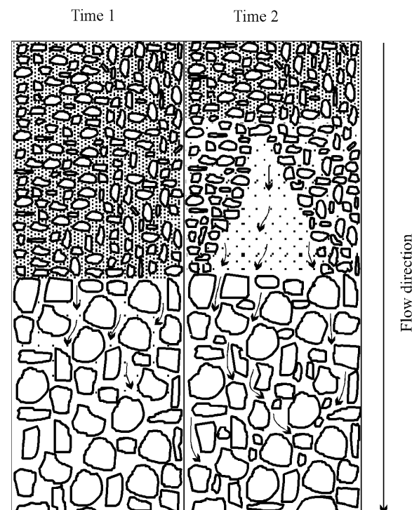
FIGURE 34 Contact erosion (after Stuyt, 1982)
