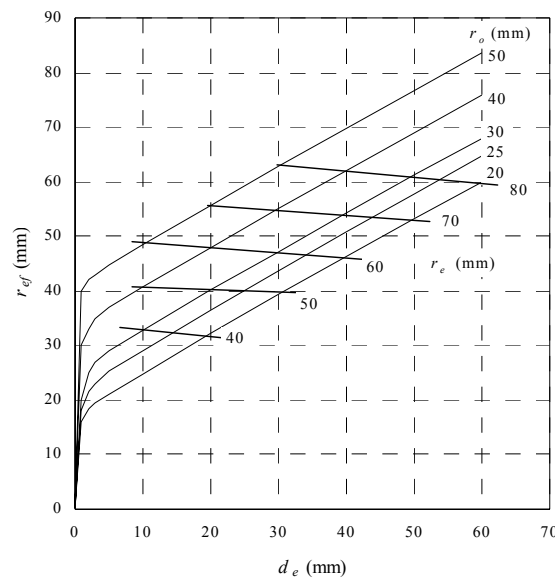
FIGURE 32 Effective radii, r_{ef} , for drains of different pipe radii, r_o , and provided with four continuous longitudinal slits as a function of the envelope thickness d_e for K_e = 10
