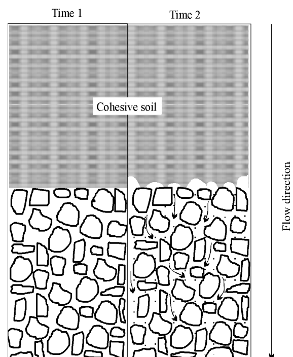
FIGURE 36 Soil collapse (after Stuyt, 1982)
