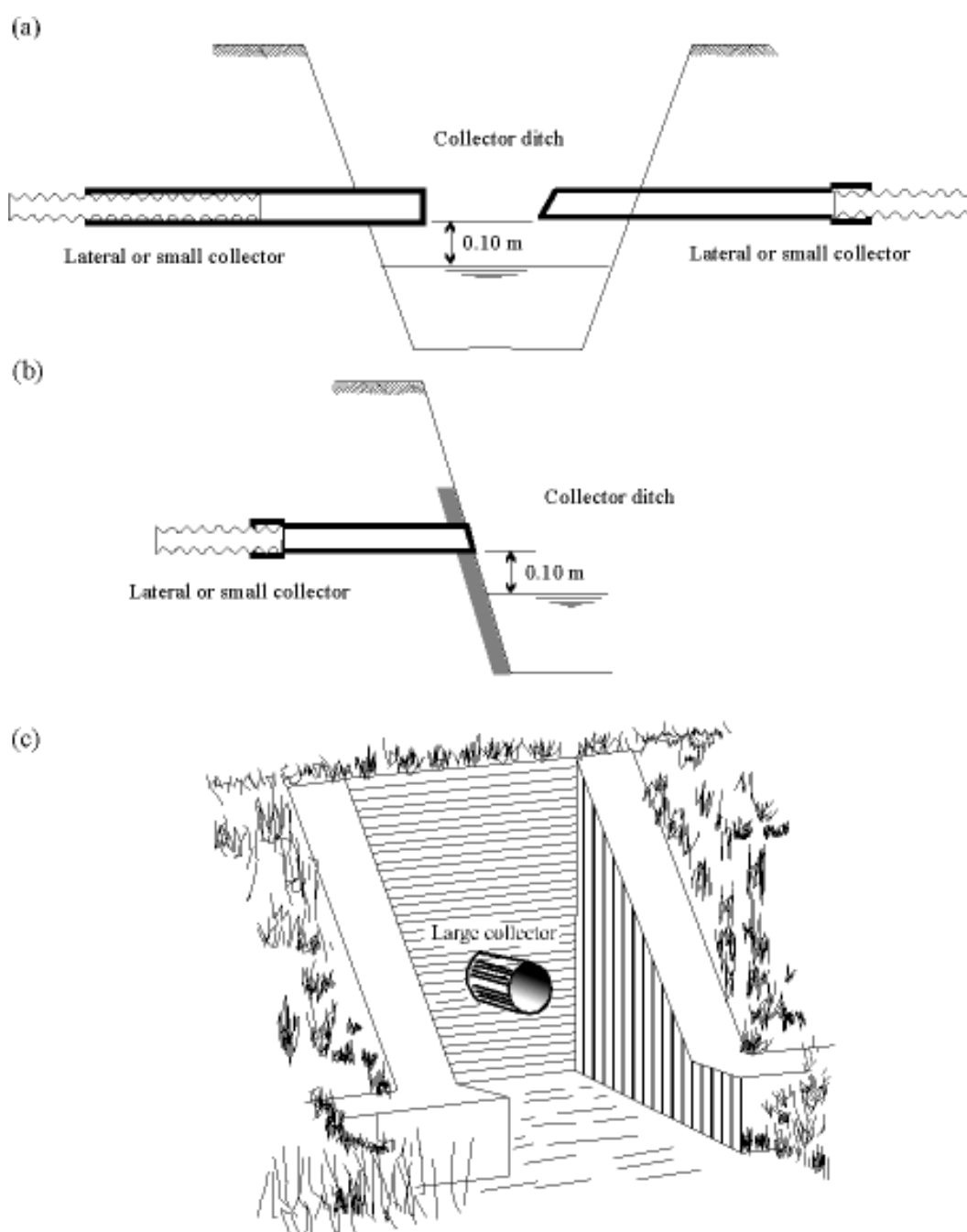
FIGURE 11 Gravity outlets
