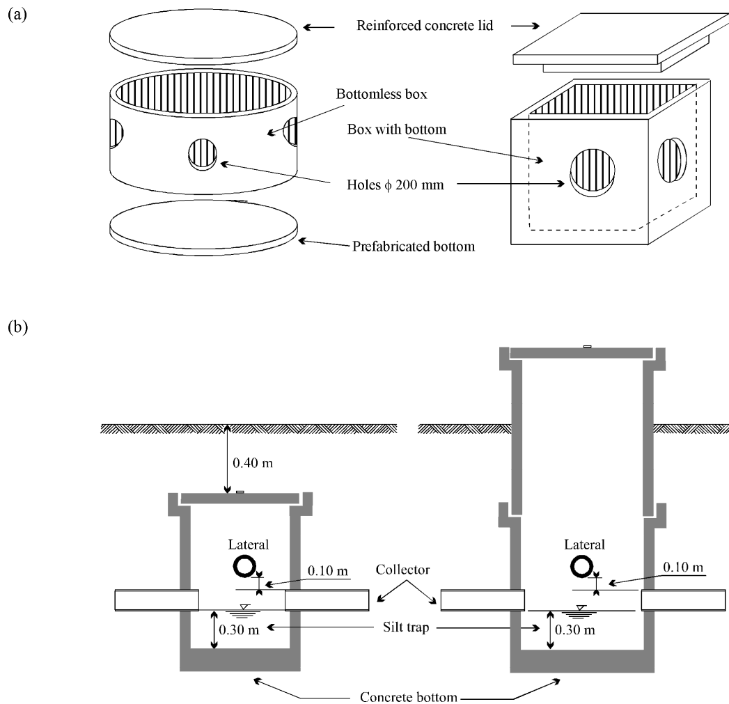
FIGURE 9 Junction boxes
