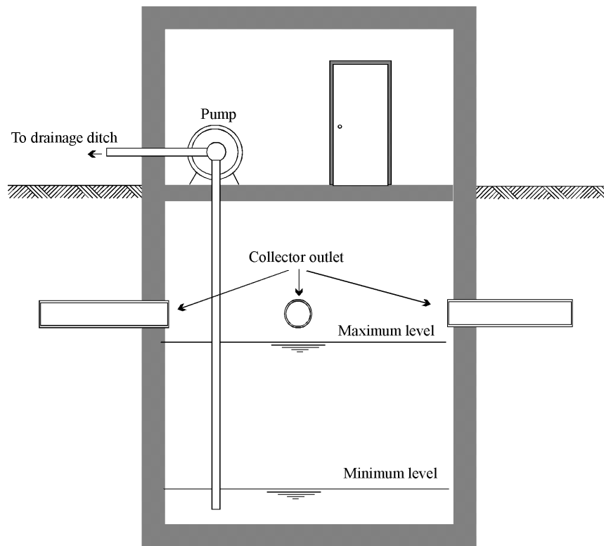
FIGURE 12 Drainage pump sump
