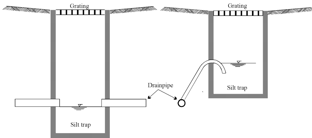
FIGURE 8 Surface inlets
