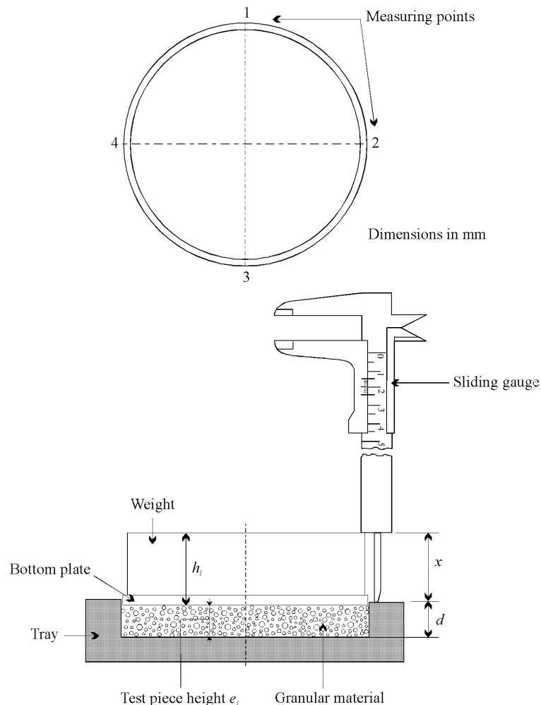
FIGURE D.5 Thickness determination under load of a test piece of granular envelopes
