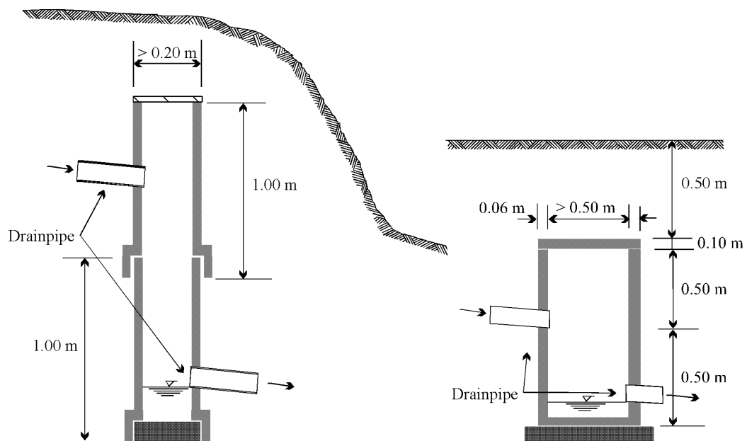
FIGURE 13 Gradient reducers (after Eggelsmann, 1978)
