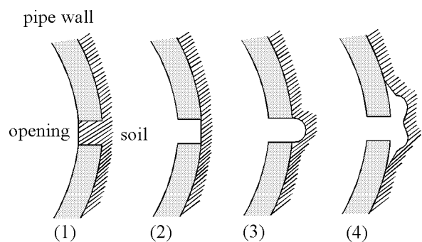
FIGURE 30 Possible boundaries between soil and drain openings (after Cavelaars, 1970)
