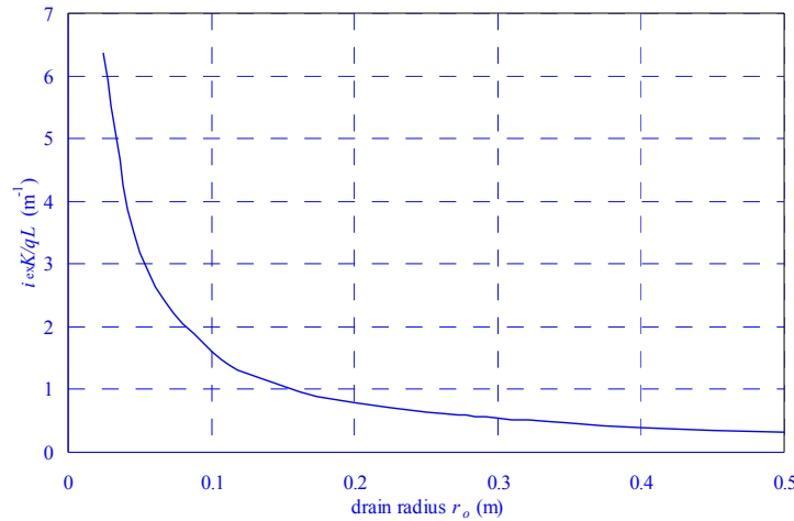
FIGURE 27 Exit gradient i_{ex} , expressed as the ratio i_{ex}K/qL for radial flow as a function of the drain radius, r_o
