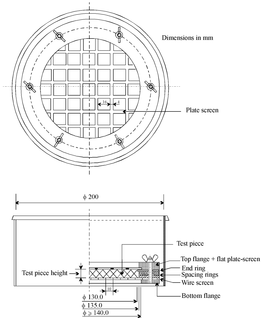
FIGURE D.1 Envelope clamping device
