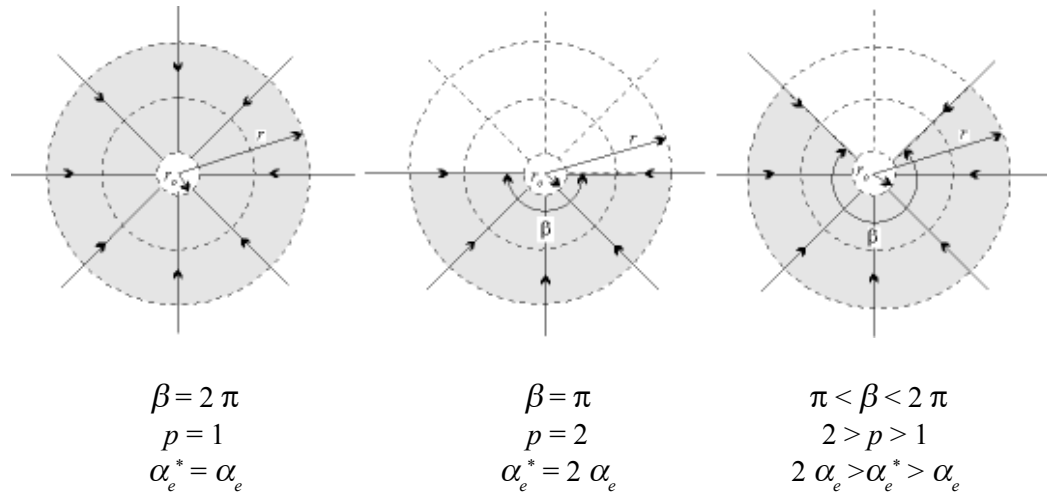
FIGURE 29 Influence of a partly radial flow pattern on the entrance resistance of real drains
