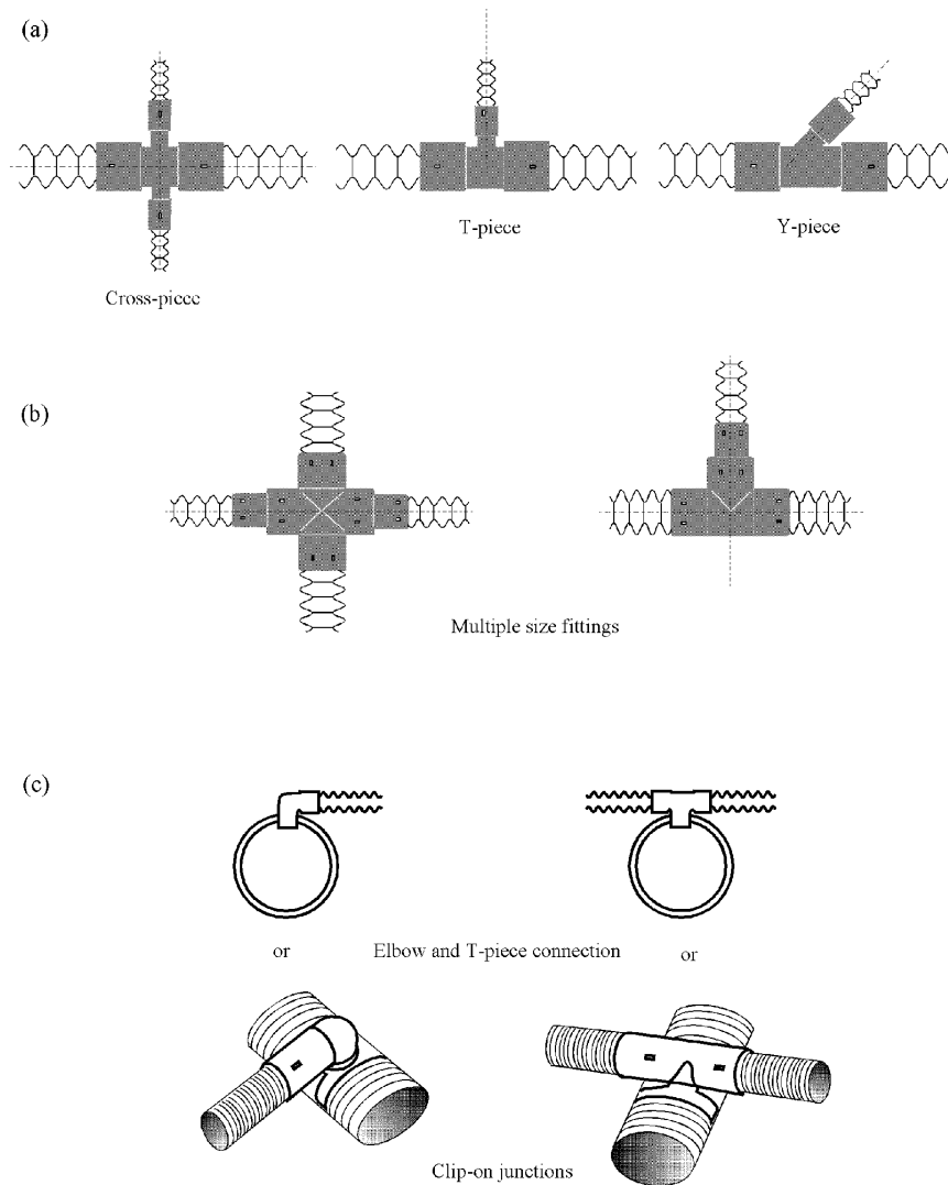
FIGURE 4 Pipe fittings
