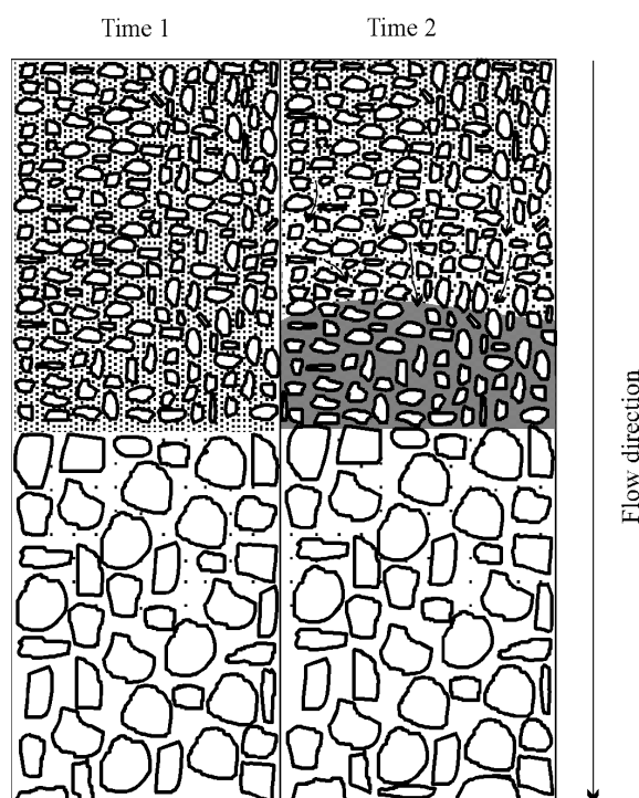
FIGURE 35 Filter cake
