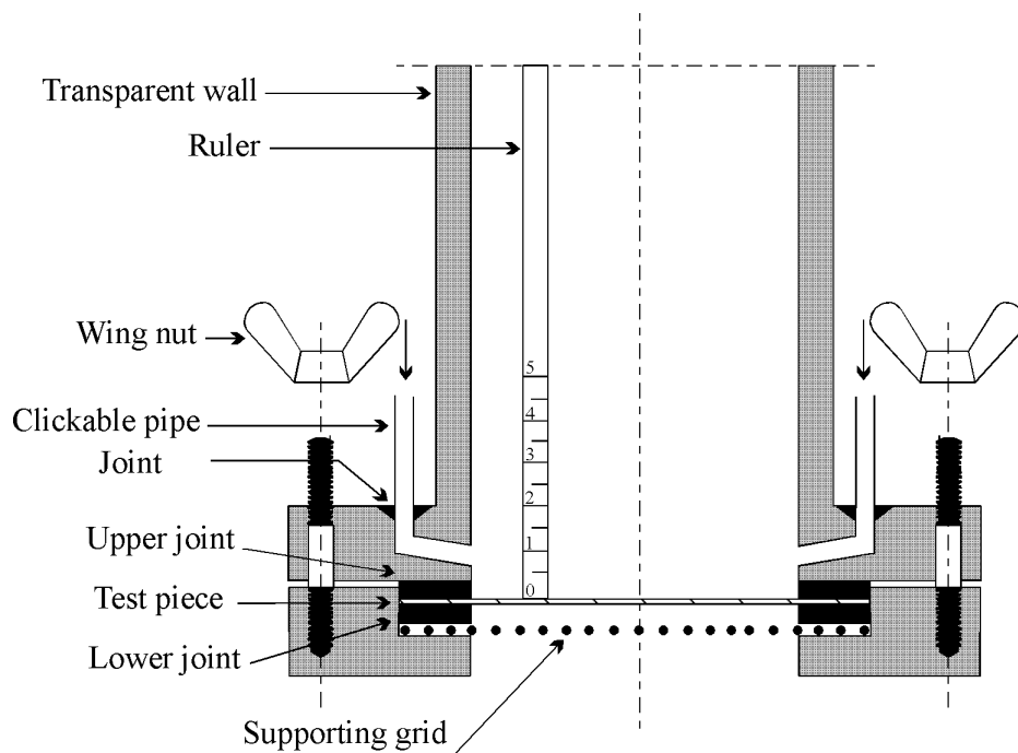
FIGURE A.4b Base of the measuring cylinder
