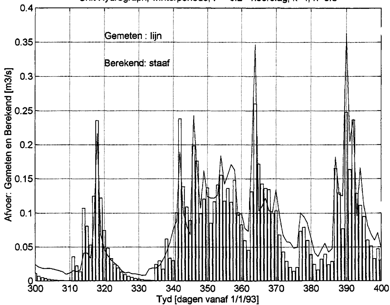
Unit Hydrograph, winterperiode, P = 0.2 * neerslag, k=4 , n=0.3
