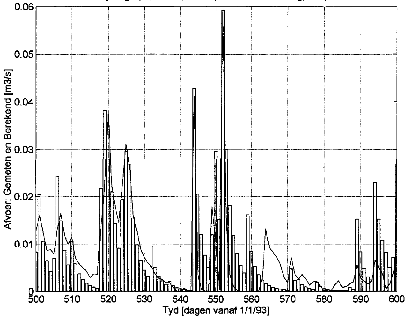
Unit Hydrograph, zomerperiode, P = 0.04 * neerslag, k=4, n=0.3
