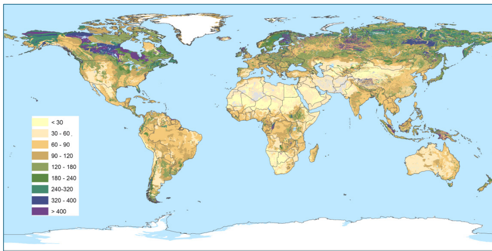
Figure 2. Soil organic carbon content to 1m depth (Mg C ha -1 )
