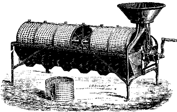
Fig. 105. Pernollet's sorteermachine; agent G. Stout te Tiel.
