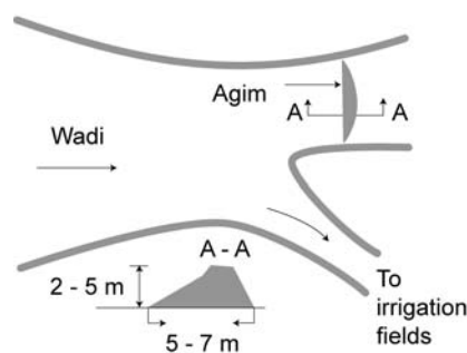
Figure 3.1 Weir type low earthen bund
