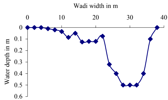
Figure 1.2 The Wadi Laba bed shape at the end of one hour of the flow duration
