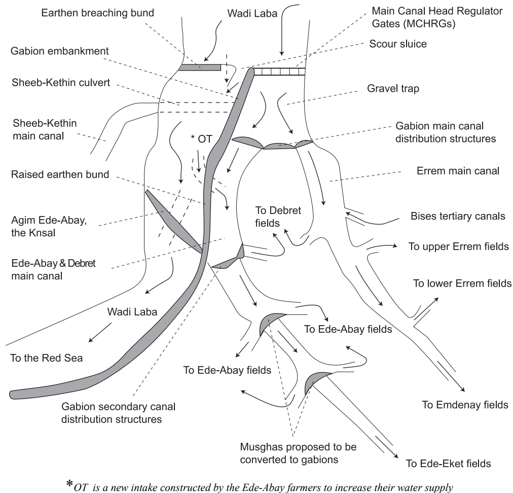
Figure 4.9 The layout of the Wadi Laba modern spate irrigation system after water management reforms (Mehari, et al., 2005c)
