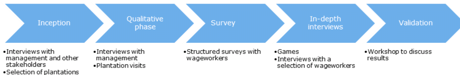
Figure 2.1 Overview methodology
