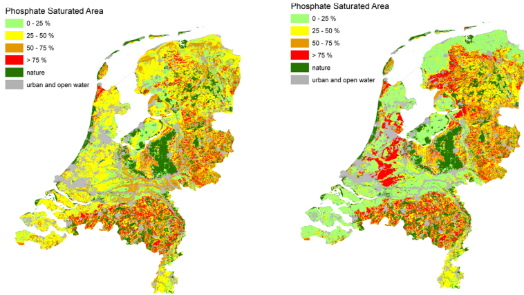
Figure 5. Percentage of the area classified as phosphate-saturated soil for agricultural soil use: left-hand map, based on PSD_{crit} of 25%; right-hand map, based on the PSD_{crit} specific to the soil type (see Table 2).
