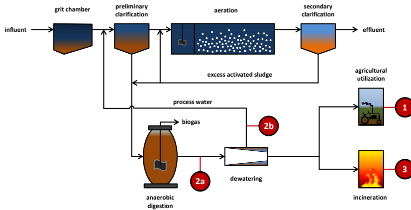
Figure 2. Hotspots for phosphorus (P) recovery from the wastewater stream (in centralized sanitation systems) Source: (Kabbe, 2013) Legend: 1 – direct sludge application in agriculture; 2a – P recovery from aqueous sludge phase prior to dewatering; 2b – P recovery from sludge liquor after dewatering; 3 – P recovery from mono-incineration ash.
