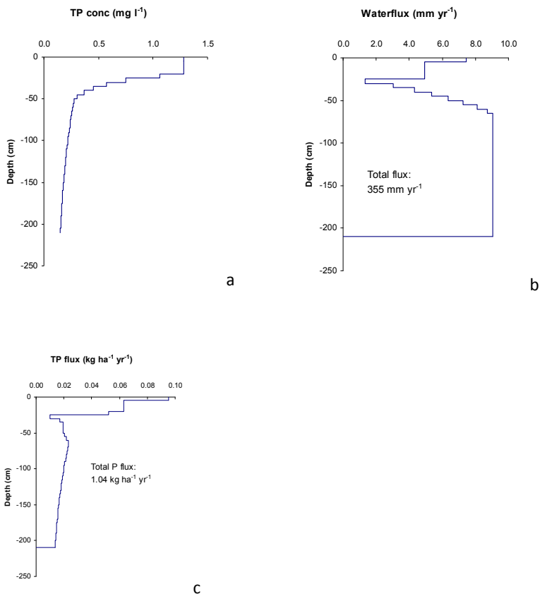
Figure 2. Example of the distribution of the (a) total P concentrations (mg l -1 ), (b) annual horizontal water flux ( J ; mm yr -1 ) and (c) total P flux (kg ha -1 yr -1 ) per 0.05 m layer.
