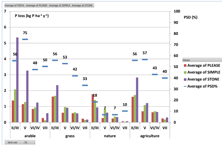
Figure 1. The measured average PSD, and estimates of the average annual P losses according to the PLEASE and SIMPLE approaches and the STONE dynamic model.
