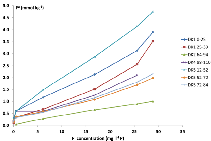
Figure 4. Additional amount of P bound ( F^3 ) after 56 days as a function of the final P concentration.
