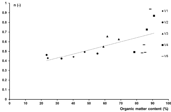
Figure 6. The relation between the exponent of the modified Freundlich equation ( n -value; Table 3) and the organic matter content.
