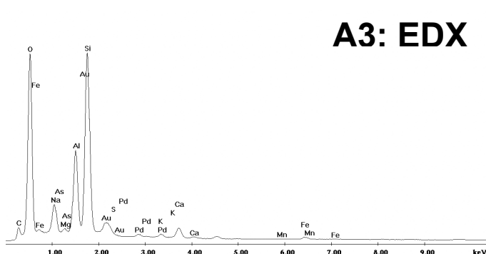
Figure 3-5 Left : Pre-testing SEM image of a grain (mother material cannot be identified due to weathering layer) completely covered with clay particles as shown by close up (A2) and EDX (A3). Right : Post-testing SEM image of K-feldspar grain from 60°C sediment partially covered with gibbsite and kaolinite fragments and EDX scan. Both images are from sediment B.
