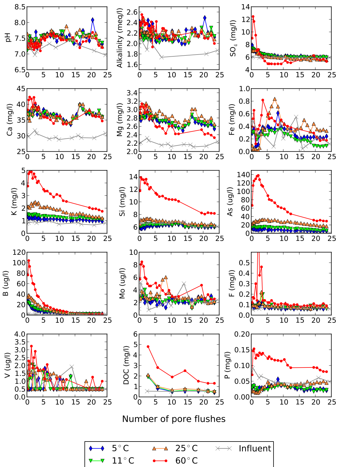
Figure 3-1 A selection of effluent graphs for main cations and anions, trace elements, and nutrients for sediment C. Results for the 60°C column between pore flushes 13 and 19 are not shown because of sampling errors.
