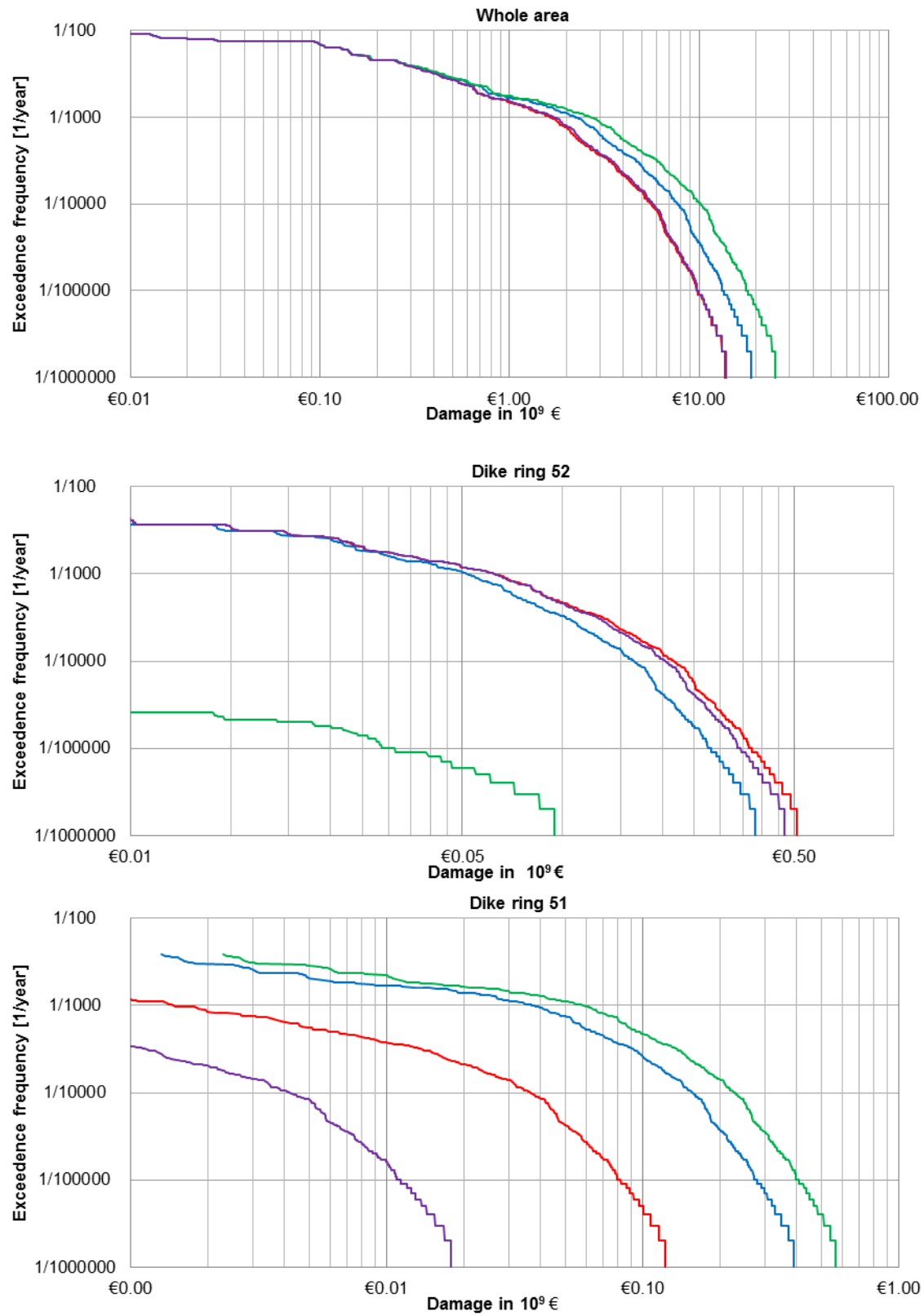
Figure 7 Results for economic damage for cases with breaches (red), without polder breaches (blue), no shortcutting (green) and no cascade effect (purple).
