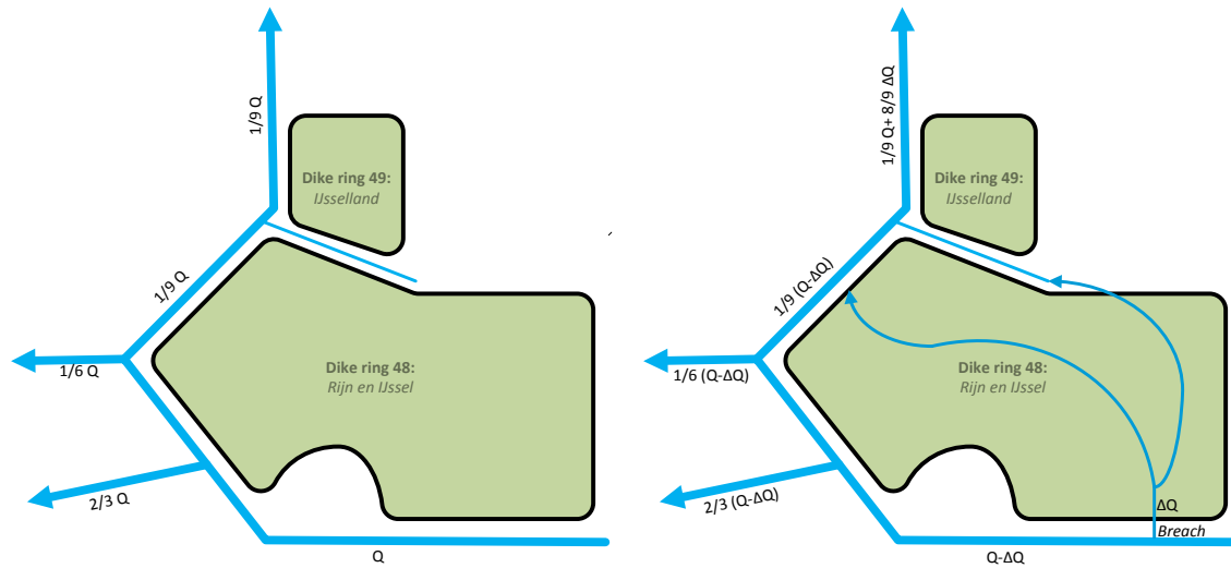
Figure 1: Change in discharge distribution due to shortcutting at the Bovenrijn/IJssel area, the Netherlands. Left is the given situation, right is the situation including shortcutting (time effects are ignored)
