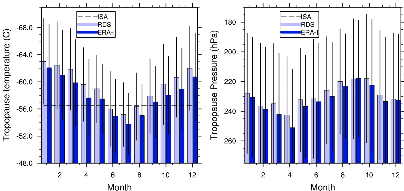
Figure 9. Climatology of average tropopause temperature (left) and pressure level (right) per month with standard deviation from De Bilt (left bar) and ERA-Interim (right bar). ICAO standard atmosphere values are presented in the horizontal broken lines.
