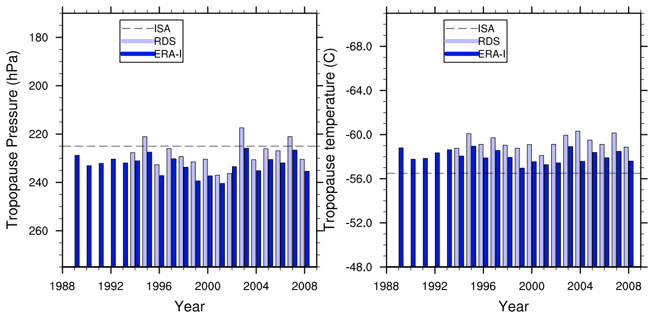
Figure 10. Average and standard deviation of tropopause pressure level (left) and temperature (right) per year in De Bilt 1994-2008 and ERA-Interim 1989-2008 for Netherlands-central.
