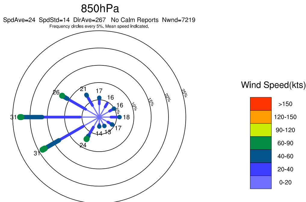
Figure 4. Example of a climatological wind rose.
