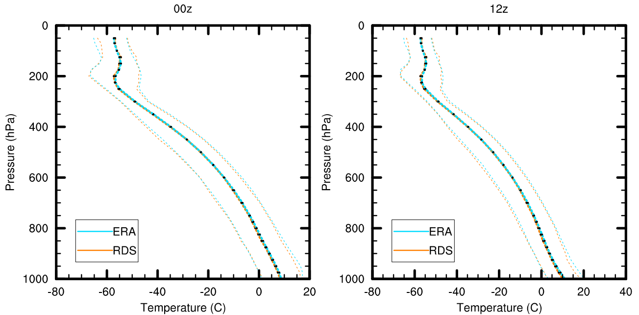
Figures 3. Example of profile-comparison of the soundings (RDS) and ERA-Interim from location De Bilt with average, 5 and 95 percentile of the parameter temperature in spring (months MAM) 00 and 12 UTC.
