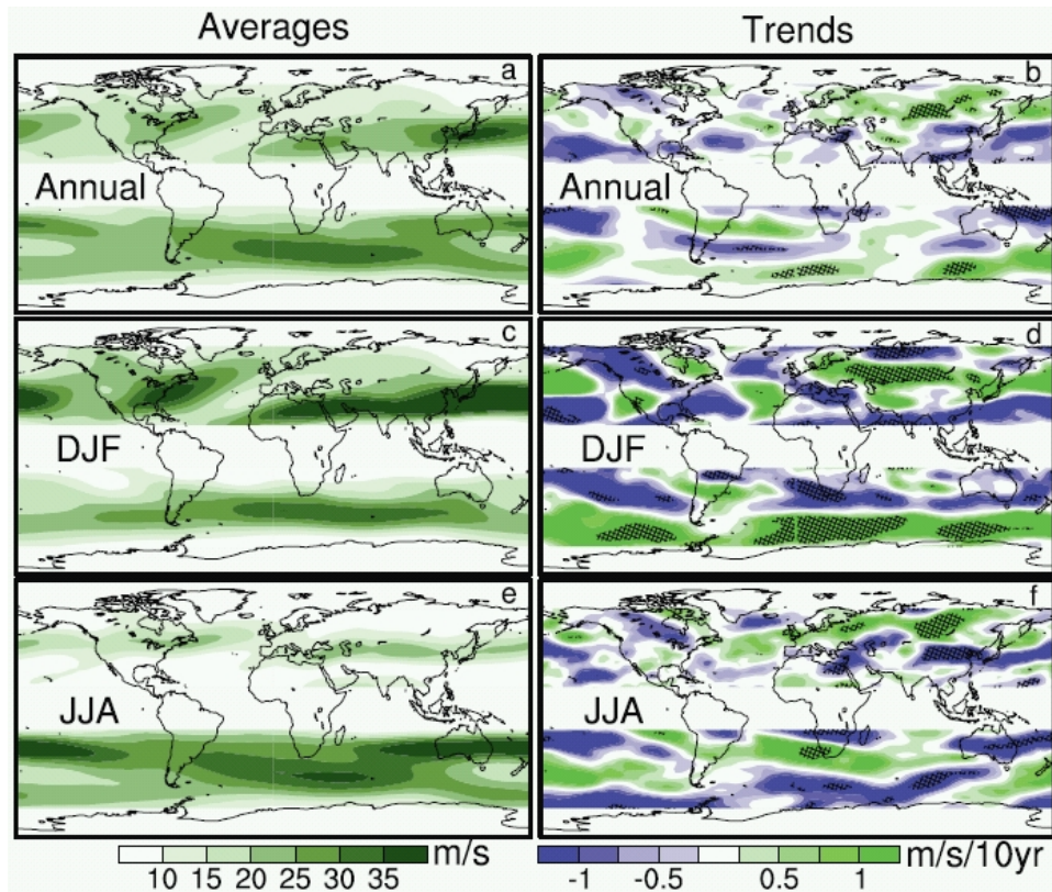
Figure 12. Jet stream wind speed from the ERA-40 reanalyses in 1979–2001: (a, c, e) annual, winter (DJF), and summer (JJA) averages (m/s); (b, d, f) linear regression trends (m/s/decade), hatched where statistically significant ( P -value < 0.15 ), taking auto-correlation into account.
