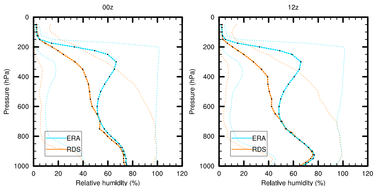
Figure 6. Example of profile-comparison of the soundings (RDS) and ERA-Interim from location De Bilt.
