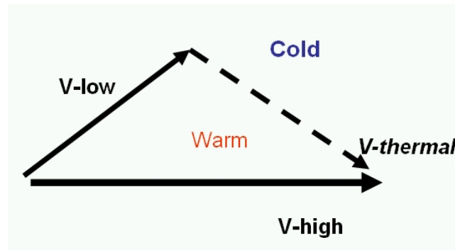
Figure 5. The thermal wind is the difference vector of the geostrophic winds in a layer of air, representing the temperature distribution (thickness) in that layer. In warm advection the geostrophic wind veers with height in the Northern Hemisphere.
