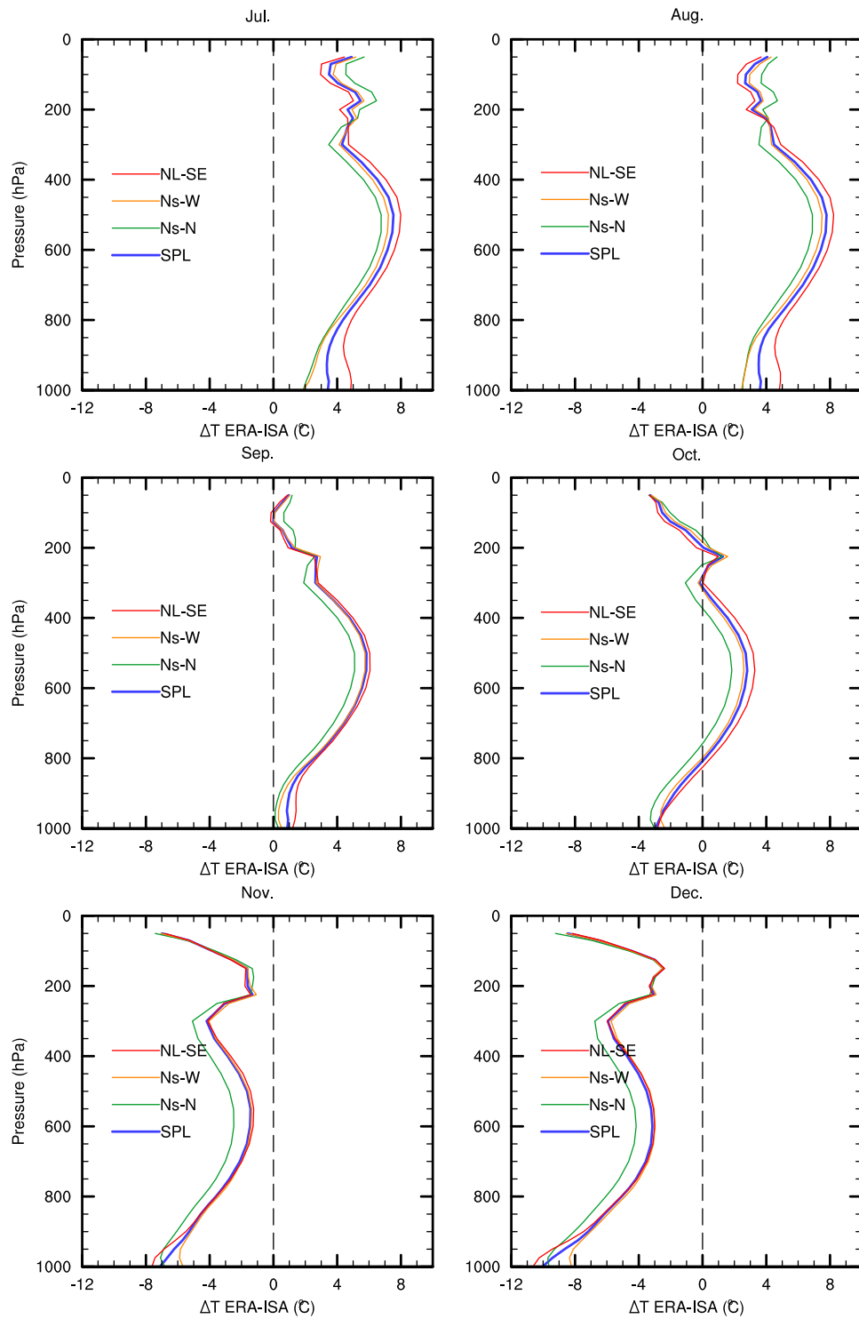
Figure 8. Deviation of temperature per month from ICAO Standard Atmosphere for requested locations.
