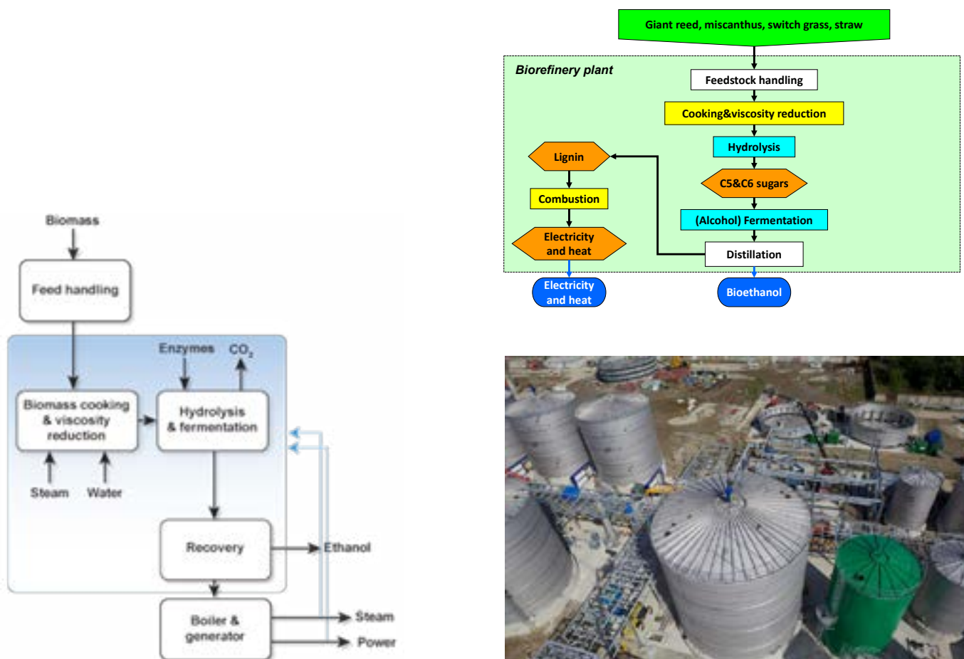
Figure 27. Demo Plant Crescentino, Italy [Beta Renewables]
