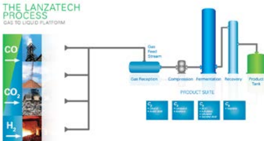
Figure 39. Pilot Plant Set-up [Lanzatech]
