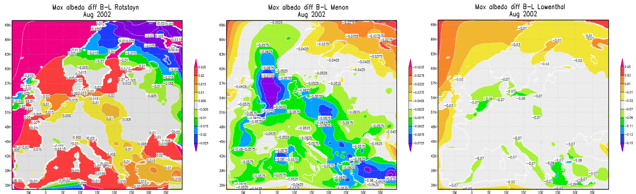
Figure 3.3 – Maximum possible difference in albedo: monthly average for August 2002. Different colorbars are used to show the complete range of variation for each comparison.
