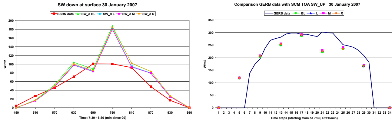
Figure 5.5 - Comparison with data of the radiation output.
