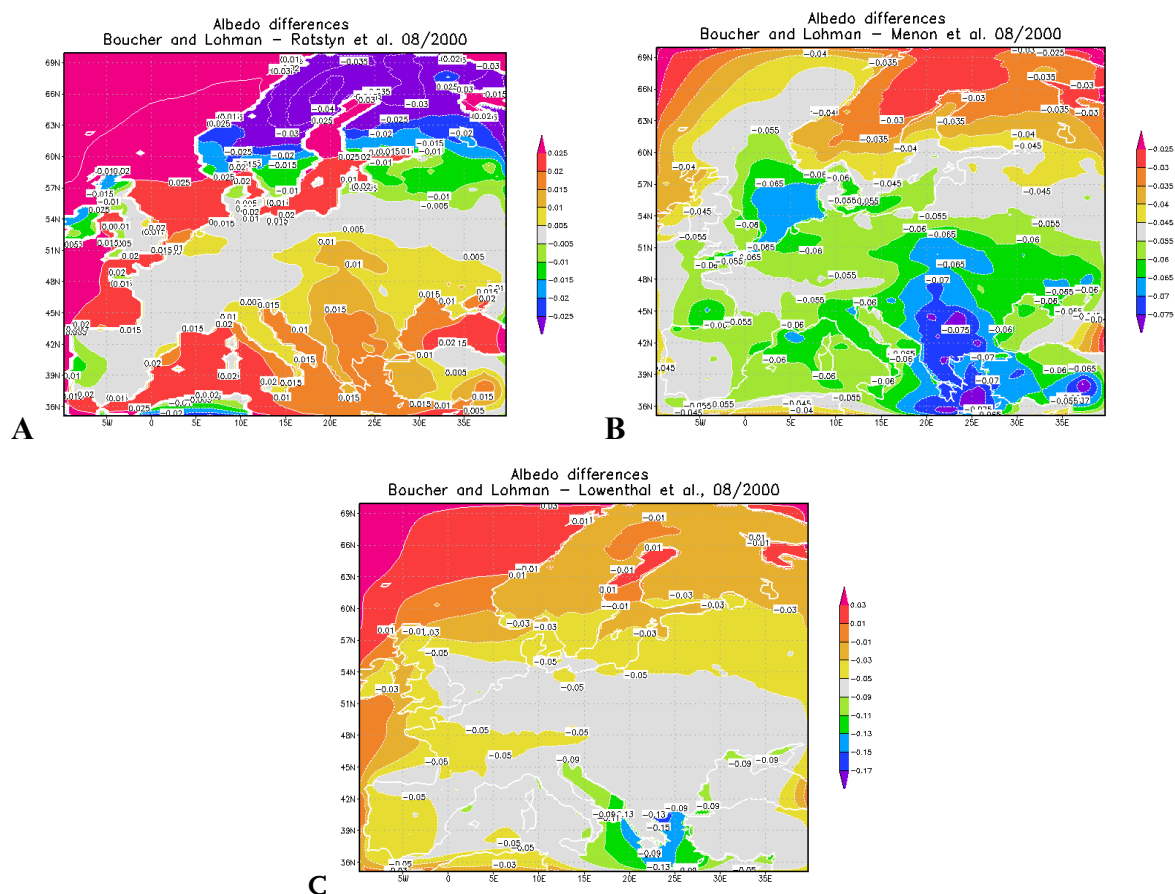
Figure 4.1 - Maximum possible difference in albedo, plotted on the LOTOS domain between the formulation proposed by Boucher and Lohmann, (1995) and the one by Rotstayn (1999) [panel A]; between Boucher and Lohmann, (1995) and Menon et al. (2002) [panel B]; between Boucher and Lohmann, (1995) and Lowenthal et al. (2004) [panel C], based on aerosol data for August 2000.
