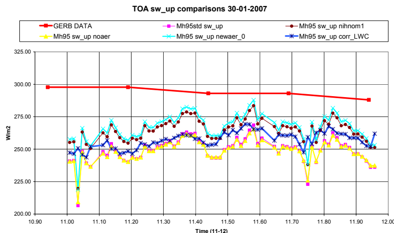
Figure 5.16 - SW going up at TOA: Comparison of model output and data for different numerical experiments
