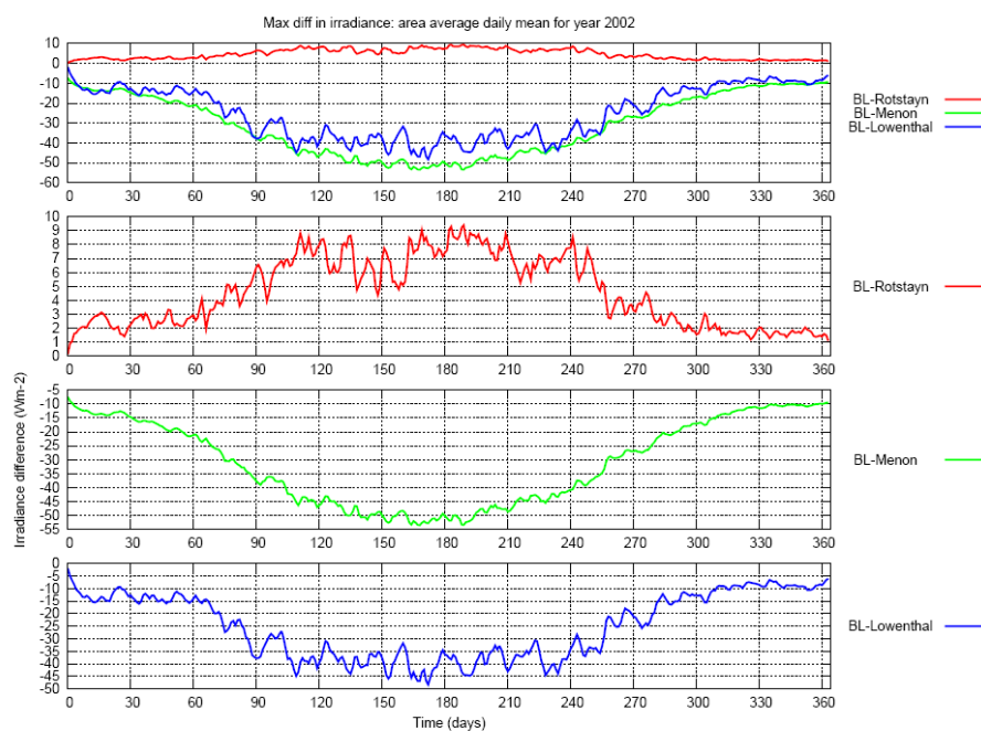
Figure 4.2 – Maximum differences in irradiance for the whole year 2002: area average.
