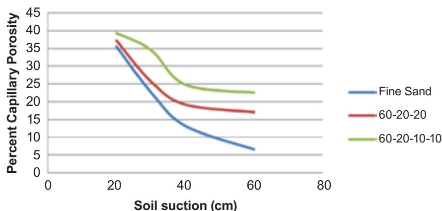
Figure 1 Water-release characteristics of three mixes for sand-channel drains
