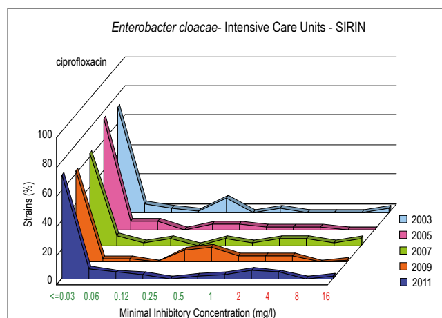
Figure 4.4.2.1.12. MIC distributions of ciprofloxacin for Enterobacter cloacae (N=756) from Intensive Care Units.
