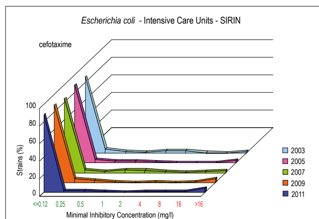
Figure 4.4.2.1.03. MIC distributions of cefotaxime for Escherichia coli (N=3042) from Intensive Care Units
