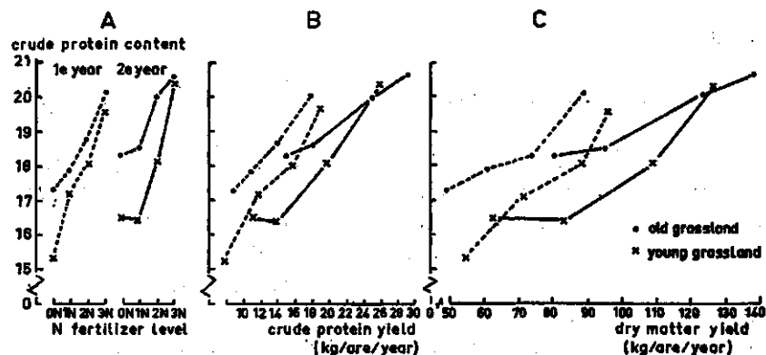
Fig. 4. Relation between crude protein content in the dry matter and nitrogen application (A), crude protein yield (B) and dry matter yield (C). Yield in kg/100 m 2 per year. Experiment E1.
