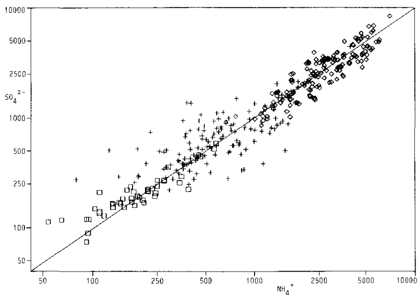
Figure 30. Ionic equivalent concentrations of \text{NH}_4 and \text{SO}_4 in precipitation (squares), throughfall (crosses) and stemflow (diamonds) in 1982 and 1983 ( \text{mmol/m}^3 , logarithmic scale). The line indicates equal concentrations of \text{NH}_4 and \text{SO}_4 .
