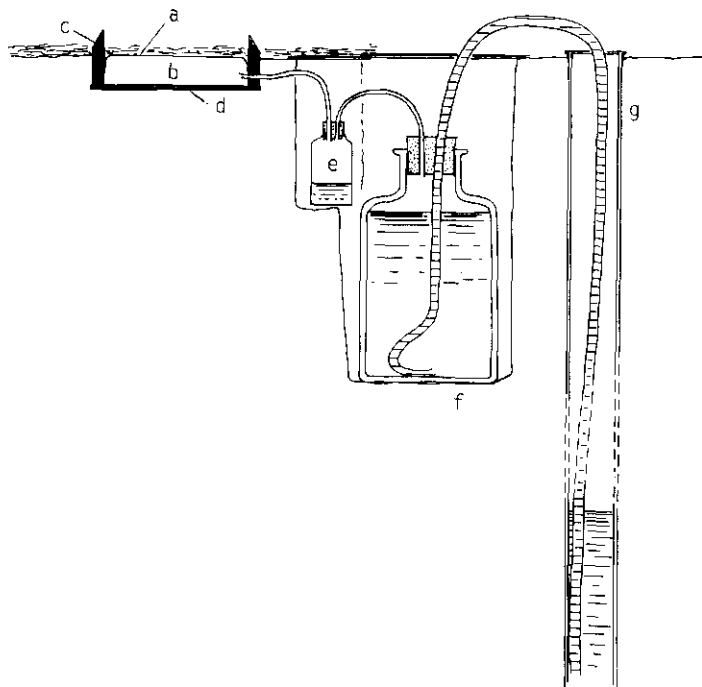
Figure 21. Cross section diagram of the porous plate and the hanging drop arrangement to collect soil solutions at the bottom of the forest floor. For explanation see text.
