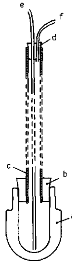
Figure 20. Cross section diagram of porous ceramic cups used to collect soil solutions in the mineral soil (not to scale). For explanation see text.
