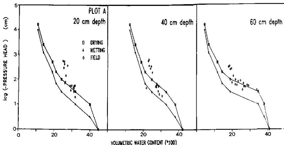
Figure 22. Comparison of water retentivity curves ( h(\theta) ), for plot A at 20, 40 and 60 cm depth, obtained by equilibration of 100 cm 3 undisturbed soil cores in the laboratory and obtained in the field from simultaneous measurements of volumetric water content (gamma attenuation method) and pressure head (tensiometry).
