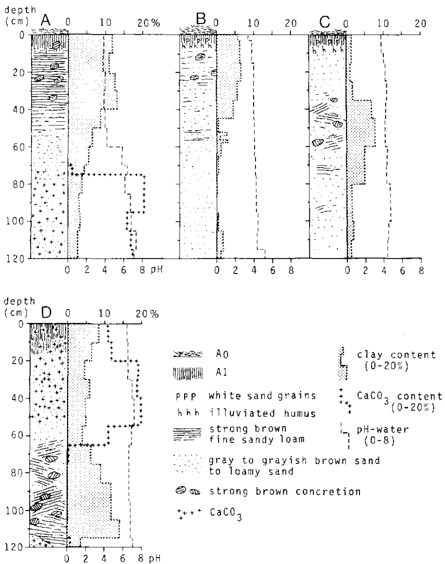
Figure 5. Some morphological and chemical characteristics of the soils used in this study (From: Van Breemen and Jordens, 1983).
