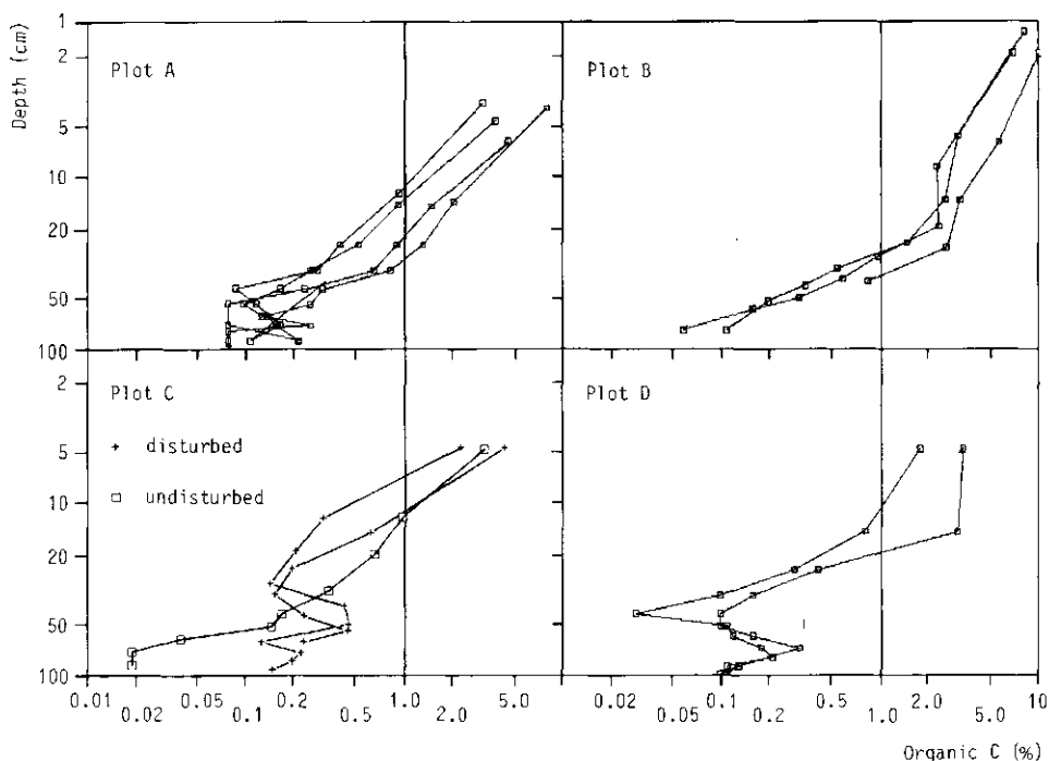
Figure 8. Organic carbon contents of the fine earth against depth for the mineral soil in plots A, B, C and D (double logarithmic scale).
