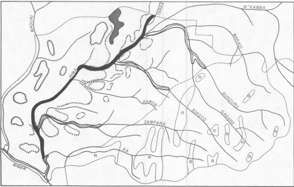
Stage 8. Slight incision and deposition by lacustrine-like rivers
