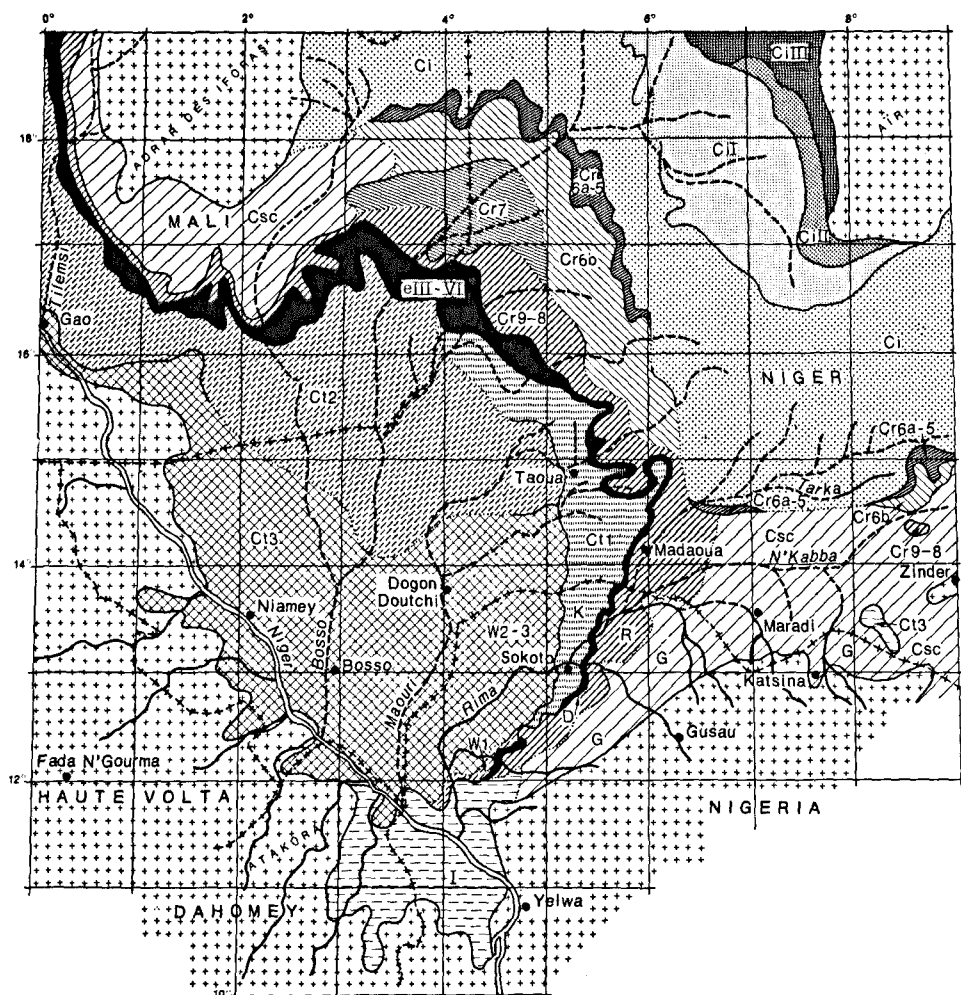
Fig. 4. Map of the pre-Quaternary geology of the Iullemeden-Middle Niger basin. Legend is Table 1.
