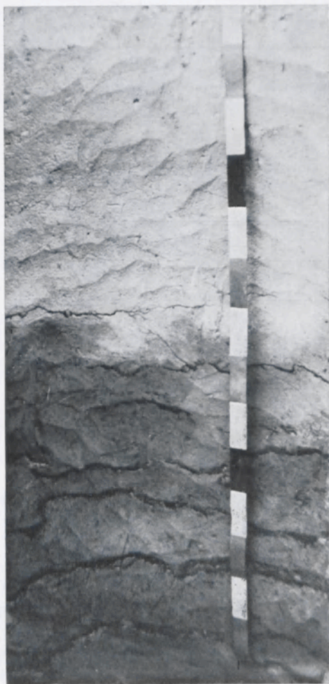
Fig. 13. Soil profile on the Rabah terrace. Yellowish Brown soil of Arid and Semi-Arid Tropical Regions/Haplargid, with banded clay accumulations in the subsoil ("fibers").
