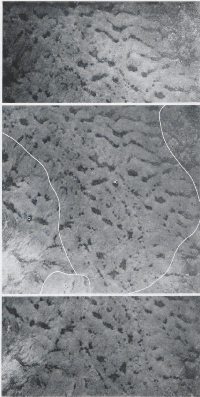
Fig. 9. The ripply vegetation pattern of pseudo dunes and gullies of the denudated Sangiwa coversands (A), a relic of low transversal dunes. For the symbols of the other mapping units cf. Appendix 1. (stereo-triplet E-W, scale 1 : 40,000, of an area 25 km south of Dange).
