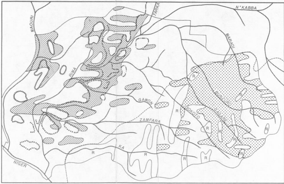
Stage 3. Coversand deposition
