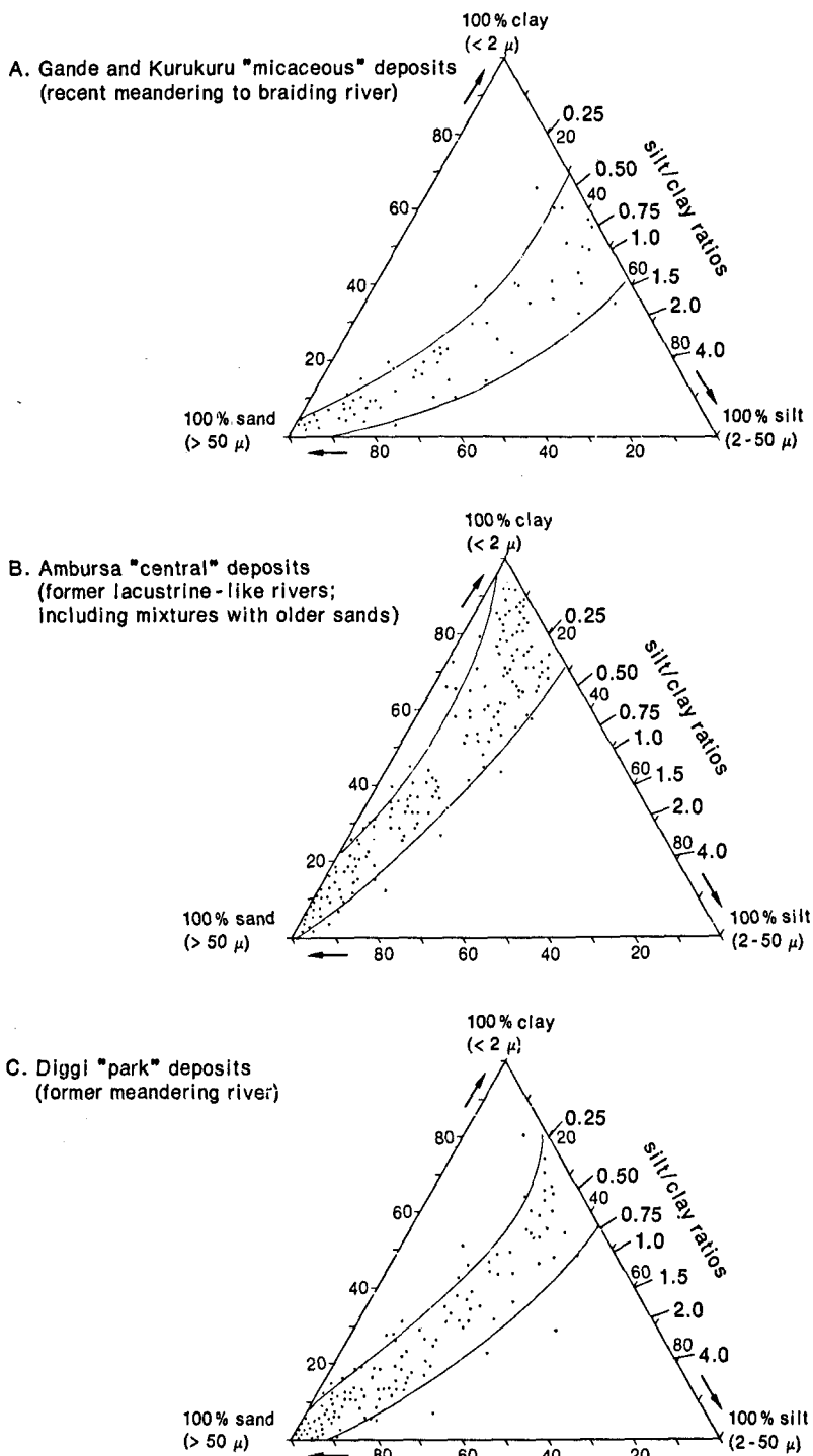
Fig. 14. (A to C) Triangular comparison of the grain-size distribution of some clayey aqueous deposits.
