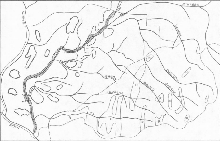
Stage 6. Incision and deposition by braiding rivers
