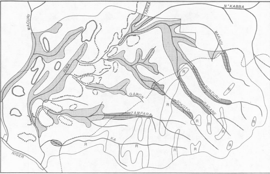
Stage 2. Sheetflood erosion and deposition
