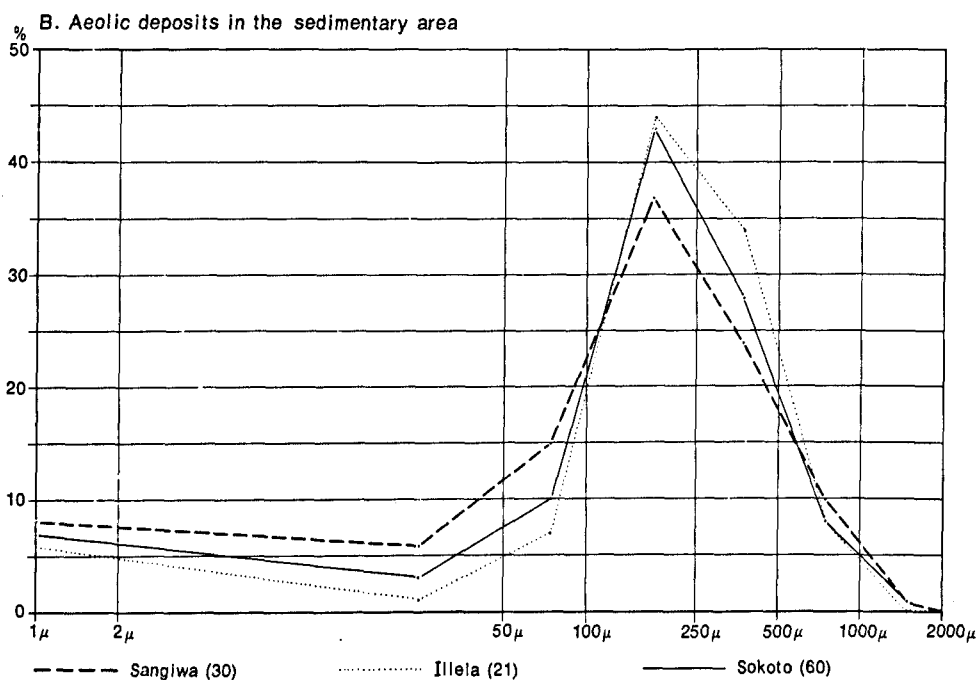
Fig. 12. (A to D) Graphical comparison of the grain-size distribution of various Quarternary deposits.
