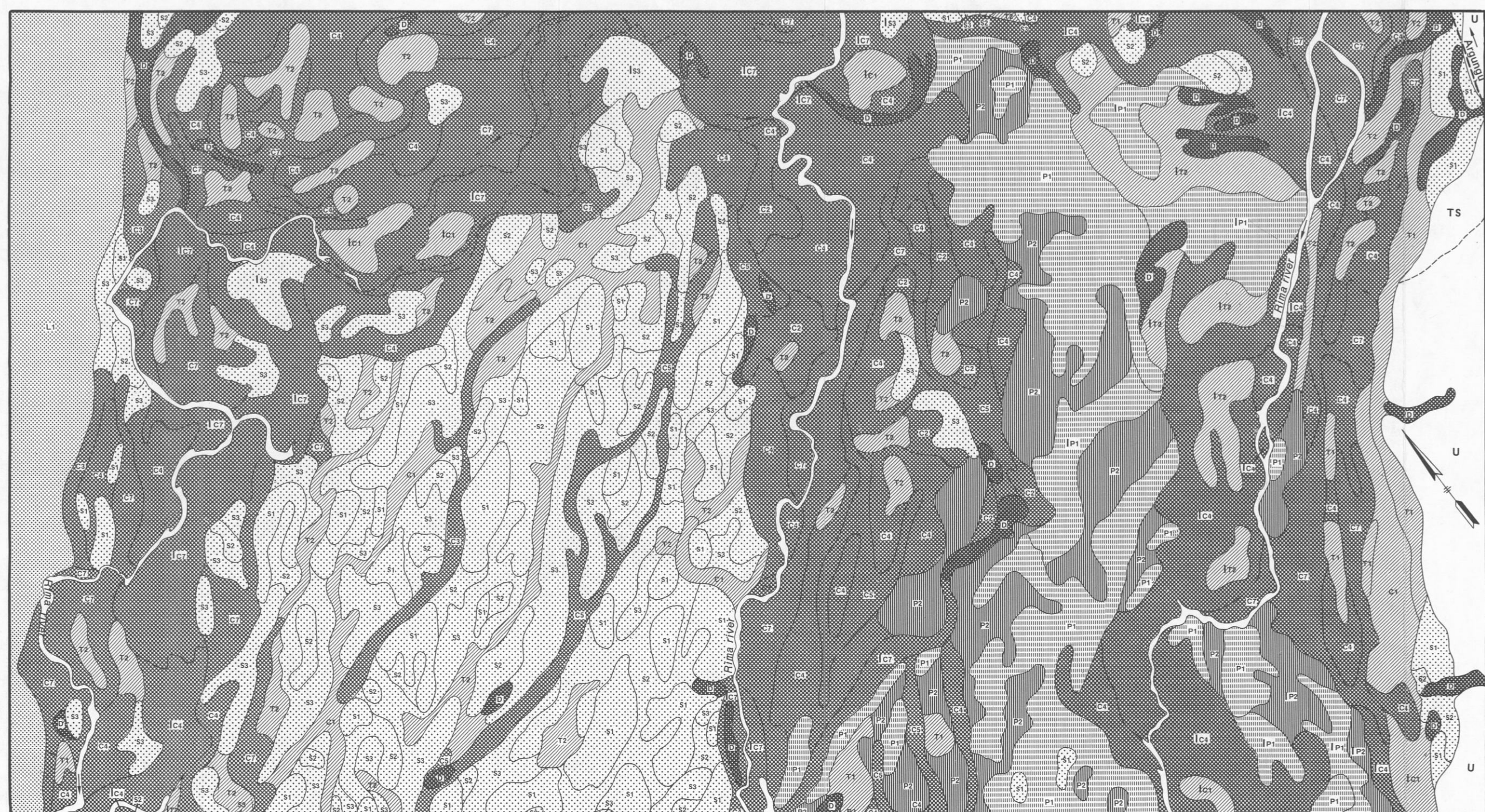
b) SOIL PATTERN IN A FLOODPLAIN AREA WITHOUT PRESENTDAY SEDIMENTATION (Rima river near Argungu)
