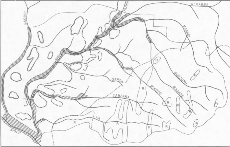
Stage 5. Incision and deposition by braiding to meandering rivers
