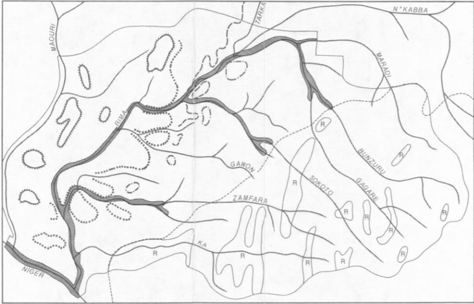
Stage 7. Incision and deposition by meandering rivers
