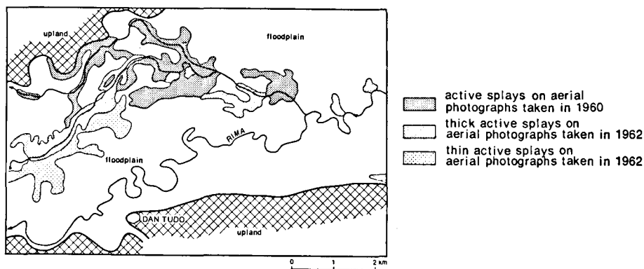
Fig. 23. Progress of Gande sedimentation in the Rima floodplain near Dan Tudu (between Kurukuru and Sabon Birni).
