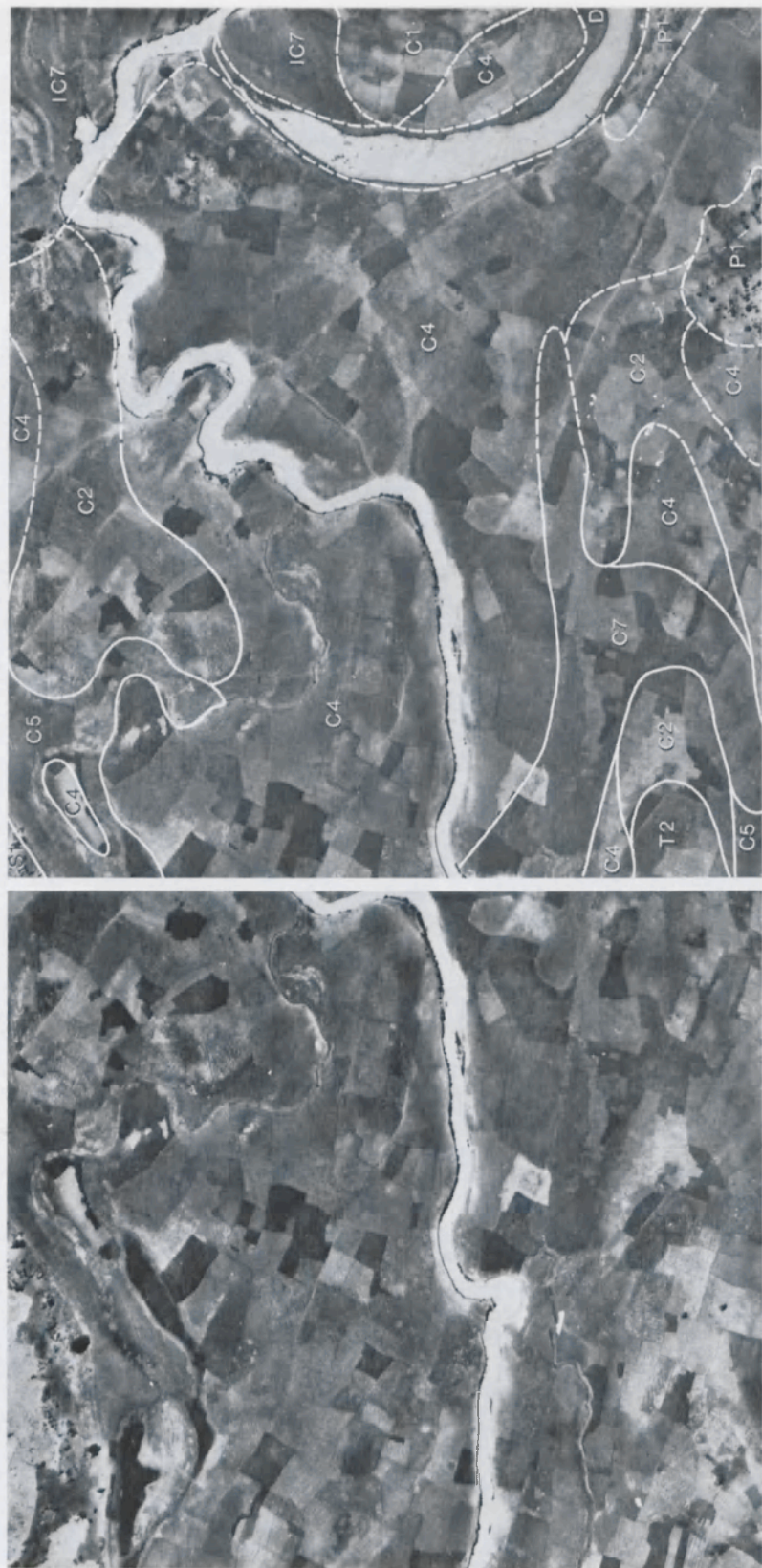
Fig. 17. The extensive level floodplain parts (C1 to C7), constituted by Ambursa deposits, of lacustrine origin. The present-day river channels, carrying sediment-poor water in these areas, cross the terrains without a banding of levees. For the other mapping symbols cf. Appendix 2. (stereo-pair NE-SW, scale approx. 1 : 10,000, of a floodplain part near Argungu, top-centre of Map b. of Appendix 2)
