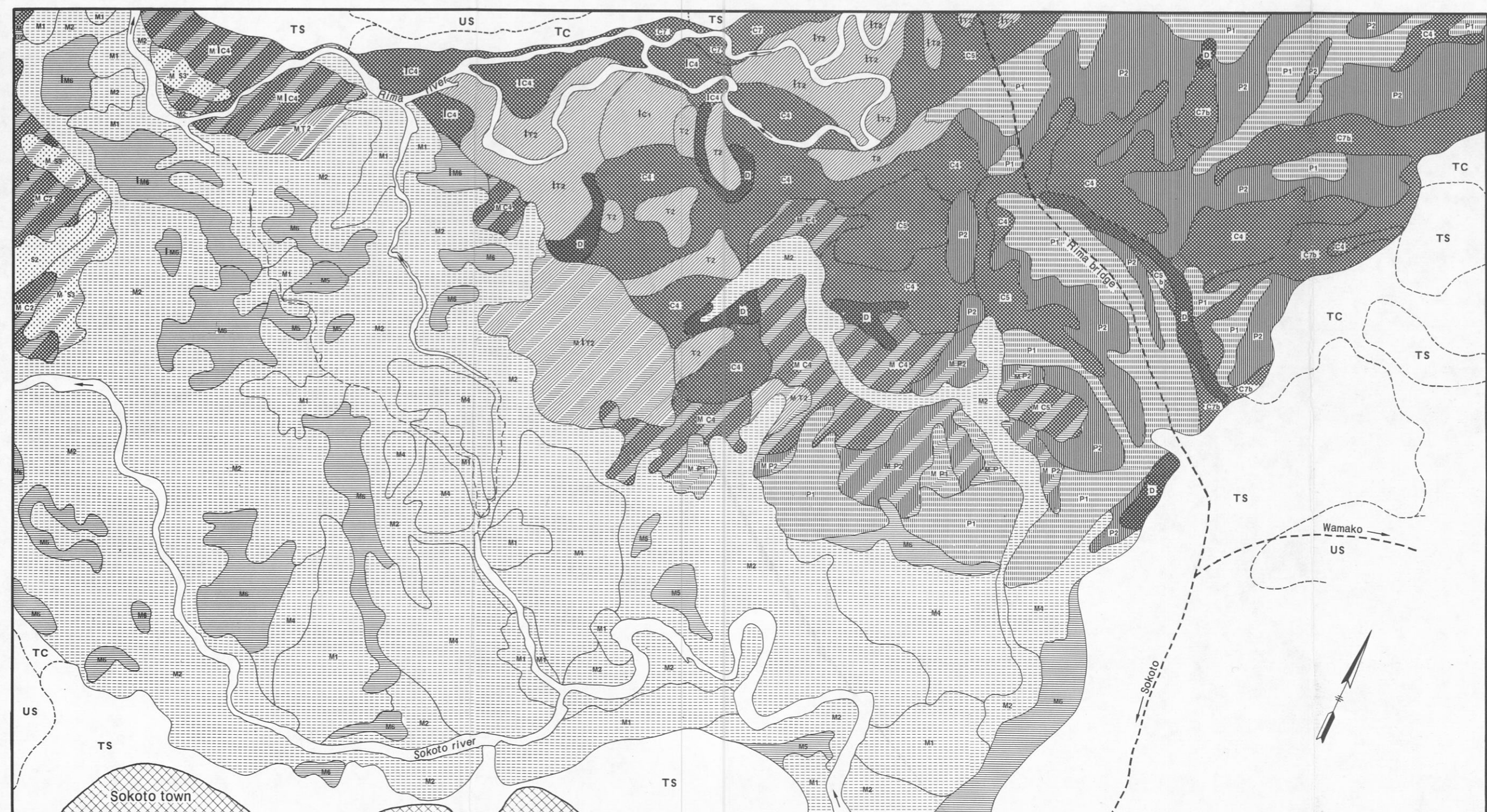
a) SOIL PATTERN IN A FLOODPLAIN AREA WITH PRESENTDAY SEDIMENTATION (confluence of the Sokoto and Rima rivers)
