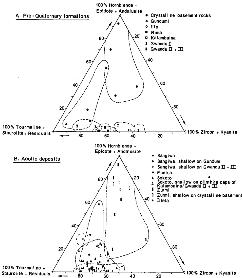
Fig. 24. (A to D) Triangular comparison of the heavy mineral composition of pre-Quaternary formations and Quaternary deposits.
