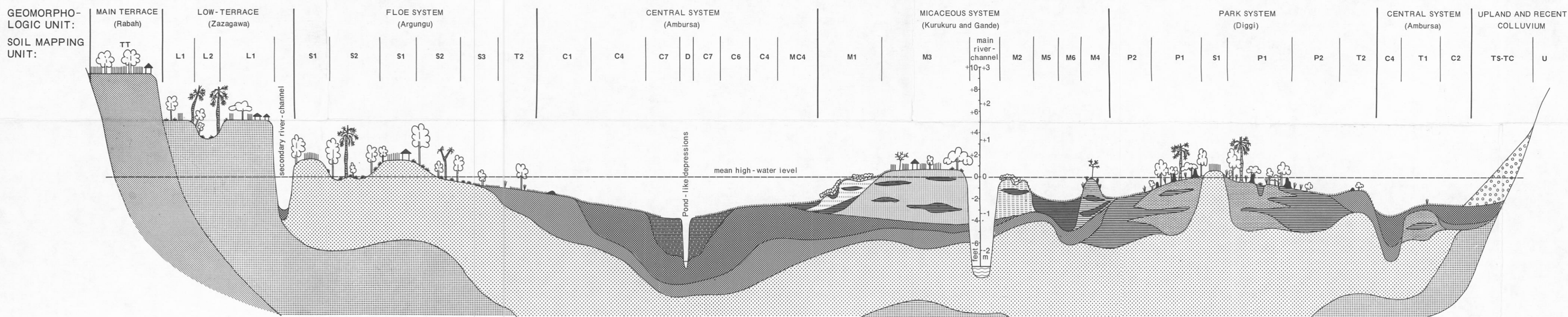
SCHMATIC CROSS-SECTION OF THE RIMA FLOODPLAIN (textural differentiation due to pedogenesis not indicated)
