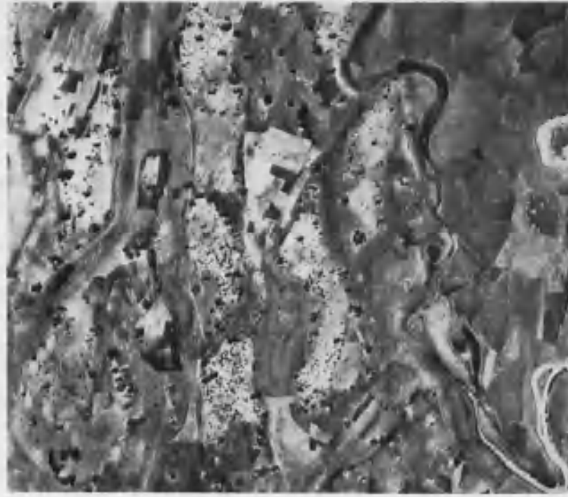
Fig. 15. The floe-like pattern of non-eroded parts (S1), shallowly eroded parts (S2), and low, flattened stretches (S3) of the Argungu deposits, of braiding river origin. For the other mapping symbols cf. Appendix 2, (stereo-pair NE-SW, scale approx. 1 : 10,000, of a floodplain part near Argungu, centre of Map h. of Appendix 2)
