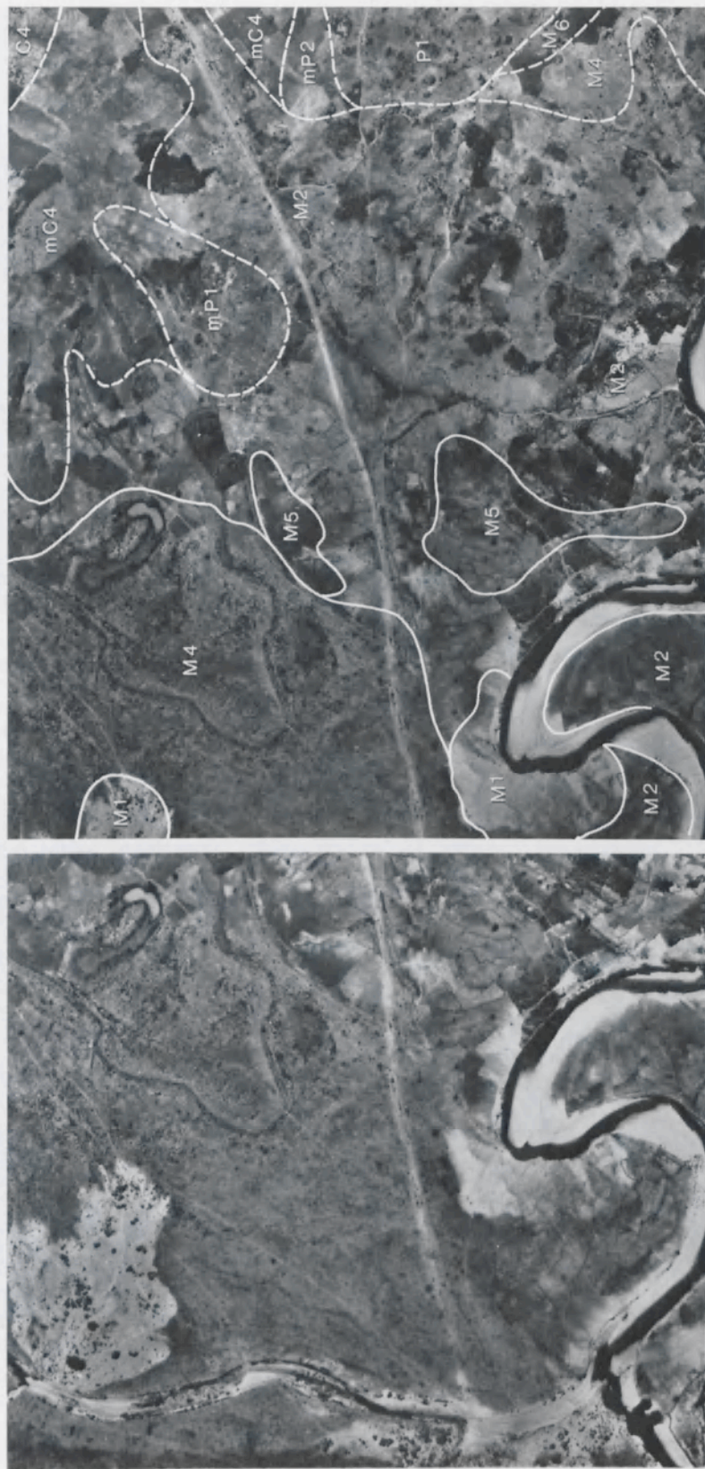
Fig. 18. The irregular meso-relief of the various units and phases (M1 to M6) of the Kurukuru-Gande micaceous deposits, the result of present-day meandering-river activity in stretches with sediment-rich water. For the other mapping units cf. Appendix 2. (stereo-pair N-S, scale approx. 1 : 10,000, of a floodplain part near Sokoto town, bottom-centre of Map a. of Appendix 2)
