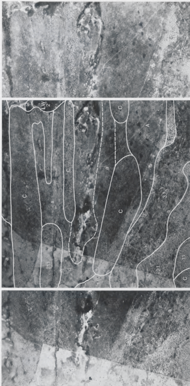
Fig. 10. The elongated pattern of the low longitudinal dunes of the Sokoto coversands (C). For the symbols of the other mapping units cf. Appendix 1. (stereo-triplet E-W, scale 1 : 40,000, of an area 25 km north of Lema)
