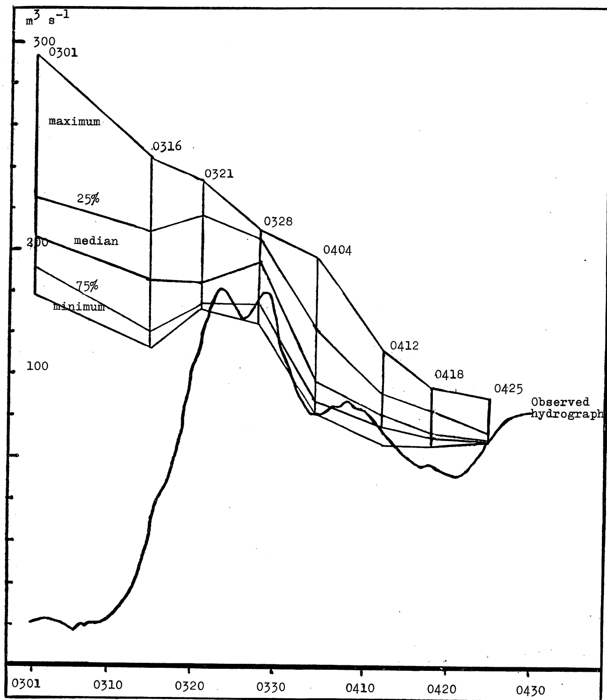
Figure 4 - Forecast of peak flows in Blankastrom based on 13 simulations
