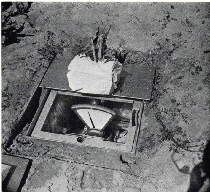
FOTO 12. Ingebouwde balans, geopend, zonder afdak tegen de zonnewarmte. PHOTO 12. Built-in balance, opened, without screen against insolation.
