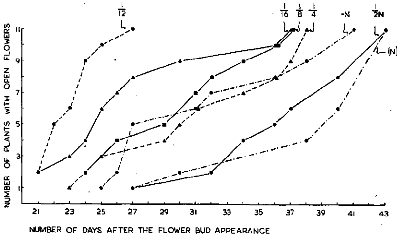
FIG. 3. Experiment VII: Effect of nitrogen on flower development of mustard in long day.
