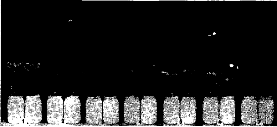
PHOTO 1. Experiment I, see p. 9: Mustard plants in water culture, showing the accelerating effect of nitrogen deficiency on flower development: 1. complete nutrient solution, 2. minus N, 3. -P, 4. -S, 5. -Mg, 6. -K, 7. -Ca.
