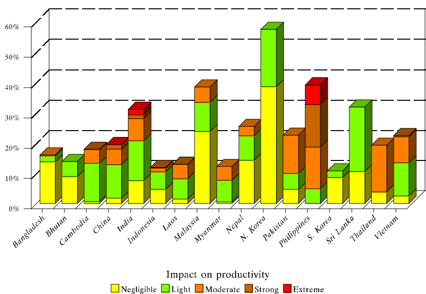
Fig 4 Relative distribution of water erosion (on-site effects) (as % of total land area per country)
