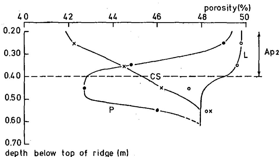
Fig. 11. Porosity after different treatments of a loamy sand soil.
