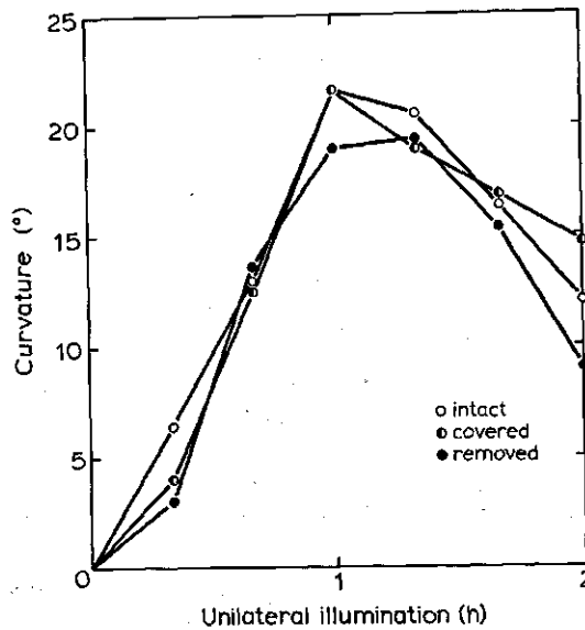
FIG. IV.1. Influence of covering (◐-◐) or removal (●-●) of cotyledons on hypocotyl curvature and their intact control (○-○). Average values of 10 seedlings.
