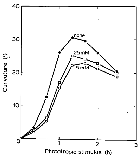
FIG. VII.8. Phototropic curvature of seedlings grown in white light treated daily with 1 ml 5mM (O—O) or 1 ml 25 mM (□—□) chlor-mequat on the pot soil; untreated controls: (●—●). Average values of 10 seedlings.
