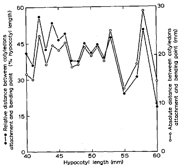
FIG. III.5. Relation between the length of the hypocotyl and the location of the bending point. Average values of samples of 6 to 9 seedlings.
