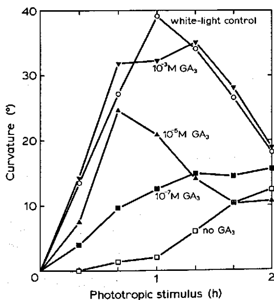
FIG. VII.7. The influence of 100 \mu l 10^{-3} M (▼-▼), 10^{-5} M (▲-▲), and 10^{-7} M (■-■) GA_3 on the phototropic curvature of seedlings pretreated with red light (□-□), and the phototropic curvature of seedlings grown in white light (○-○). Average values of 10 seedlings.
