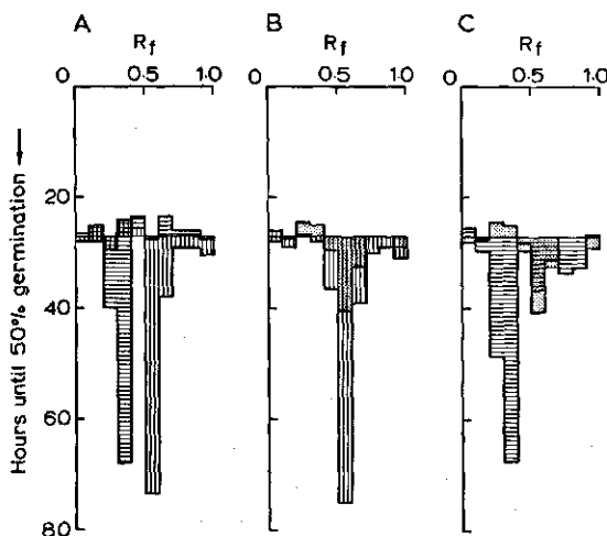
FIG. VII.2. The inhibiting zones in the cress seed germination assay of A: ABA (horizontal bars) and xanthoxin (vertical bars), B: plant extract (horizontal bars) and plant extract mixed with xanthoxin (vertical bars) and C: plant extract (horizontal bars) and plant extract mixed with ABA (vertical bars). Solvent system used: ethyl acetate:hexane = 3:1.
