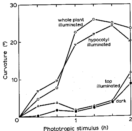
FIG. V.5. Phototropic response of etiolated seedlings after 18 h white light on the whole seedling (O—O), on the hypocotyl only (▽—▽), on the top only (Δ—Δ), or after continuous darkness (●—●). Average values of 10 seedlings.
