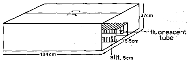
FIG. II.1. A schematic presentation of the experimental box, one side wall removed.
