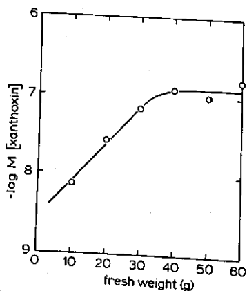
FIG. VII.5. Relation between the amount of fresh weight extracted and the amount of inhibitor obtained as determined in the cress seed germination assay.
