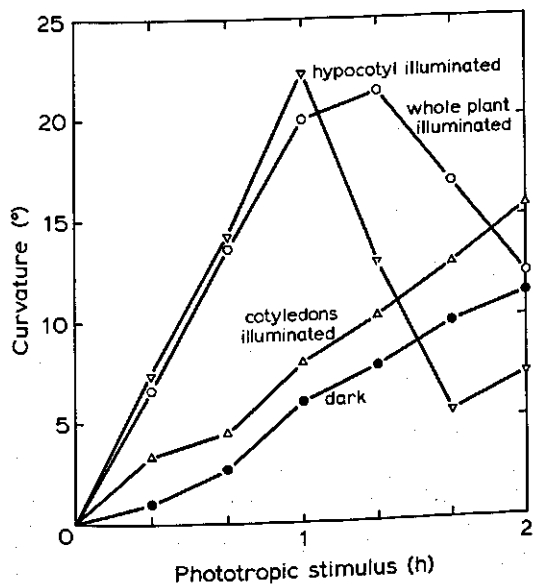
FIG. V.6. Phototropic response of green seedlings after 18 h white light on the whole seedling (O—O), on the hypocotyl only (▽—▽), on the cotyledons only (Δ—Δ) or after darkness (●—●). Average values of 10 seedlings.
