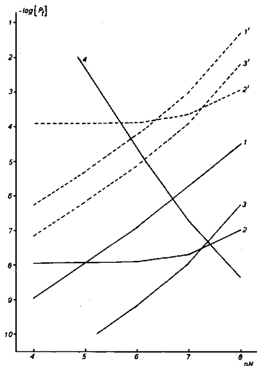
Fig. 3.6 Solubility diagram of different aluminum phosphates (1=variscite, 2=crandallite and 3=wavellite) in equilibrium with amorphous (solid line) and crystalline (broken line) \text{Al}(\text{OH})_3 . The solubility of hydroxyapatite (line 4) is based on a reference level of (\text{Ca}^{2+}) = 1.16 \text{ mmol/l} .
