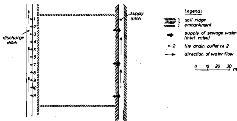
Fig. 3.1 Schematic plan of a single parcel of the sewage farm located near Tilburg.
