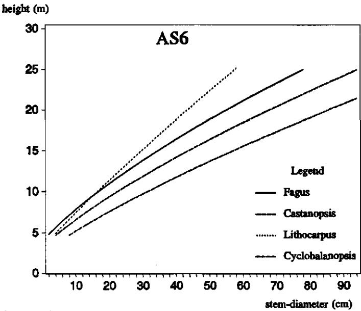
Figure 3.7 Example of the height / stem diameter regression curves for different species within one site (AS6): d = \alpha * h^b .
