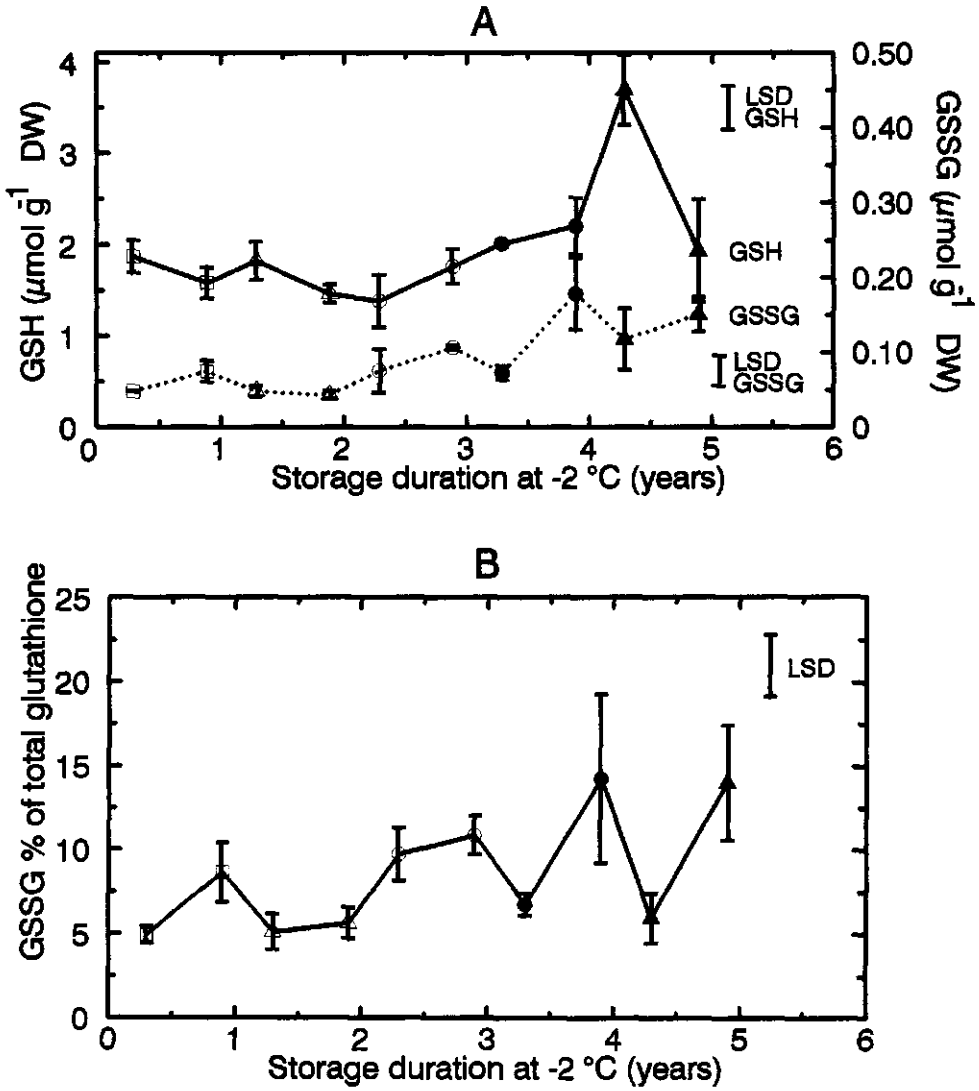
Figure 8.3 Effect of storage at -2\text{ }^{\circ}\text{C} in moist peat on content of reduced glutathione (GSH) and oxidized glutathione (GSSG) (A); and oxidation state of glutathione (B) in lily bulb scales of 'Enchantment' ( \square = harvest 1993, \Delta = harvest 1992, \circ = harvest 1991, \bullet = harvest 1990, \blacktriangle = harvest 1989). Data represent means \pm SD of three bulbs (20 to 60 scales each).
