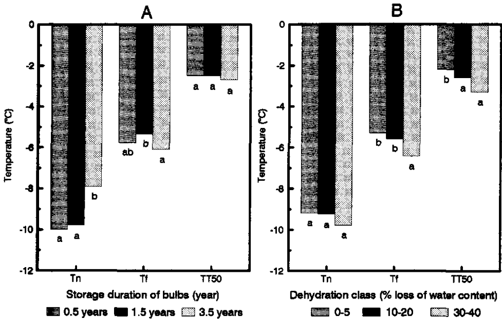
Figure 7.3 Nucleation temperature (Tn), maximum temperature during freezing (Tf), and melting temperature (TT50) of lily scales 'Enchantment' exposed to a temperature declining from 10 °C to -12 °C in about 30 minutes. (A): Scales were taken from bulbs stored previously for 0.5, 1.5 and 3.5 years at -2 °C; (B): Scales were air-dried and distributed into three classes of water content loss (all the three storage durations). Different minor characters indicate significant differences ( P \leq 0.05 ) between treatments. Nine to twelve scales were used per treatment.
