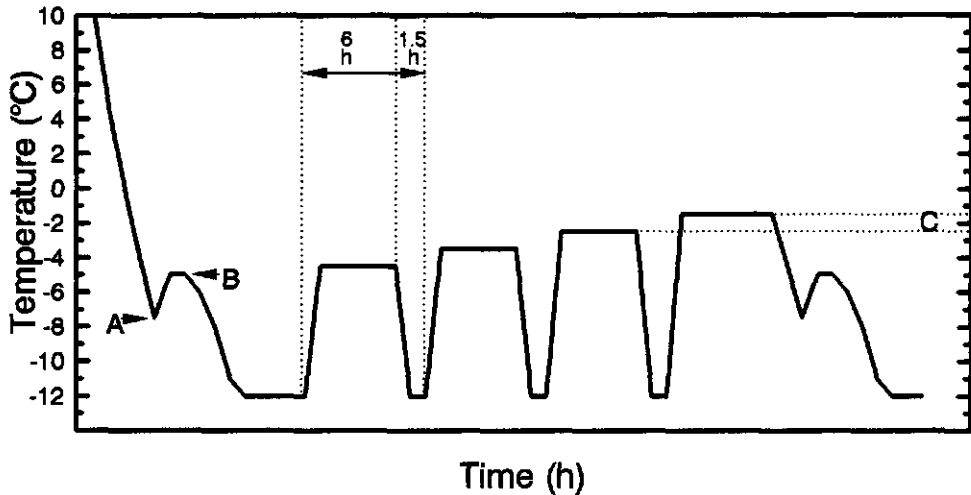
Figure 7.2 Determination of the nucleation temperature (A), the maximum temperature during freezing (B), and the melting temperature range (C) of lily scales. The temperature was regulated by a cooled incubator and was measured in the scales by a copper/constantan thermocouple. Further method description: see page 61.
