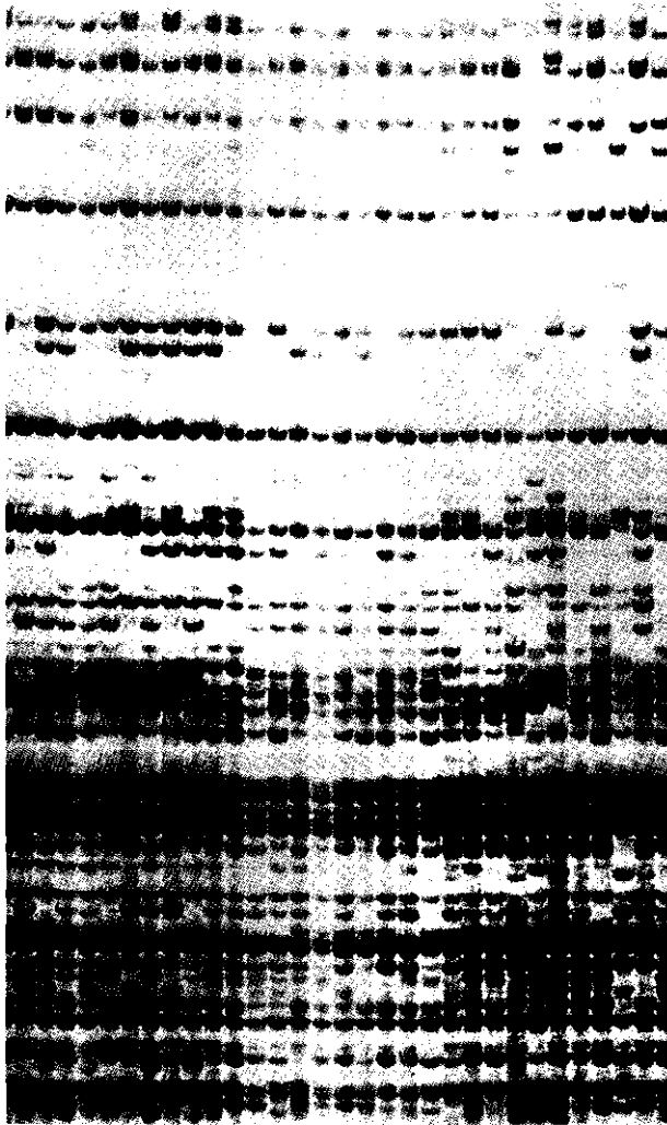
Figure 1.6 AFLP fingerprints.
