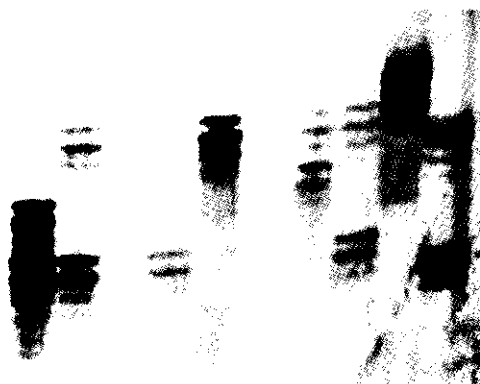
Figure 1.7 Microsatellite fingerprints
