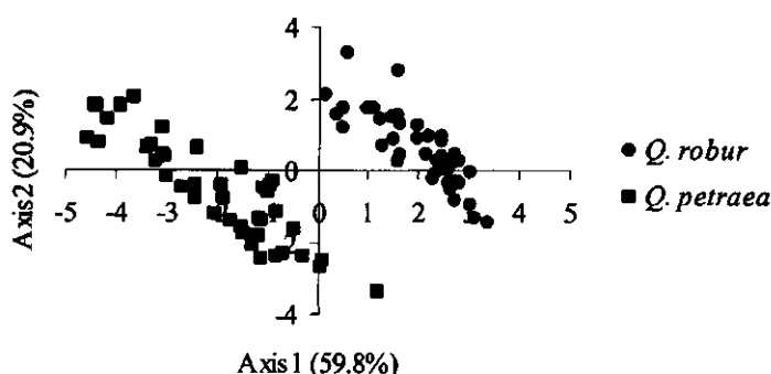
Figure 2.2 PCA
